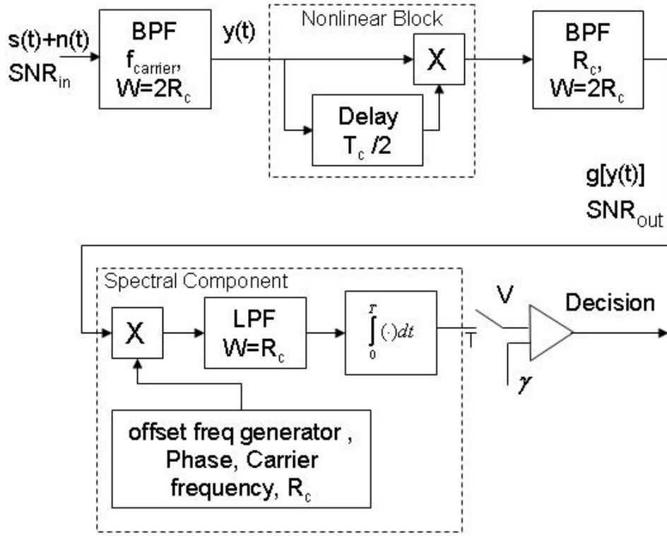
Figure 3 Block diagram of a CRD from [11].
