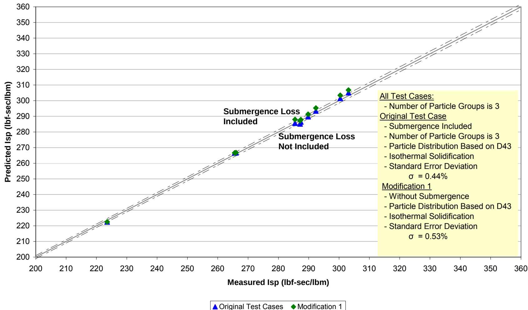
Measured Isp vs Predicted Isp ATA Test Cases Original & Modification #1 Test Cases
