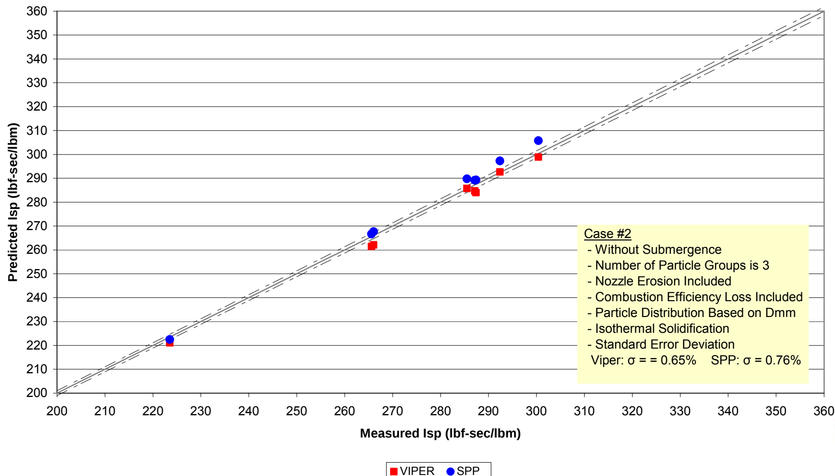
Measured Isp vs Predicted Isp Comparison Between SPP and VIPER Codes (Case #2)
