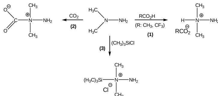
Figure 8: Proposed schemes for preparing four different UDMH adducts
