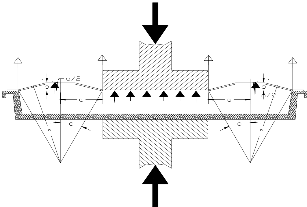
Figure 2: Force Diagram
