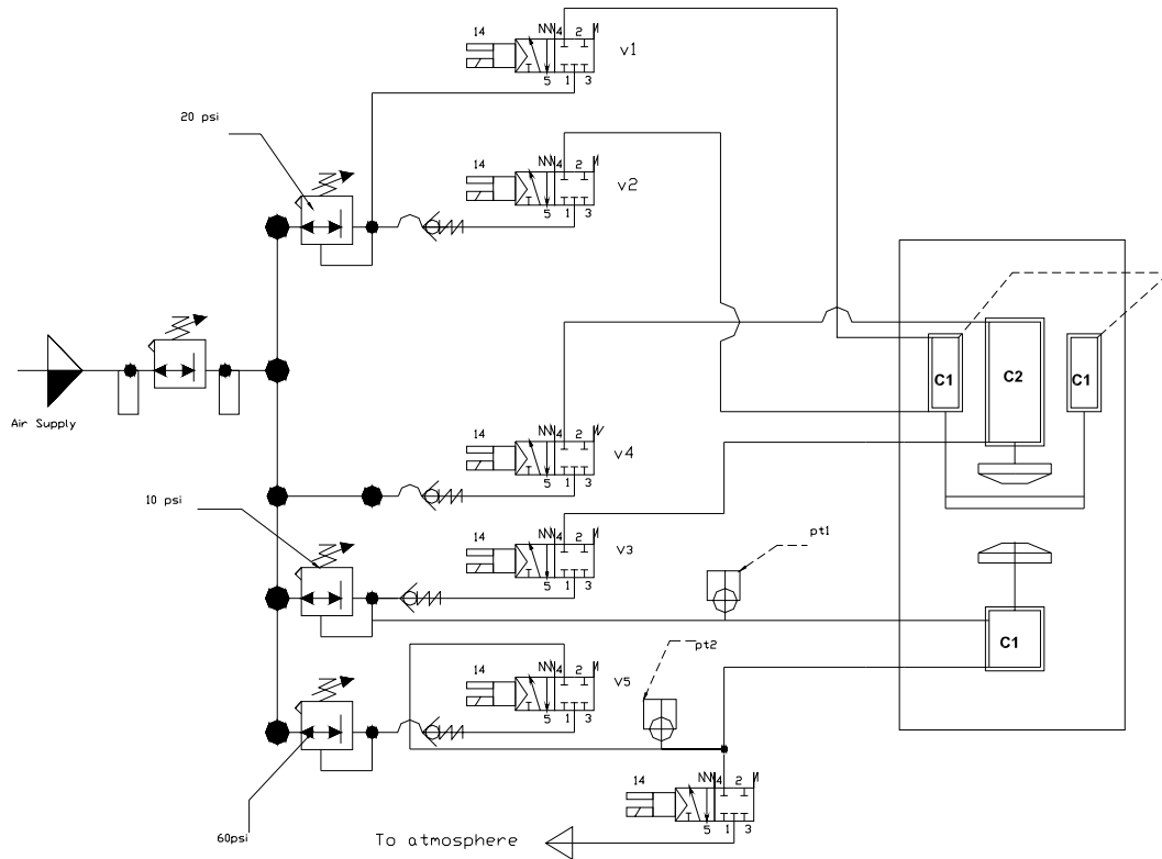
Pneumatic Circuit of Food Tray Tester Designed by Basily B Basily (8/26/06)
