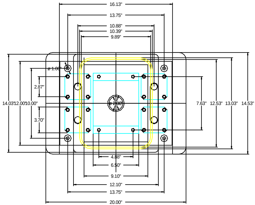
Figure 16: Top View Tester
