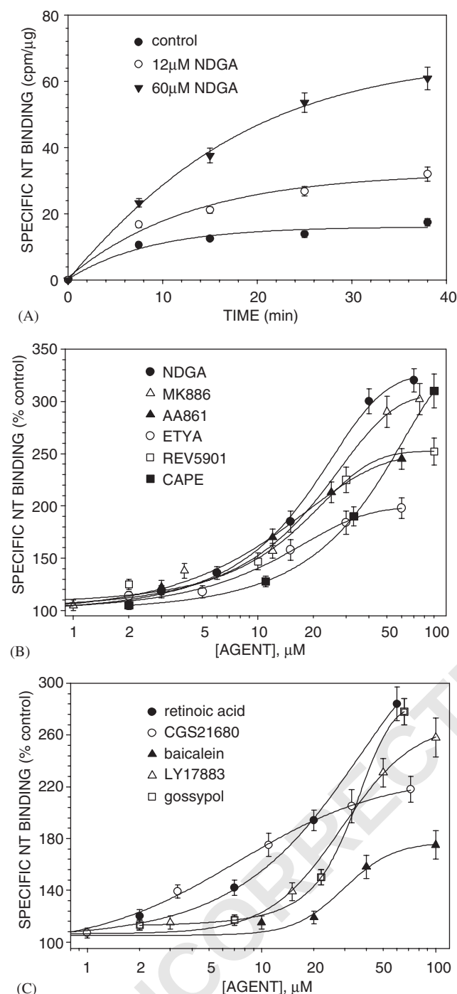
Fig. 1. LOX blockers increased the rate of (A) and the level of (B, C) specific NT binding to PC3 cells. (A) Cells were incubated with indicated concentrations of NDGA or vehicle at 37°C. After 10 min, ^{125}\text{I} -NT ( 10^5 cpm; 50 pM) was added. Incubation continued for times indicated and specific binding was measured. Non-specific binding was <5\% of total binding in all cases (data not shown). The data (mean \pm SEM) were from a typical experiment that was repeated. (B and C) Log dose-response plots for effects of LOX blockers on specific NT binding. Cells were pretreated 10 min with agents indicated, ^{125}\text{I} -NT ( 10^5 cpm; 50 pM) was added and specific NT binding was measured at equilibrium (30 min). The minimum dose that significantly ( P < 0.05 ) increased specific NT binding above control was 2 μM (Rev-5901, retinoic acid), 3 μM (AA861, NDGA, CGS21680), 4 μM (MK886), 5 μM (ETYA), 7 μM (gossypol, LY 171883), 10 μM (CAPE), 20 μM (baicalein). The data (mean \pm SEM) were pooled from at least 4 experiments.
