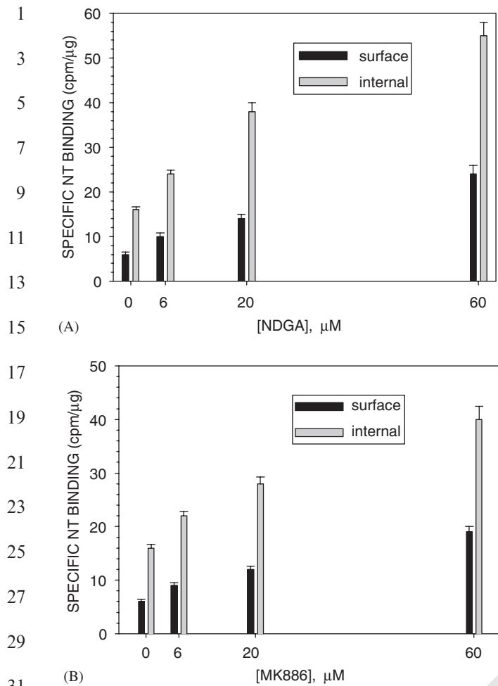
Fig. 3. NDGA (A) and MK886 (B) enhanced cell-surface binding of ^{125}\text{I} -NT, without altering the percentage of ^{125}\text{I} -NT internalized by PC3 cells. Cells were pretreated 10 min with indicated concentrations of NDGA, MK886 or vehicle control. After NT binding was performed at 37^\circ\text{C} for 30 min, the amounts of ^{125}\text{I} -NT bound specifically to the cell surface and internalized were determined by acid washing. The data (mean \pm SEM) were pooled from 3 experiments. In A, internalization as a percentage of total binding was (mean \pm SEM): 73 \pm 2 , 71 \pm 2 , 73 \pm 3 and 70 \pm 5 at the 0, 6, 20 and 60 \mu\text{M} doses. In (B) internalization was 73 \pm 2 , 71 \pm 2 , 70 \pm 2 and 68 \pm 4 at the 0, 6, 20 and 60 \mu\text{M} doses.
