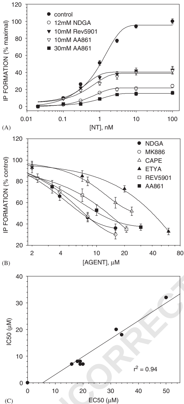
Fig. 2. NT-induced IP formation was inhibited by LOX blockers. (A) Log dose-response plots for the effect of NT in the presence and absence of LOX blockers. NT increased IP formation \cong 5-fold, with EC_{50} \cong 1.0 nM. The efficacy of NT, but not its potency, was reduced by LOX blockers. The data (mean \pm SEM) were from a typical experiment that was repeated. (B) Log dose-response plots showing that IP formation in response to a maximal dose of NT (30 nM) was inhibited by LOX blockers. The minimum dose that significantly ( P < 0.05 ) decreased the response to NT was 4 \mu M (NDGA, MK886, AA861), 7 \mu M (Rev5901), 8 \mu M (CAPE) and 20 \mu M (ETYA). The data (mean \pm SEM) were pooled from 3 experiments. (C) Plot showing that the ability of LOX blockers to inhibit NT-induced IP formation ( IC_{50} ) correlated to the ability to enhance NT binding ( EC_{50} ). The values shown in the plot were determined from studies such as those in Figs. 1B, C and 2B, and are presented in Table 1 for the agents used. The plot yielded a correlation coefficient r^2 = 0.94 .
