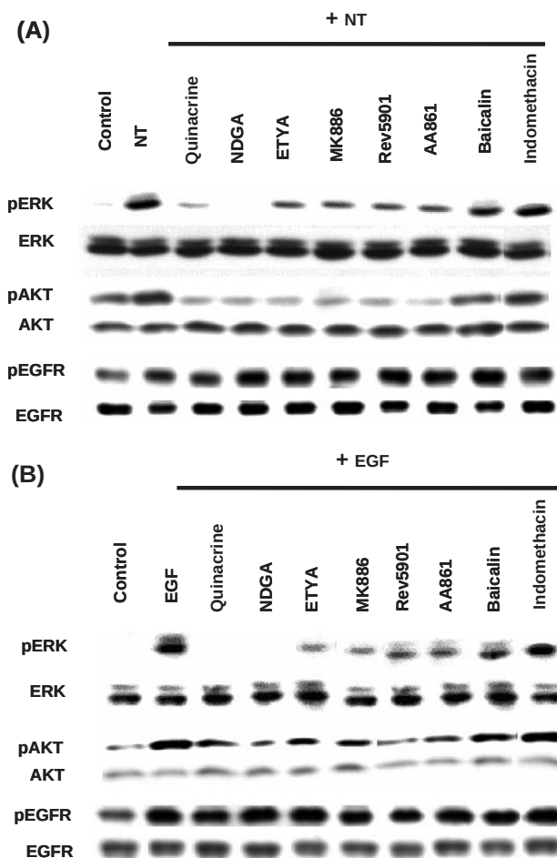
Fig. 6. Effect of various inhibitors of PLA2, LOX and COX on phosphorylation of ERK, AKT and EGFR in response to NT (A) and EGF (B) in PC3 cells. Quiescent cells were preincubated with PLA2 inhibitor (quinacrine, 30 \mu M) or LOX-inhibitors (NDGA, 30 \mu M; ETYA, 30 \mu M) or FLAP inhibitor (MK886, 30 \mu M), selective 5-LOX inhibitors (Rev5901, 30 \mu M; AA861, 30 \mu M), 12-LOX inhibitor (baicalin, 30 \mu M), COX inhibitor (indomethacin, 50 \mu M), or control (0.3% DMSO) for 15 min and then stimulated with NT (20 nM) or EGF (1 nM) for 3 min. Shown is a typical result for an experiment that was performed 3 times. Note that LOX blockers inhibited the effects of NT and EGF on phosphorylation of ERK and AKT without altering the effects on phosphorylation of EGFR.
