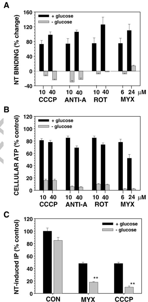
Fig. 6. Inhibition of both glycolysis and oxidative phosphorylation greatly suppressed NT binding (A), reduced cellular ATP levels to <15% control (B), and increased the inhibitory effects of mitochondrial blockers on NT-induced IP formation (C). In (A), cells were preincubated 20 min in Locke (+ glucose) or in Locke minus glucose (– glucose). The mitochondrial inhibitors were added at concentrations indicated and after 10 min, ^{125} I-NT was added. Specific NT binding was measured at equilibrium (30 min). The % increase or the % decrease in NT binding was determined relative to control. Data (mean \pm SEM) were from 3 experiments. In (B), cells were treated as in (A), and cellular ATP was measured after 40 min and expressed as % control. Data (mean \pm SEM) were from 3 experiments. In (C), glucose was withdrawn from half the cells for 10 min. DMSO (0.1%), myxothiazole (5 \mu M) and CCCP (10 \mu M) were added and after 10 min, cells were stimulated with 30 nM NT for 30 min. IP formation was measured and expressed relative to the + glucose control. Data (mean \pm SEM) were from 2 experiments. **Result for – glucose was significantly different from result for + glucose ( p < 0.01 ).
