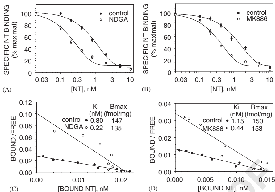
Fig. 4. Binding displacement curves (A, B) and Scatchard plots (C, D) for 125 I-NT binding to PC3 cells in the presence and absence of LOX blockers (NDGA and MK886). Specific binding of 125 I-NT (15.6 cpm/μg protein) measured at equilibrium was increased 2.9-fold by 50 μM NDGA and 2.6-fold by 50 μM MK886. (A, B) Log dose-response plots show displacement of specific 125 I-NT binding by NT, in which binding was expressed as percentage of control. The agents shifted the curves to the left. Results are from a typical experiment repeated twice. (C) Scatchard plots for a typical experiment showing that NDGA increased NTR1 affinity (apparent Ki: control, 0.80 nM; NDGA, 0.22 nM) without increasing receptor number (Bmax: control, 147 fmol/μg; NDGA, 135 fmol/μg). (D) Scatchard plots for a typical experiment showing that MK886 increased NTR1 affinity (apparent affinity: control, 1.15 nM; MK886, 0.44 nM) without much effect on receptor number (Bmax: control, 150 fmol/μg; MK886, 153 fmol/μg).
