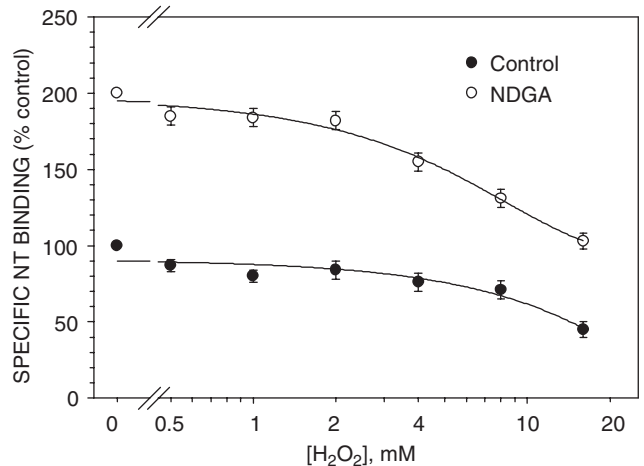
Fig. 8. H_2O_2 dose-responsively reversed the NDGA-induced elevation in NT binding in PC3 cells. After PC3 cells were incubated with 25 \mu M NDGA or vehicle for 10 min, H_2O_2 was added at the indicated doses and specific NT binding was measured at equilibrium (30 min). The data were expressed as a percentage of the binding measured in cells treated with the vehicle control (0.25% DMSO) and represent 3 experiments (mean \pm SEM).
