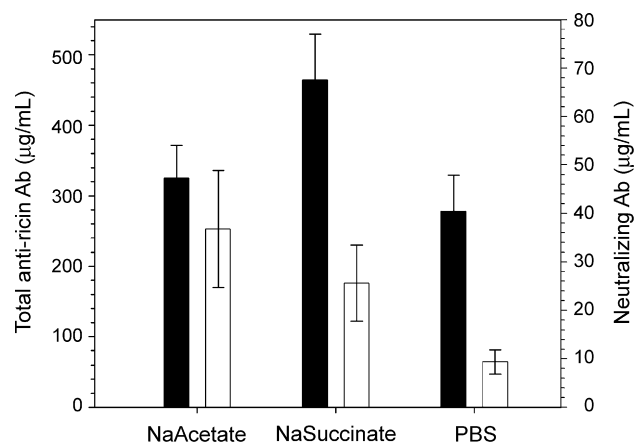
Fig. 3. Total anti-ricin IgG (black, left axis) and neutralizing antibody concentrations (white, right axis) from the sera of vaccinated mice.
