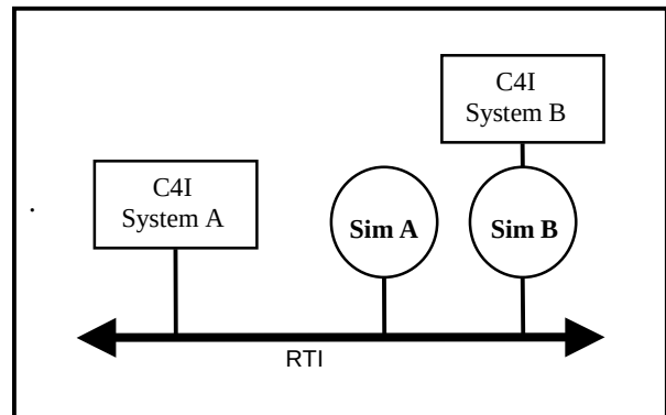
Figure 2. C4I/Simulation Federation
