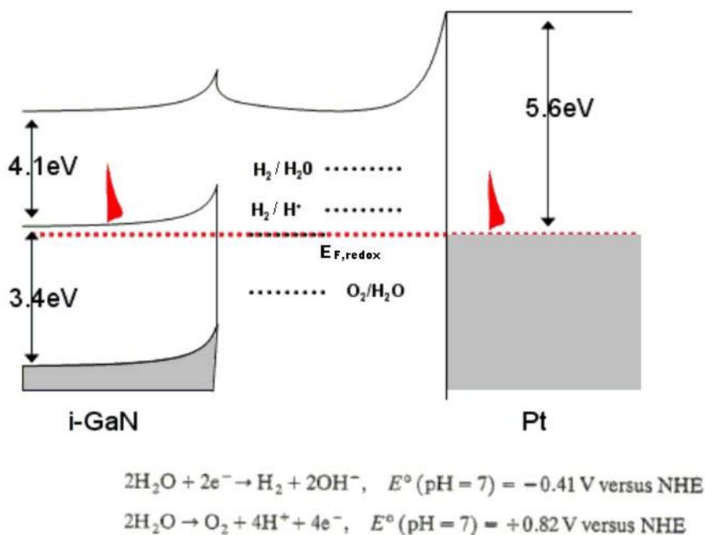
Figure 2.2.1 Band diagram of the electrochemical circuit before bias applied
