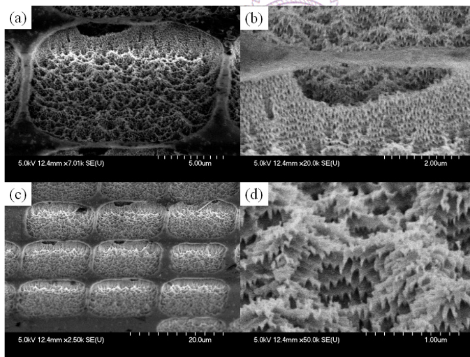
Figure 4.1.1.4.11 The SEM microscopy of the LED after BTELPEC-CS etching (a) hole-pattern (b) under cut of NiAu on p-type GaN. (c) hole-pattern array (d) n-type GaN etched surface
