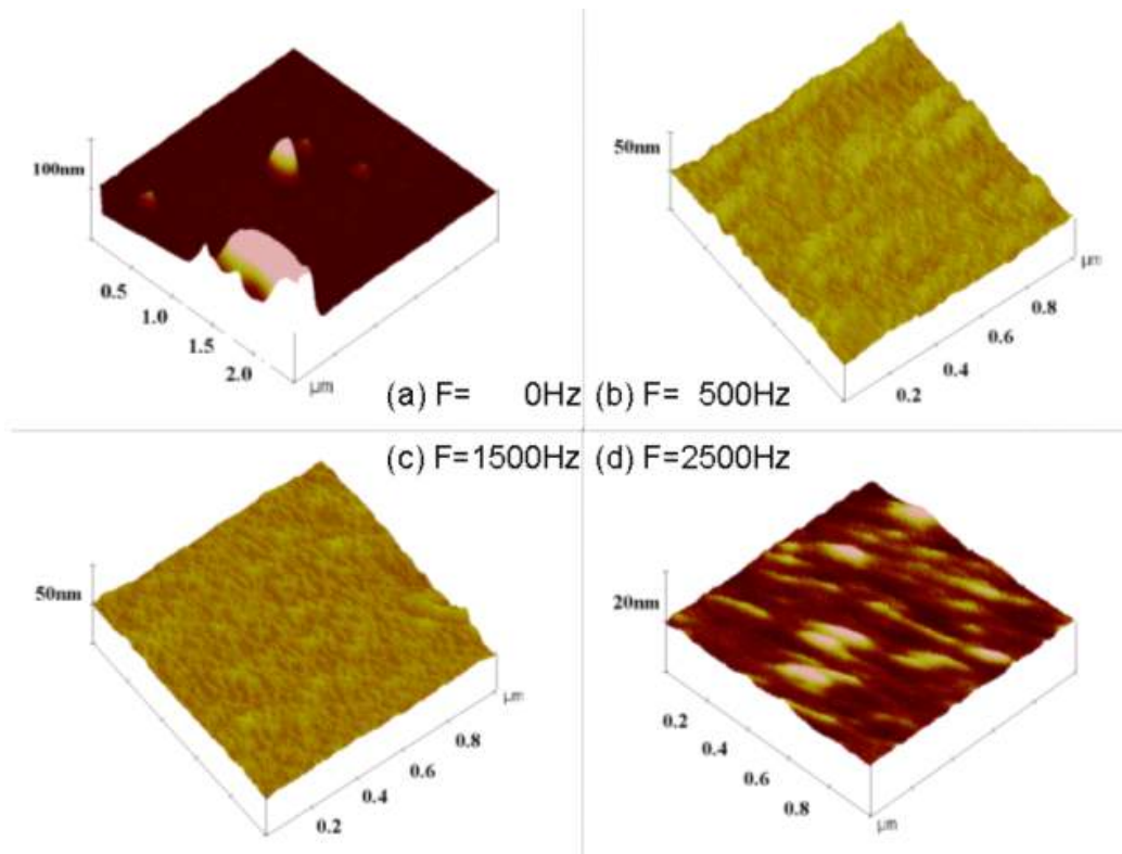
Figure 2.5.1.2 AFM images of a GaN surface obtained from EPPEC etching with varied chopper frequencies: (a) 0 Hz; (b) 500 Hz; (c) 1500 Hz; (d) 2500 Hz. The RMS The RMS roughnesses of resulting GaN are 9.1, 1.34, 0.95, and 0.37 nm, respectively. The GaN samples were etched in solution (0.01 M KOH, 0.05 M K_2S_2O_8 ) for 20 min. (From Hwang's group)
