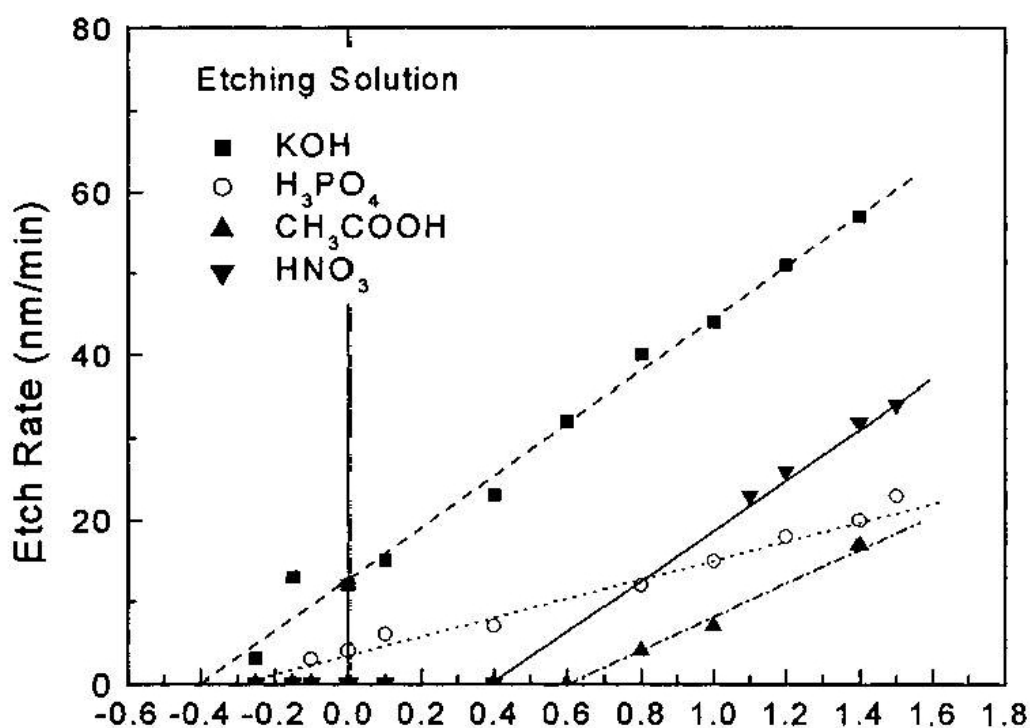
Figure 2.3.1.2 Etch rate for n-GaN on appiled bias form various etching solution under the UV intensity of 90\text{mW}/\text{cm}^2 . The figure is reproduced from J.W. Seo (2001).
