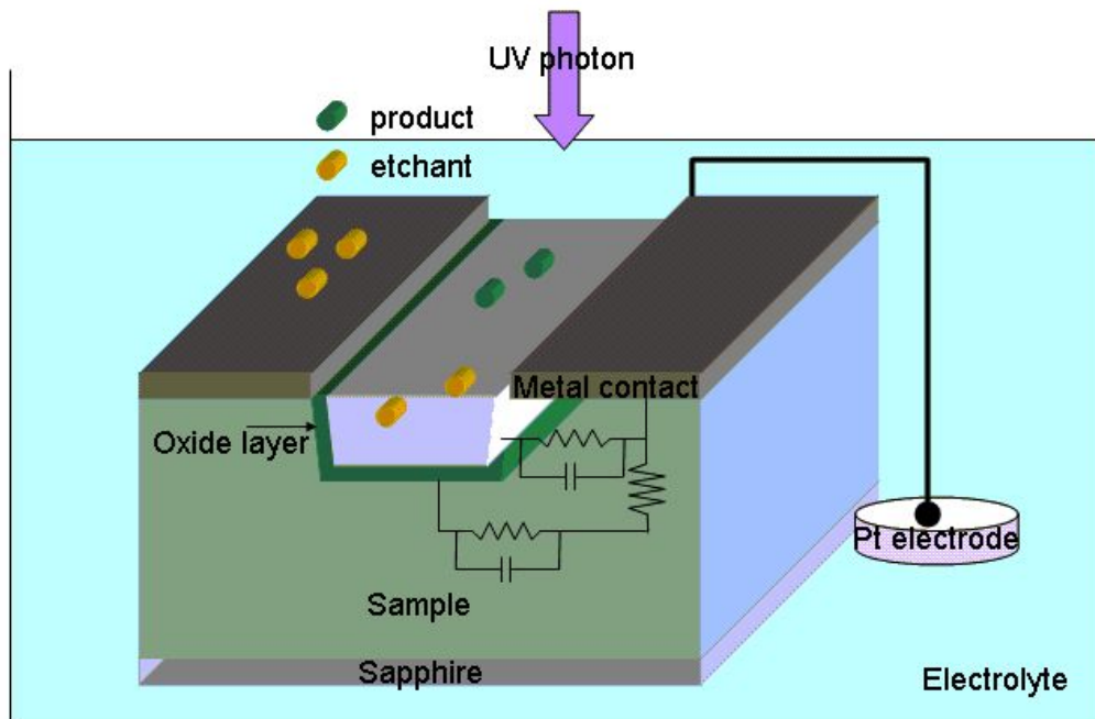
Figure 2.3.1 the diagram of PEC etching III-Nitride
