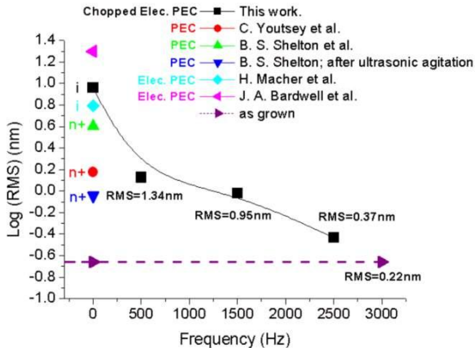
Figure 2.5.1.6 Comparison of RMS roughnesses for PEC etched GaN surfaces from previously reported results and the present work. Etching methods include photoelectrochemical (PEC), electrodeless PEC (Elec. PEC) and chopped-UV-assisted electrodeless wet etching (Chopped Elec. PEC). The samples were unintentionally-doped GaN (i) and n^+ -GaN ( n^+ ). (From Hwang's group)
