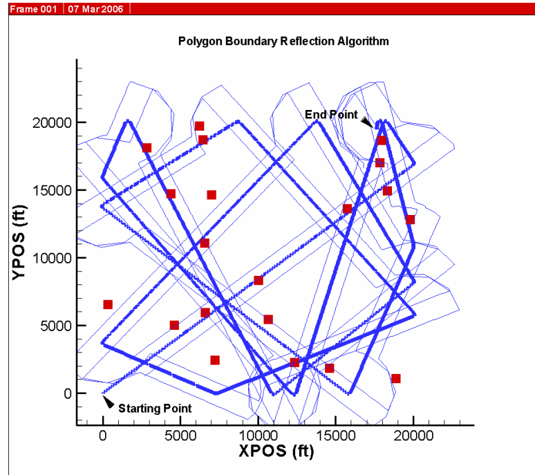
Figure 9. PBRA Trajectory
