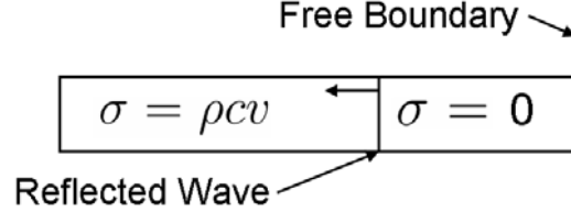
Figure 2.5: Reflection of a Stress Wave
