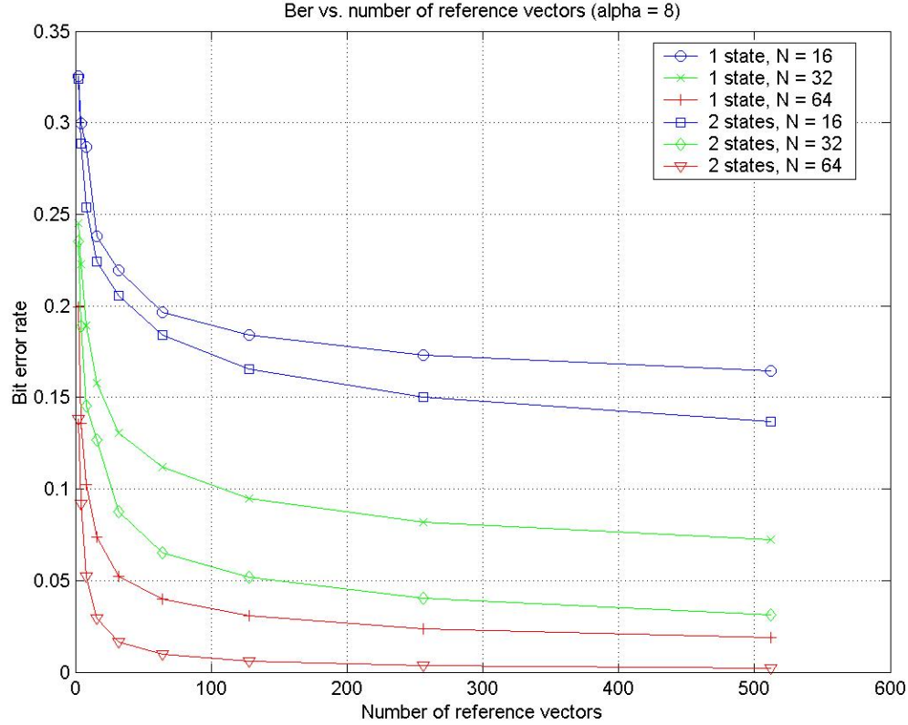
Figure 1: BER vs. number of reference vectors (Number of states = (1, 2), \alpha = 8 )
