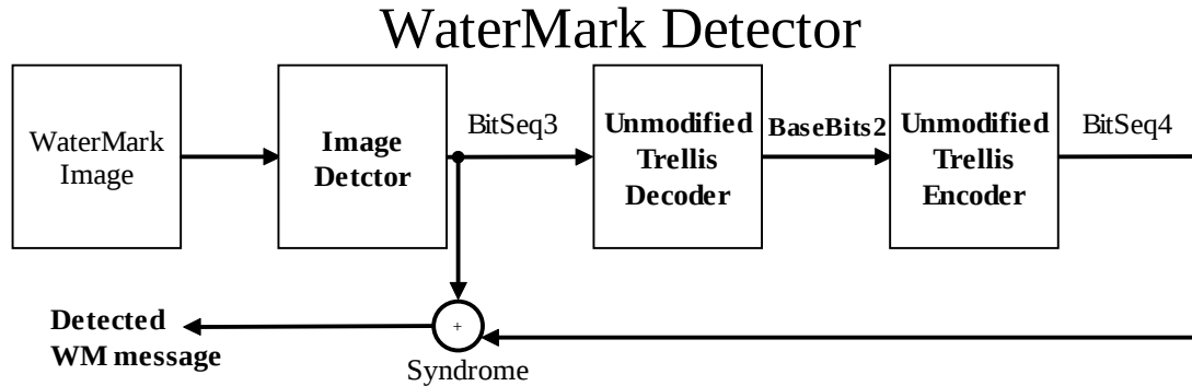
Figure 2. Watermark Detector
