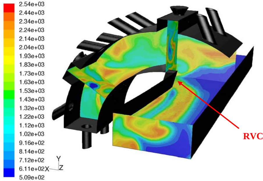
Figure 7: Curved sectional 2-D rig used by Moenter for CFD comparisons of the final design. This plot shows contours of temperature (K). Airflow is to the right in the cavity and out of the page in the main vane. (Moenter, 2006: 112)
