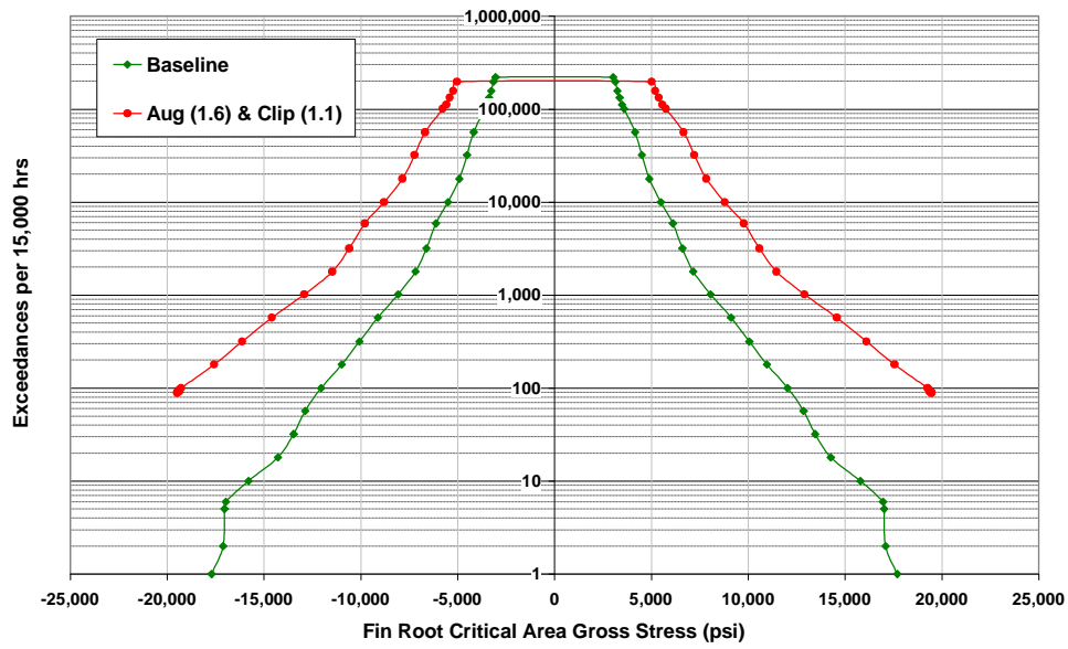
Figure 20: Baseline and Augmented spectra
