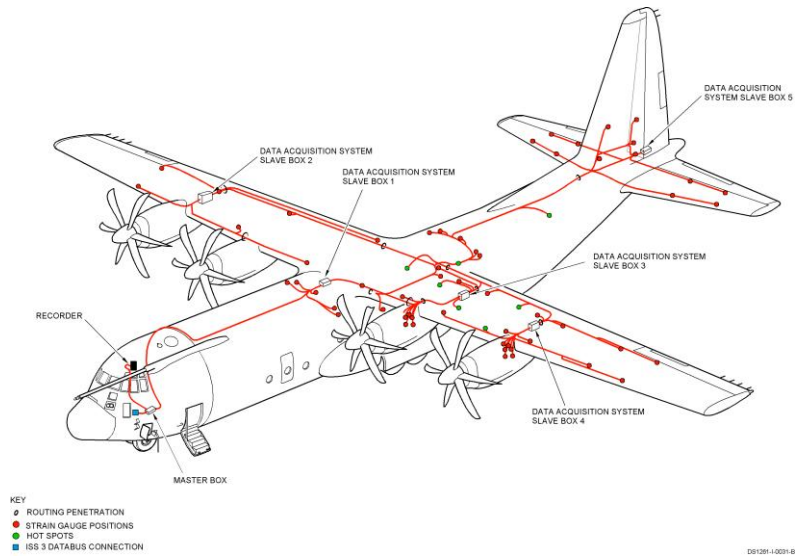
Figure 29: RAAF - Marshall Aerospace OLM Installation
