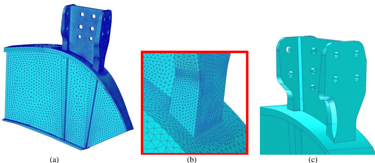
Figure 80: Typical finite element baseline model and optimised repair shape: (a) overall model, (b) detail at critical region, (iii) solid geometry of reduced length optimal
