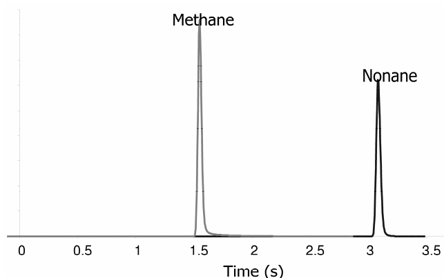
Figure 7. The methane and nonane peaks seen in the 3 meter column at high velocity
