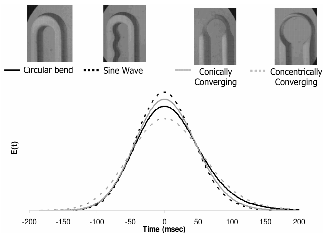
Figure 2. The methane peaks observed on serpentine columns with different turn geometries measured on a 0.3 m long column. Notice that the sine wave bends give lower dispersion than any of the other geometries
