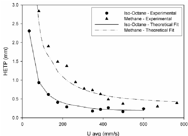
Figure 6. Golay plots for methane and iso-octane separation in 100 micron diameter, 3 meter long serpentine column.
