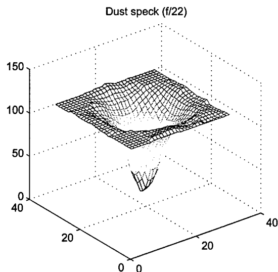
Fig. 3. Intensity loss due to dust speck ( f/22 )
