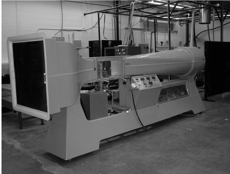
Figure 3.2: Photograph of the Aerolab wind tunnel.
