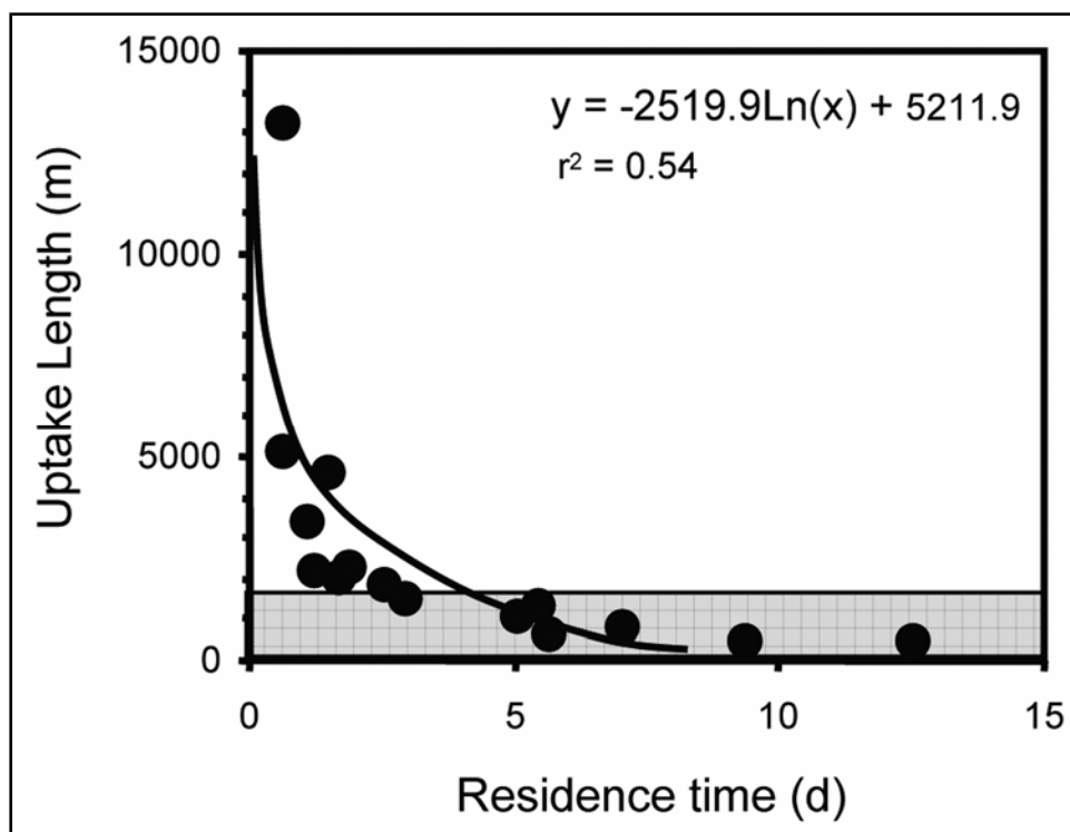
Figure 4. Relationships between residence time and uptake length. Shaded area represents the length of the backwater systems.
