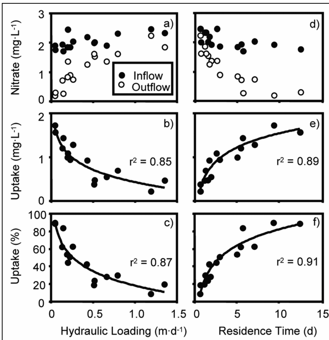
Figure 2. Relationships between hydraulic loading or residence time and nitrate nitrite-N concentrations in the inflow versus outflow, uptake capacity, and uptake efficiency. Values represent means over the summer period (May-September) for 2003-2005.
