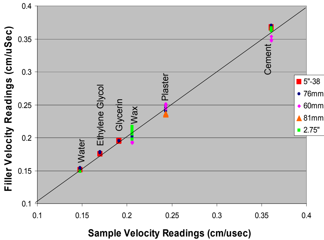
Figure 18. Measured acoustic velocities for several case types and fillers plotted versus the “true” velocity for the filler material.
