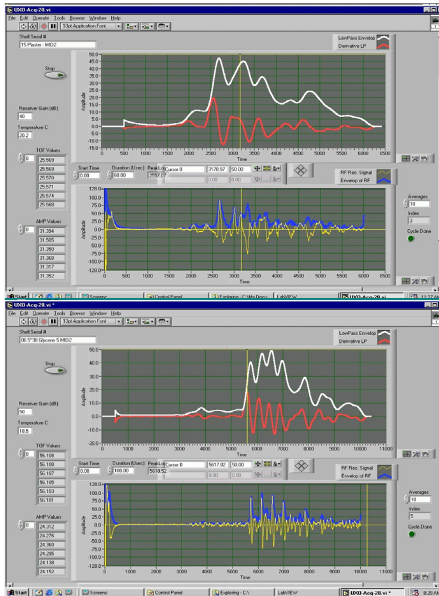
Figure 7. Example waveforms: Top - 76 mm projectile filled with plaster; Bottom - 5” projectile filled with glycerin
