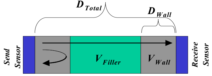
Figure 3. Schematic of sensors attached to projectile body and ultrasonic waves passing through the case and filler.
