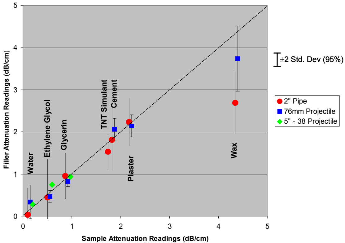
Figure 11. Attenuation readings discriminate between filler types.
