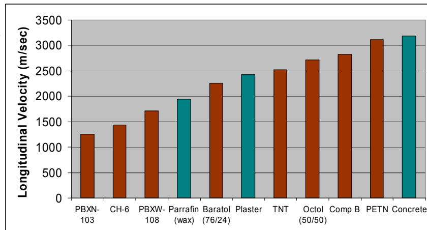
Figure 1 Comparison of the acoustic velocities for several common explosives (red) and inert (green) fillers.
