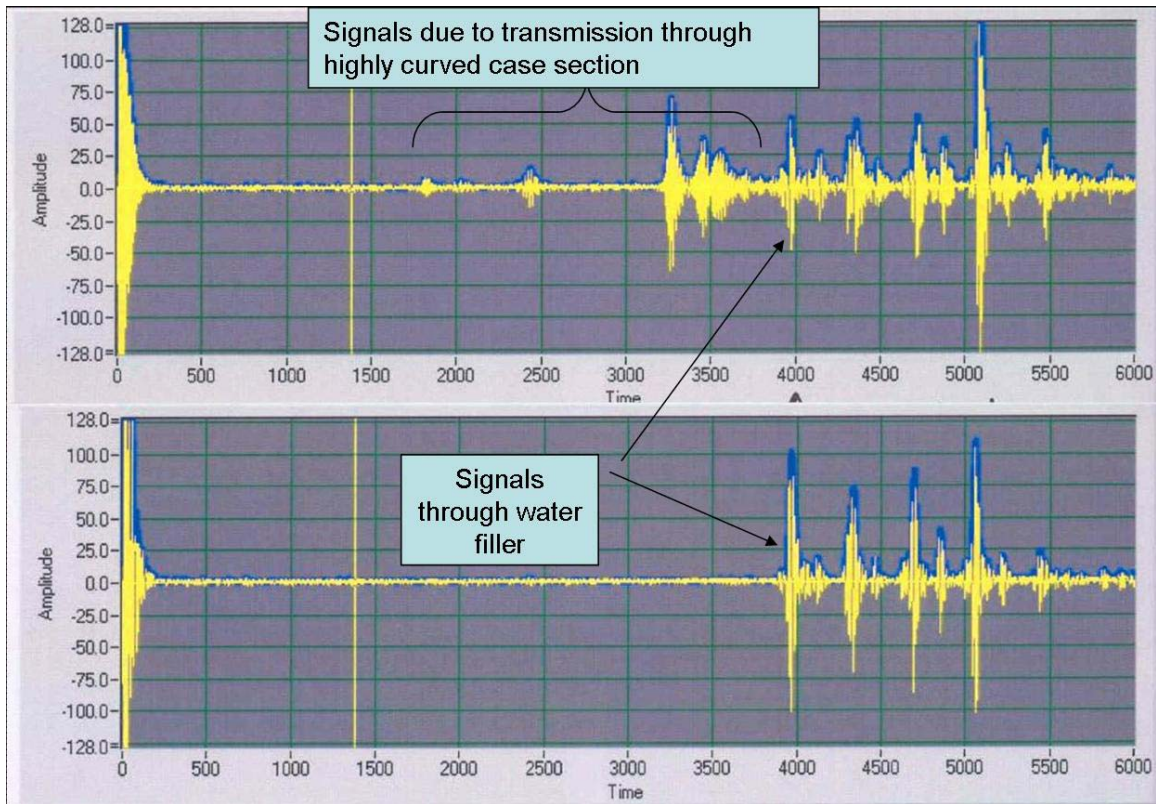
Figure 15. Acoustic signals for water filled 76 mm shell. Top trace: 5MHz sensors located flat against the case near a section where the ID was highly curved. Lower trace: same location but with the sensors tilted by 5°.
