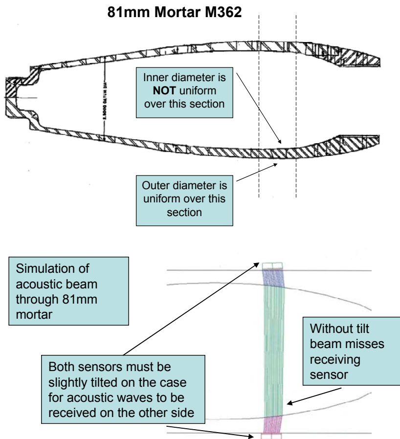
Figure 14. Illustration for a curved-case shell showing how a slight tilt of the transmitting and receiving sensors will result in a strong signal.
