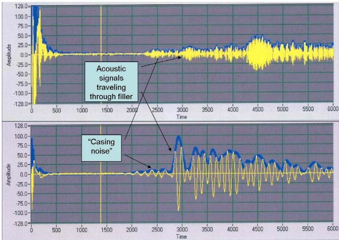
Figure 12. Measured acoustic signal received through a 76 mm casing filled with plaster. The sensor frequency is 5 MHz for the upper time signal trace, and 2.2 MHz for the lower trace.
