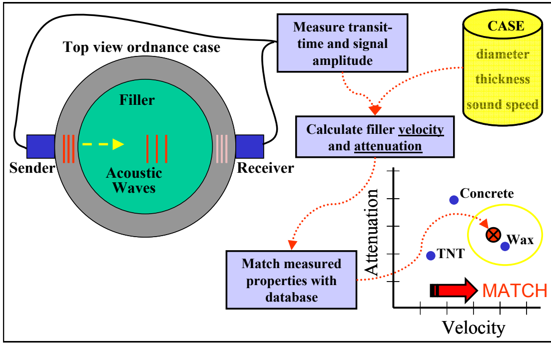
Figure 2. Sketch of the filler-identification system shown attached to an artillery shell.
