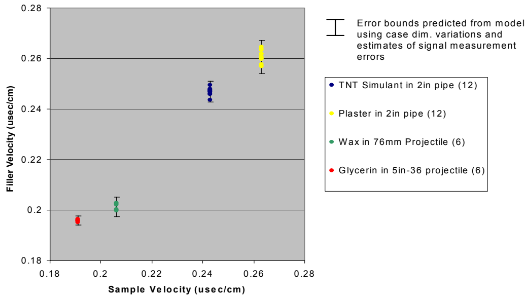
Figure 9. Filler velocity measurement vs. error predicted from model
