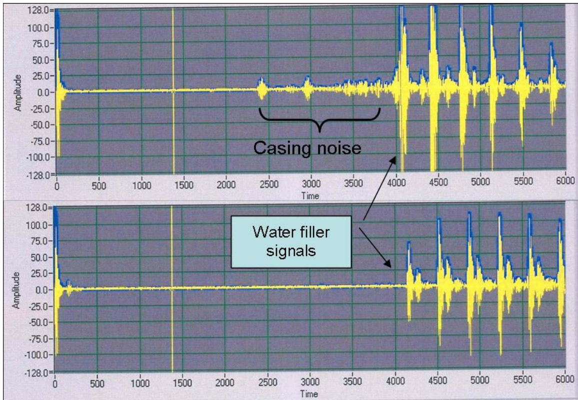
Figure 13. Acoustic signals for a water-filled 76 mm shell. Top trace: 5MHz, flat sensors placed directly against the casing. Lower trace: same sensors with aluminum caps to conform to the case.
