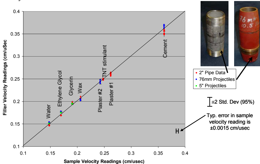
Figure 10. Measured acoustic velocities for several case types and fillers plotted versus the “true” velocity for the filler material.
