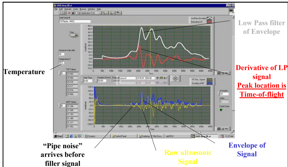
Figure 6. Digital processing for enhanced signal detection (signal for plaster in 76 mm shell).
