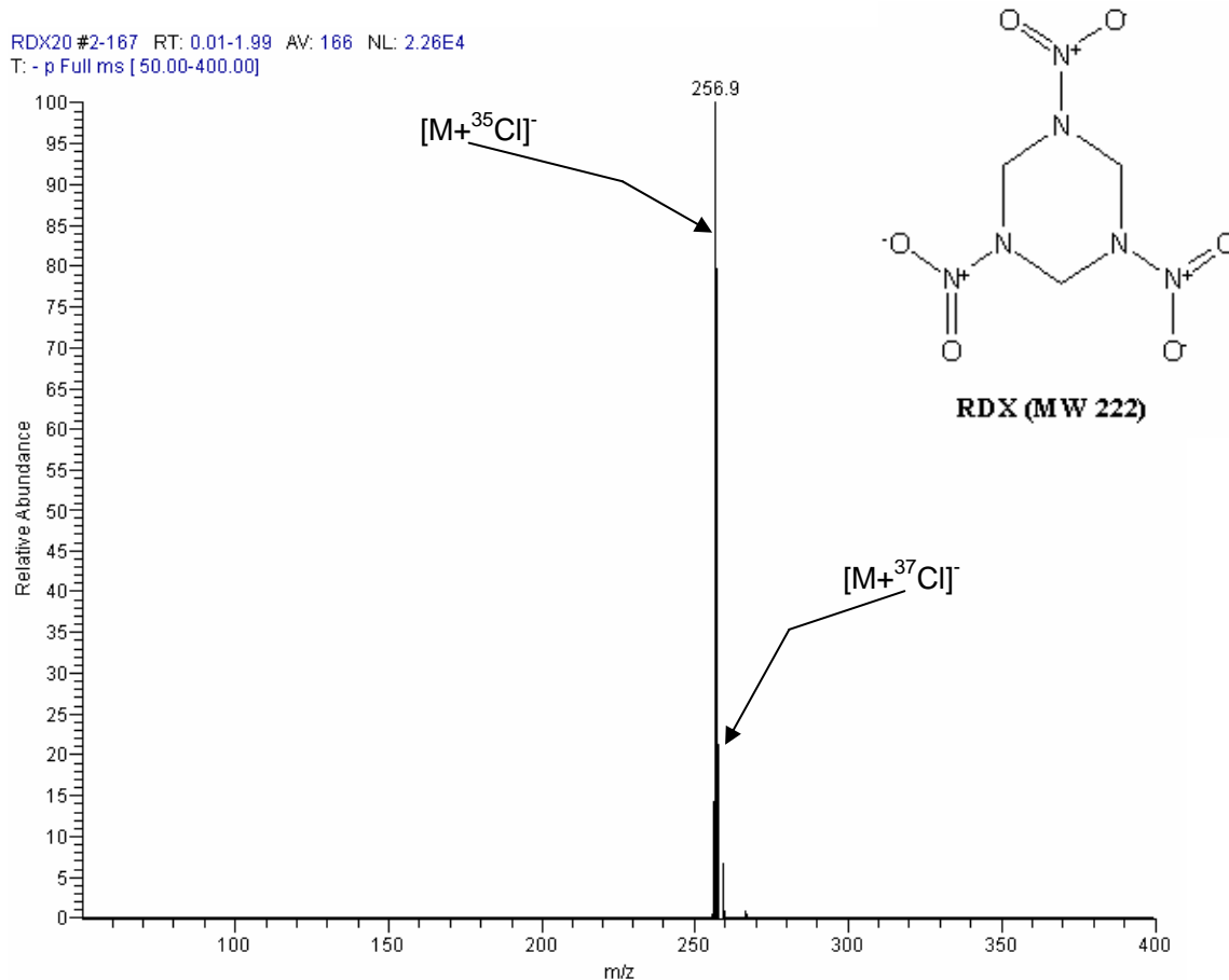
Figure 2-16. RDX: 2 min at CV = 5.1V. Figure 2-16 demonstrates that FAIMS/MS is an effective method of separating and detecting chloride adducts of RDX, as there are no interferences.
