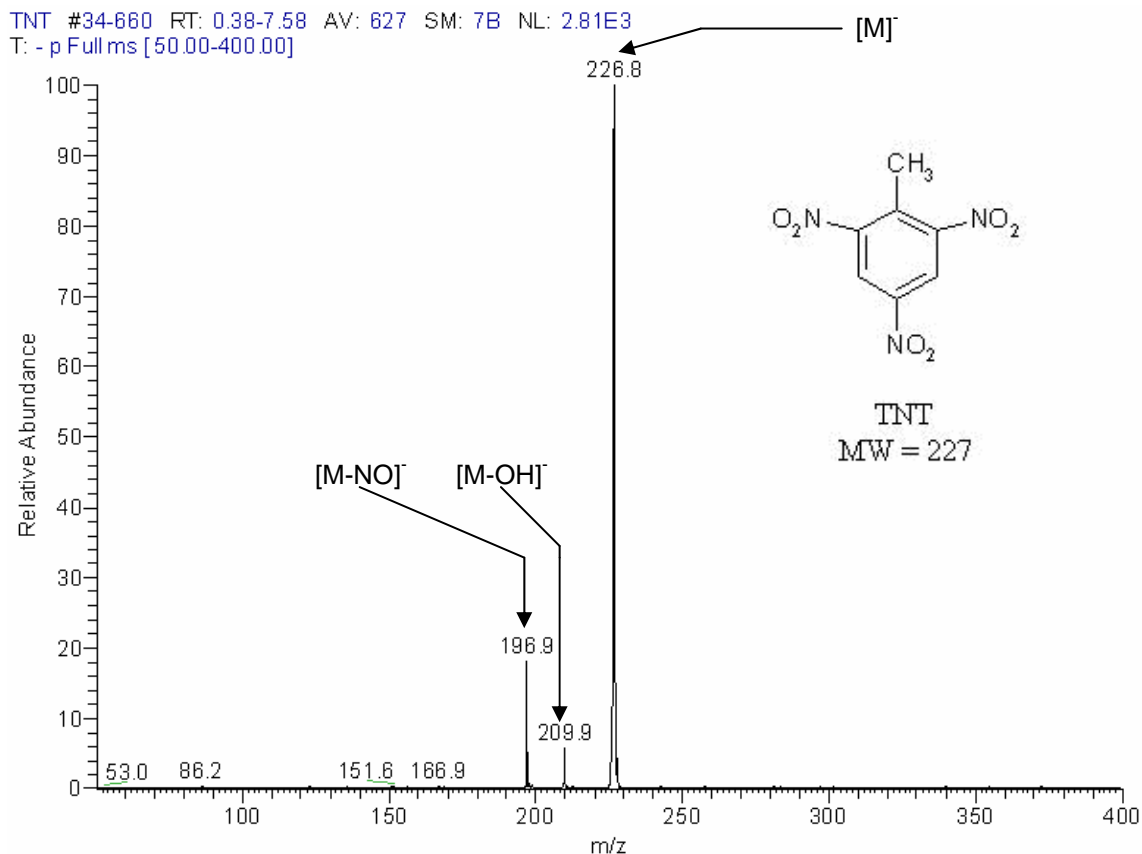
Figure 2-5. FAIMS/APCI mass spectrum of TNT. Figure 2-5 shows the FAIMS/MS spectrum for TNT. The background noise has been greatly reduced after the application of the FAIMS. (see figure 2-2) The evident tradeoff for the improved signal/noise ratio is the 50× reduction in signal strength. In addition, two fragments of TNT also pass through the FAIMS, as the fragment ion CVs are very close to the CV of the TNT [M] - ion. The fragments show that TNT is a delicate ion that readily loses NO and OH. The fragment peaks are in larger proportion to the molecular ion peak when FAIMS is applied, most likely because the total ion count is lower, and there are few to no impurities. Also, the [M-H] - no longer appears.
