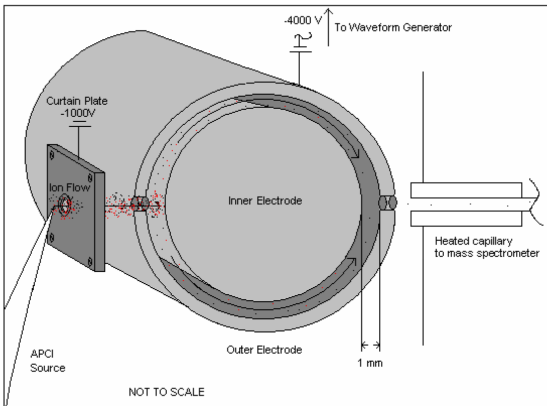
Figure 1-4. Ionalytics line-of-sight FAIMS cell geometry.
