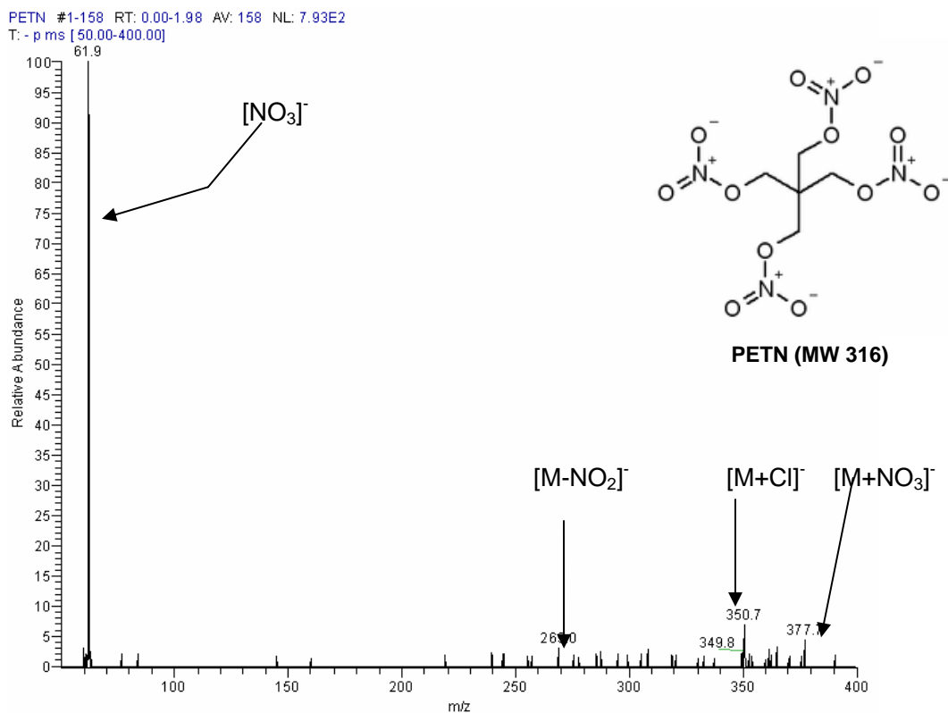
Figure 2-23. FAIMS/MS mass spectrum of PETN. Like the nitroamines and NG, PETN does not yield a detectable molecular ion. It did form both chloride and nitrate adducts; however, these were in extremely low intensity. As a result, PETN did not form any discernable peaks of high intensity during this experimentation. However, due to its extreme instability, (also like NG) PETN did fragment into nitrate ions which were separated and detected by FAIMS/MS (Figure 2-23). As this figure shows, the total ion count is relatively low.
