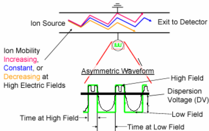
Figure 1-2. FAIMS waveform and ion mobility behavior. [Adapted from Guevremont, Roger. 2004. High-Field Asymmetric Waveform Ion Mobility Spectrometry (FAIMS). (p. 2, fig. 1-1). Ionalytics Corp., Ottawa, Canada.]
