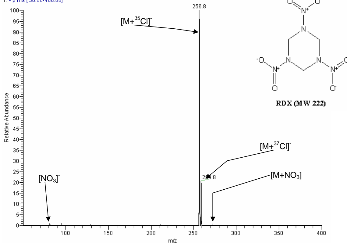
Figure 2-15. FAIMS/MS mass spectrum of RDX. The [M+Cl] - adduct is formed with the small amount of carbon tetrachloride in the solvent. (see Figure 2-15) One property of both RDX and HMX is the formation of little to no molecular ion. Interestingly, the adduct formed of RDX with the 37 Cl isotope of chloride can also be seen in the mass spectrum. The first additional peak shown in the CV spectrum (figure 2-14) is m/z 62 which is an [NO 3 ] - fragment peak; it is seen in many mass spectra of explosives, especially at higher temperatures. The second is a small amount of m/z 286, which is another adduct formed with RDX: [M+NO 3 ] - .
