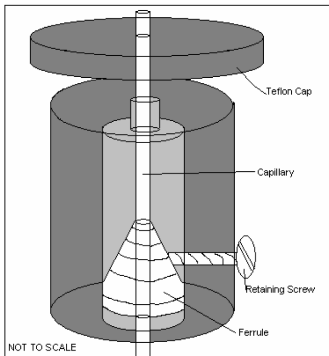
Figure 3-1. WSU electrospray ionization source. Figure 3-1 shows the WSU ESI source. The darkly shaded areas are constructed of Teflon, and the capillary is fused silica. The ferrule used is conductive stainless steel.
