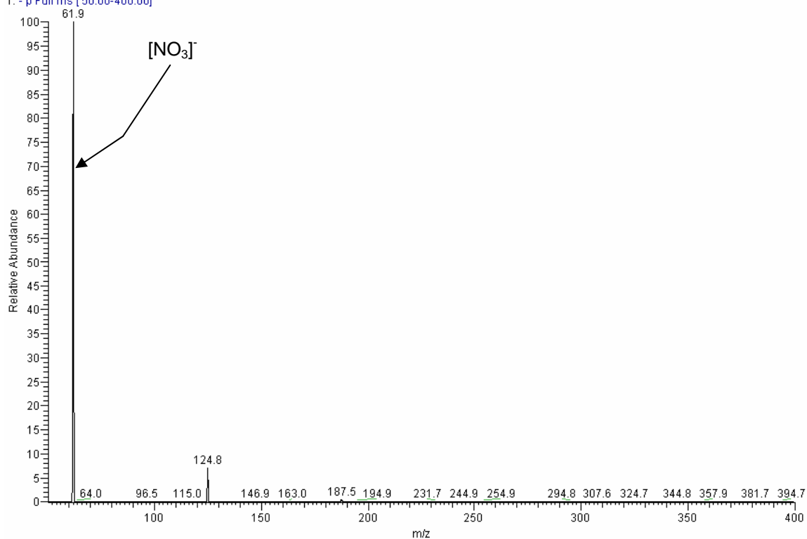
Figure 2-24. FAIMS/MS mass spectrum of ANFO made with hexane. Figure 2-24 shows a FAIMS/MS mass spectrum of ANFO made with hexane. The base peak is [\text{NO}_3]^- , which passed through the FAIMS cell at a CV of 9.7V. There is also a small peak at m/z 125.
