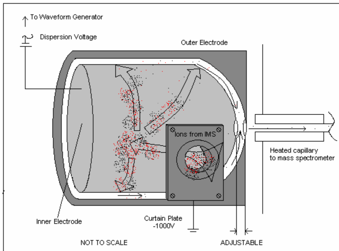
Figure 3-3. Drawing of Ionalytics orthogonal dome FAIMS cell. Figure 3-3 contains a drawing of the orthogonal dome FAIMS cell. The red and black dots describe a simple scenario in which the black dots represent the analyte of interest and the red dots are noise (interferent ions). Both types of ion enter the FAIMS cell through the curtain plate and are separated as the red ions collide with the walls of both electrodes when the proper CV is set. A percentage of the analyte ion is also lost, but this is the only ion type that enters the mass spectrometer.
