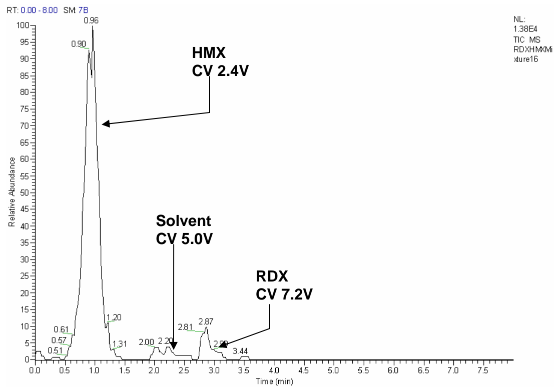
Figure 3-6. CV spectrum of HMX/RDX mixture.
