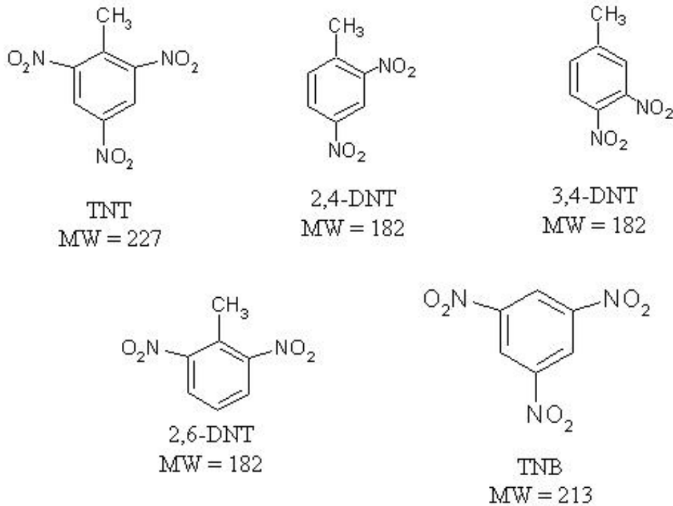
Figure 2-2. Nitroaromatics and molecular weights. [Adapted from Reich, Richard. 2001. (Figure 1-11). PhD dissertation. University of Florida.]
