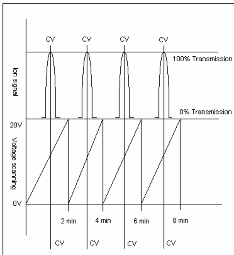
Figure 2-1. Compensation voltage (CV) scanning.
