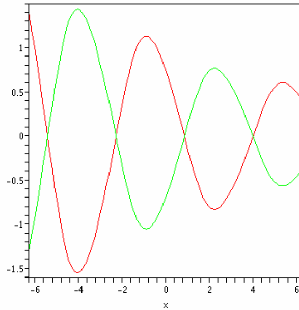
Figure 1-6. Example of oscillating ion motion according to the Mathieu equation (let a=1 and q=1/5 ). [Adapted from McLachlan, N. W. 1947. Theory and Application of Mathieu Functions, Dover].
