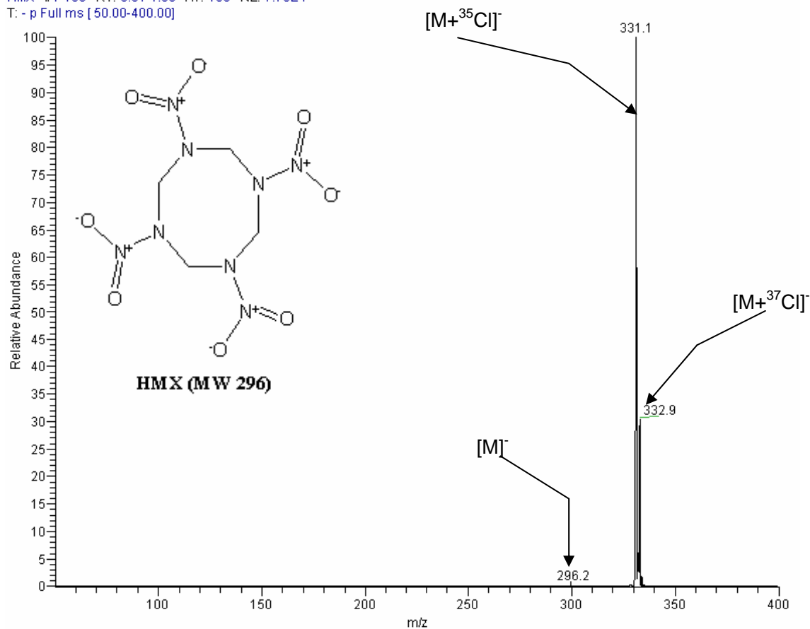
Figure 2-19. HMX: 2 min at CV = 1.2V. Figure 2-19 shows the HMX [M+\text{Cl}]^- peak as the CV is fixed at 1.2V for a period of 2 minutes. The mass spectrum contains no interferences, and there is a small amount of the molecular ion peak, as there was during the CV scans (figure 2-18).
