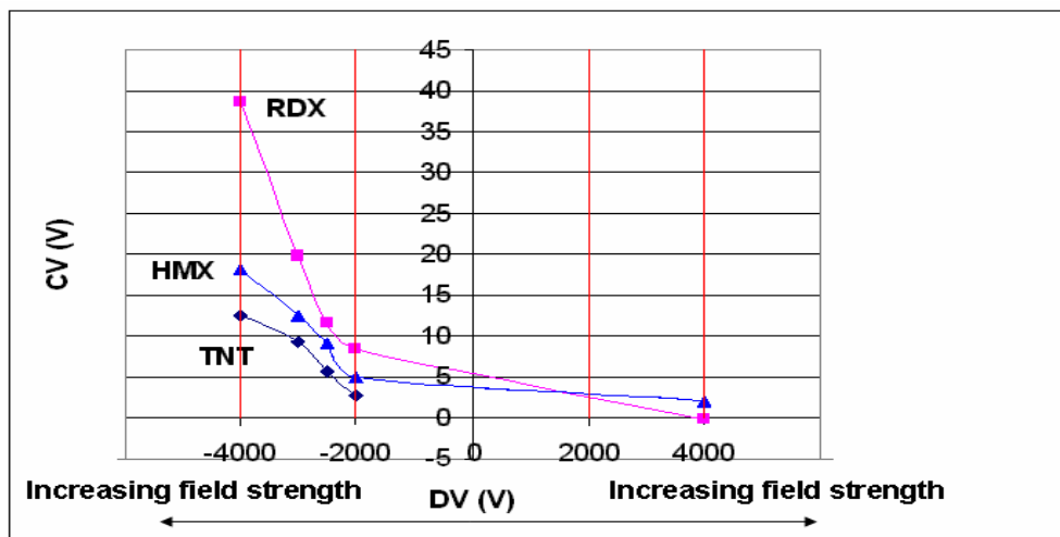
Figure 3-19. Relationship between CV and DV. Figure 3-19 is a plot of the relationship between CV and DV created using data sets taken using the FAIMS/MS setup described in chapter 2. The curves indicate that the CV of each ion increases at more negative DV (hence greater field strength). TNT and other nitroaromatics do not produce ions that are transmitted at a positive DV, although the chloride adduct ions of RDX and HMX respond to both positive and negative DVs. The Ionalytics instrument will not allow the DV to be set less than \pm 2000V or greater than \pm 4000V ; this is indicated by the vertical red lines. Because of this DV/CV relationship, most of the explosives appear to exhibit “B” type behavior when high field is applied.
