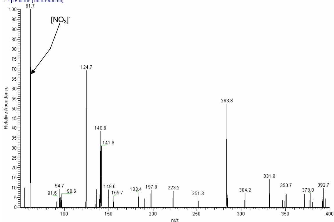
Figure 2-25. FAIMS/MS mass spectrum of ANFO made with nitromethane. ANFO made with nitromethane (figure 2-25) as the fuel has a much lower ion signal than that made with hexane; this behavior was also seen with ANFO made with toluene. It also has a [NO 3 ] - base peak, though there are some other ions as well. These ions were in common with some of the other runs as well: m/z 125, m/z 141, and m/z 284.
