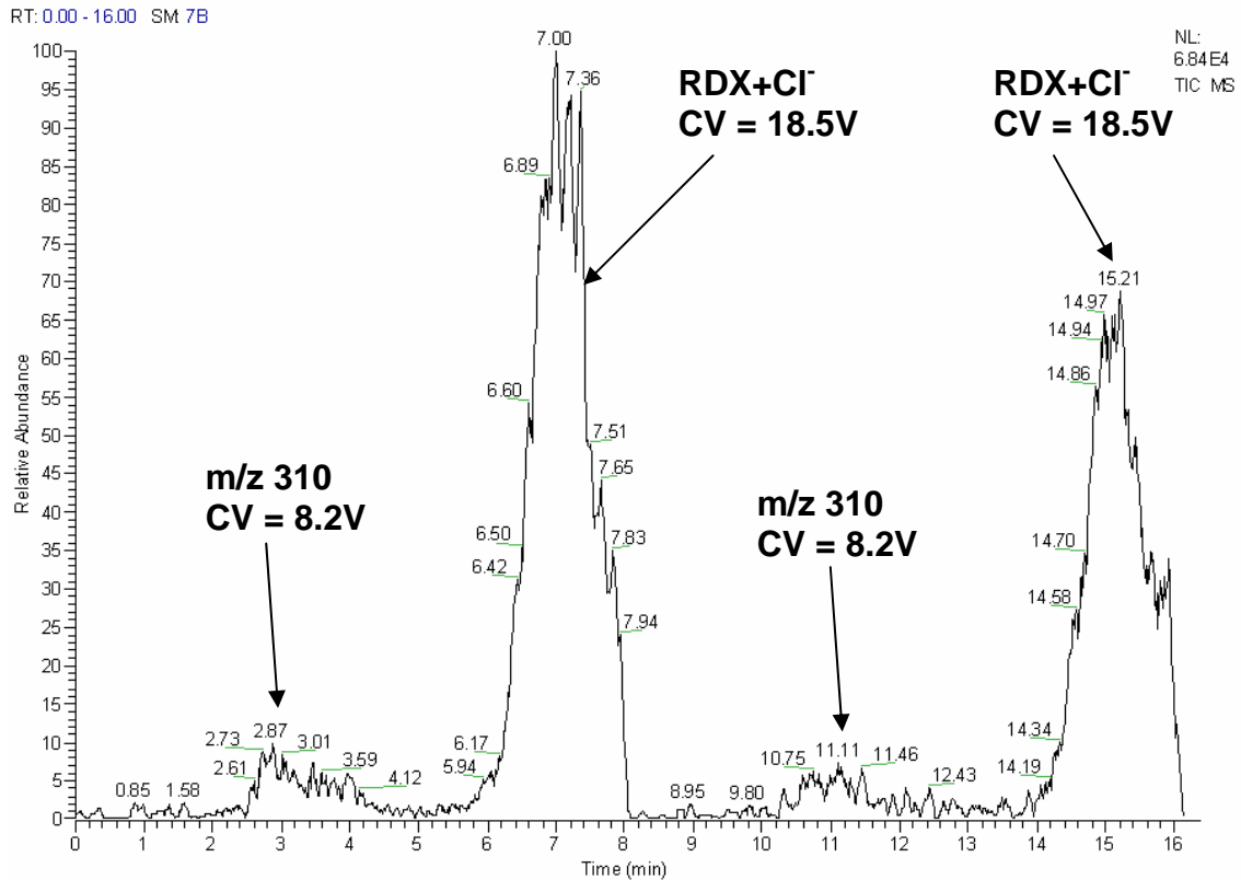
Figure 3-15. RDX CV spectrum at 1.0 mm. Next, the electrode gap was increased by a factor of 1.3, to 1.0 mm (Figure 3-15). The ion count was higher, yet the transmission behavior is completely different from the smaller gaps. This CV spectrum appears much like those in previous chapters, with a well-resolved peak for the analyte ion and only small background. The RDX [M+Cl]^- ion is much more intense, the peak at m/z 310 is much less intense, and the peak at m/z 283 is hardly visible. The maximum ion intensity has increased to 6.84 \times 10^4 counts.
