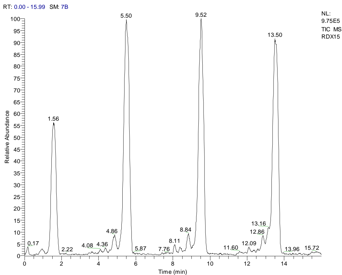
Figure 2-14. CV spectrum of RDX. Figure 2-14 shows the CV spectrum for RDX. The peaks are fairly well reproducible. There are two small peaks before the ion of interest in all four scans, which are identified in figure 2-15.
