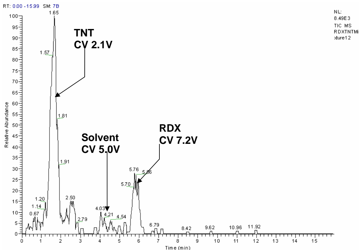
Figure 3-8. CV spectrum of TNT/RDX mixture. A second mixture examined was torpex, which consists of TNT and RDX in approximately equal portions. The only difference between the mixture that was examined here and the military explosive is that in this case there is no aluminum powder. In this case, one CV scan from 0-20V was done over 16 minutes. Once again, both components (see Figure 3-8) are fully resolved from each other and the solvent background in the CV spectrum.
