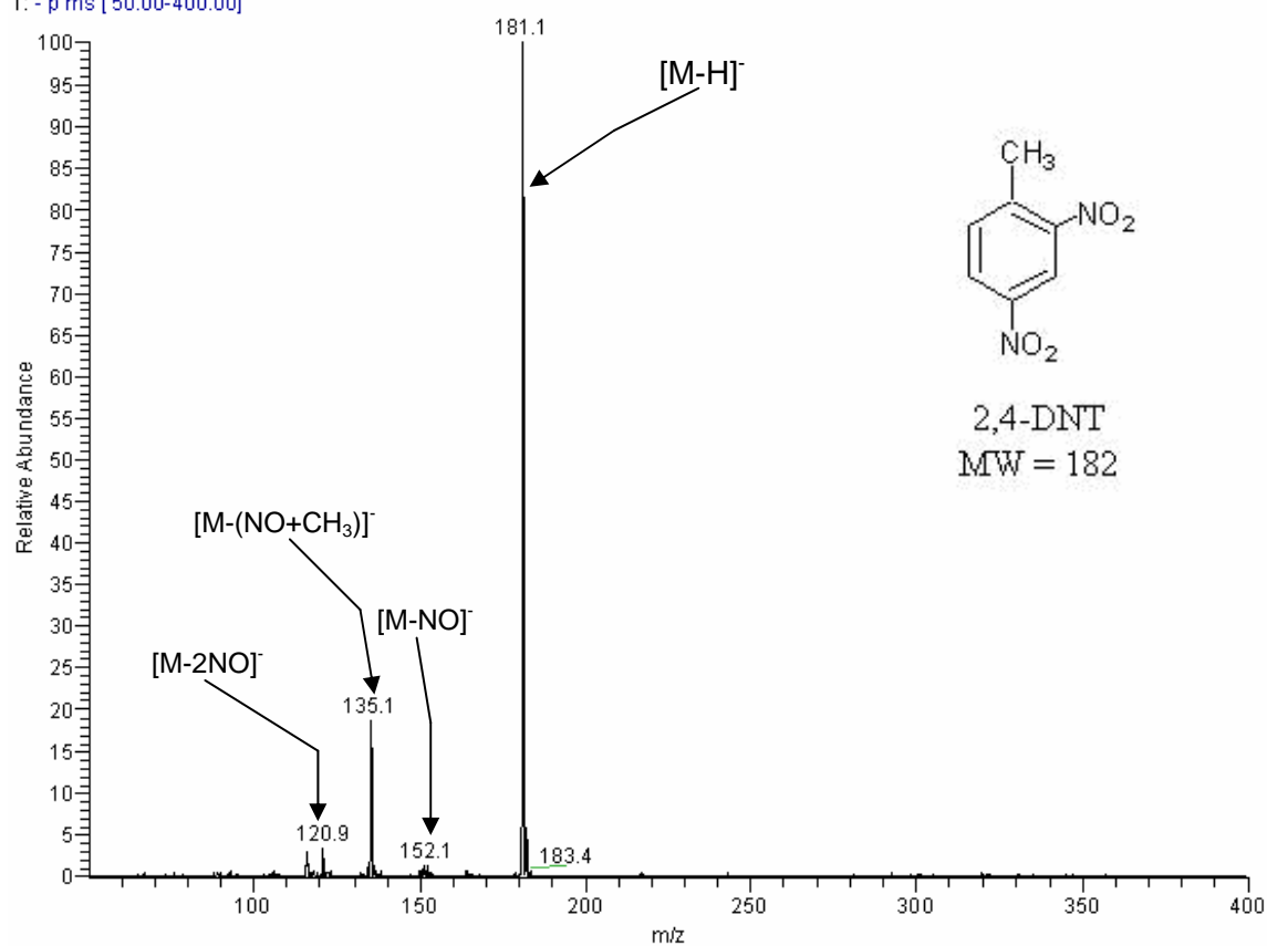
Figure 2-10. 2,4-DNT: 2 min at CV = 11.5V. A mass spectrum of 2,4-DNT at a fixed CV of 11.5V is displayed in figure 2-10. There is little to no noise.
