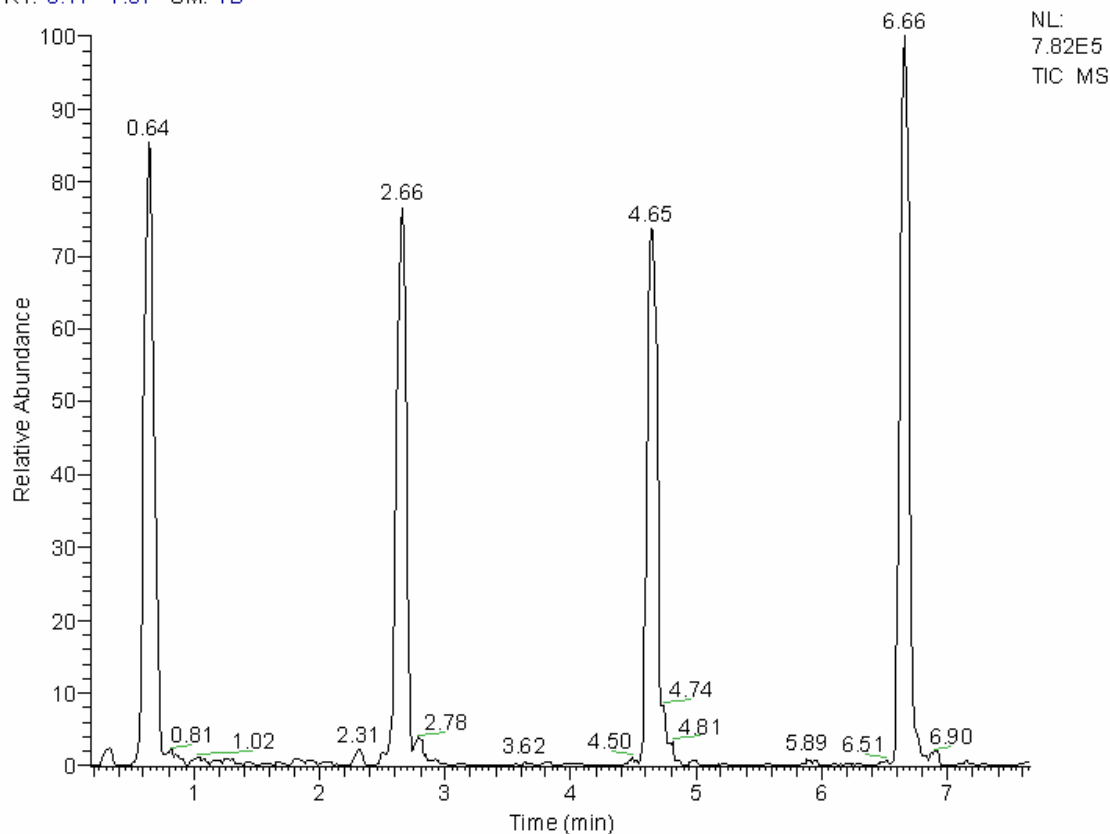
Figure 2-4. TNT total ion count over four 2 min CV scans. Figure 2-4 shows the CV spectrum (total ion count) for TNT. As mentioned earlier, the ion of interest will only pass through the FAIMS at its correct CV; therefore, there are ion peaks at these CV values. There were four CV scans from 0-20 V, each with a duration of 2 min, for a total of 8 min. It is from these spectra that the exact CV for each compound can be calculated. From this spectrum, the CV can be calculated. For instance, the peak at 0.64 min: (0.64 \text{ min}/2.00 \text{ min}) \times 20.0\text{V} = 6.4\text{V} .
