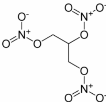
Figure 2-20. NG (MW 227) [Adapted from Paul W. 1996. Explosives Engineering, (Figure 3-3 p. 76), Wiley].
