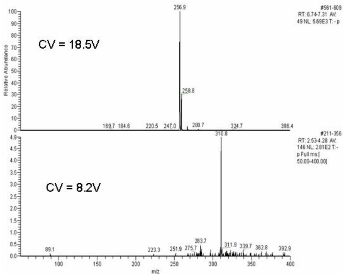
Figure 3-16. RDX mass spectra at 1.0 mm. The mass spectra for RDX taken at a FAIMS electrode gap of 1.0 mm can be seen in Figure 3-16. Thus far, both ion count and resolution are superior to those at smaller electrode gaps. At this gap, resolution and ion count are well-balanced. Likely, the electric field is at a strength optimal for ion focusing. Note that the peak at m/z 267 is barely visible.
