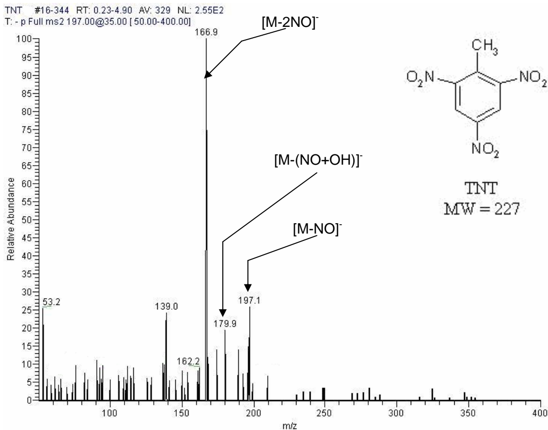
Figure 2-7. FAIMS/MS/MS of TNT m/z 197.1 peak at 35% collision energy. Figure 2-7 demonstrates that FAIMS/MS/MS of even weak ions from explosives is feasible. The FAIMS CV was set to 6.2V to allow the [M-NO]^- fragment of TNT to pass through the cell. This ion was collided with 35% dissociation energy, causing the loss of a second nitro group. In other words, the predominant fragment ion peak shown here is the same elemental composition as the [M]^- ion for mononitrotoluene.
