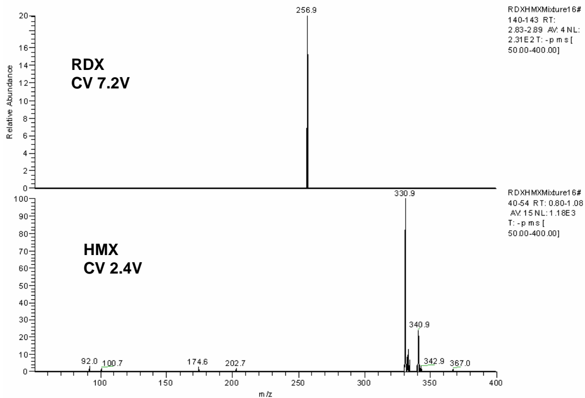
Figure 3-7. Mass spectrum of HMX/RDX mixture. Figure 3-7 contains the mass spectra of the RDX/HMX mixture, showing the [M+Cl]^- adducts of both RDX ( m/z 257) and HMX ( m/z 331) taken from the relative CV peaks (which are seen in Figure 3-6). The HMX peak at m/z 341 is an [M+NO_3]^- adduct
