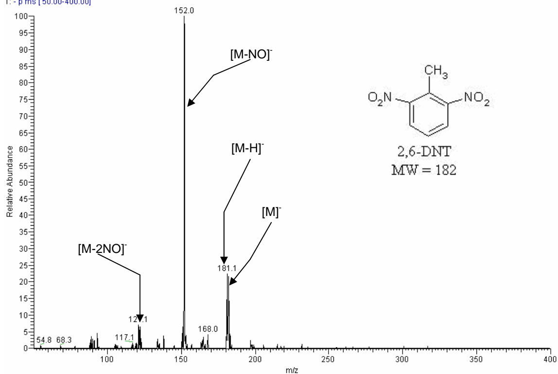
Figure 2-12. FAIMS/MS mass spectrum of 2,6-DNT. Figure 2-12 is a mass spectrum averaged over the entire 8 min run. The two predominant ions are visible at m/z 181 ([M-H] - ) and m/z 152 ([M-NO] - ), as described at figure 2-11.
