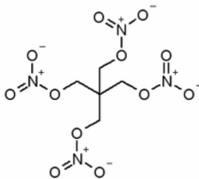
Figure 2-22. PETN (MW 316). [Adapted from Paul W. 1996. Explosives Engineering, (Figure 3-3 p. 76), Wiley].
