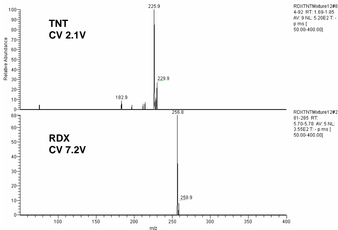
Figure 3-9. Mass spectrum of TNT/RDX mixture. Figure 3-9 shows the mass spectra of the respective CV peaks of TNT and RDX in the mixture (Figure 3-8). Both components (the TNT [M]^- ion at m/z 226 and the RDX [M+Cl]^- ion at m/z 257) are shown. It should be noted that because the same DV was used for both of these mixtures (-2500V), the CV values of RDX and the solvent is identical in the CV spectra of both mixtures. (compare figs. 3-6 and 3-8)
