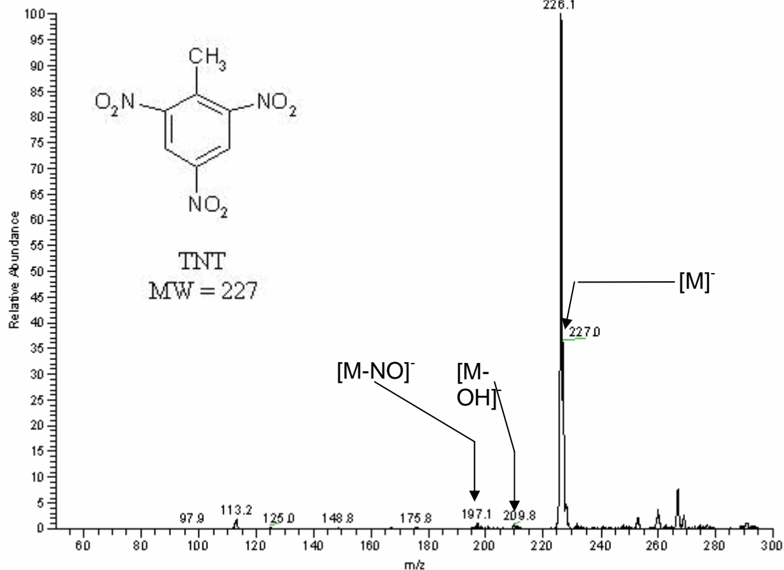
Figure 2-3. Negative ion APCI mass spectrum of TNT. The first spectrum (Figure 2-3) shows negative ion APCI of TNT without FAIMS separation. The [M]^- ion at 227.0 and [M-H]^- ion at 226.1 can be seen clearly, and a small amount of background noise (ions that correspond to minor fragment ions of TNT or impurities) is visible.
