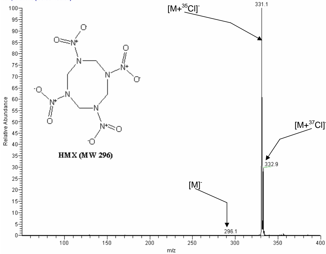
Figure 2-18. FAIMS/MS mass spectrum of HMX. Similar to RDX, the dominant ion for HMX was [M+\text{Cl}]^- . This can be seen in figure 2-18. Once again, adducts of HMX were formed with both dominant isotopes of chloride. There was also evidence of a small amount of [M]^- .
