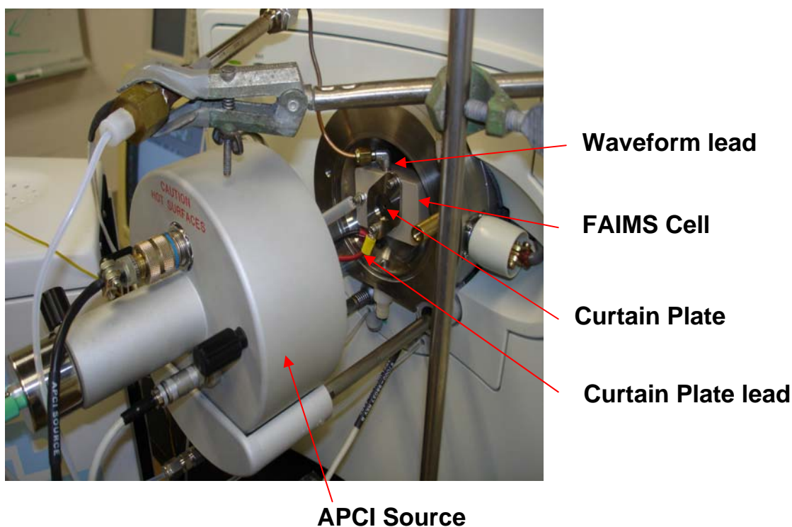
Figure 1-3. APCI source and FAIMS cell mounted on a Finnigan LCQ.
