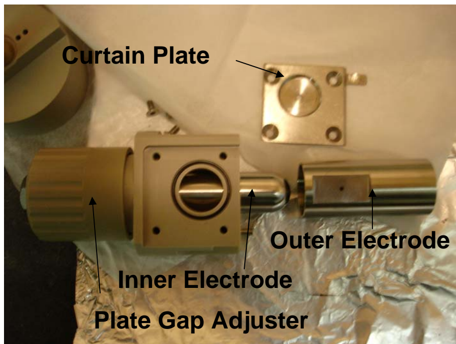
Figure 3-4. Photograph of Ionalytics orthogonal dome FAIMS cell. Figure 3-4 is a photograph of the disassembled orthogonal dome cell used for these experiments. The plate gap adjuster rotates to change the distance between the inner and outer electrodes.
