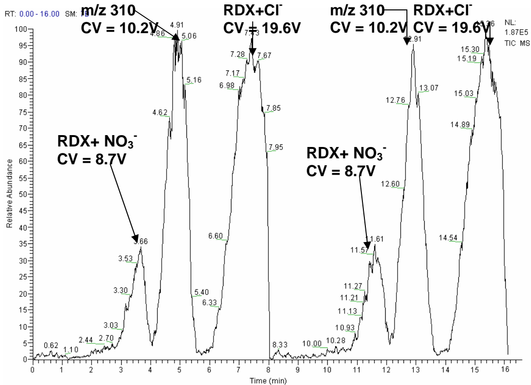
Figure 3-17. RDX CV spectrum at 2.0 mm. The last trial was done with an electrode gap of 2.0 mm (Figure 3-17). If the distance is set too high, as in this case, then the electrodes can no longer carry a waveform. This ion count was the highest of all these trials, presenting three orders of magnitude greater transmission than the smallest setting at 0.5 mm. The RDX peak was robust and well-resolved; however, the peaks at m/z 283 and m/z 310 were again visible.
