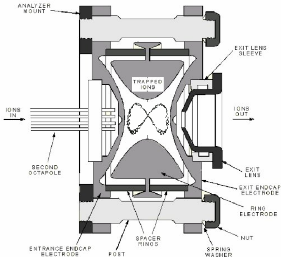
Figure 1-5. LCQ quadrupole ion trap showing ion trajectory. [Adapted from Thermo-Electron Corp. 2003. Finnigan LCQ Series Hardware Manual , Rev. A.]
