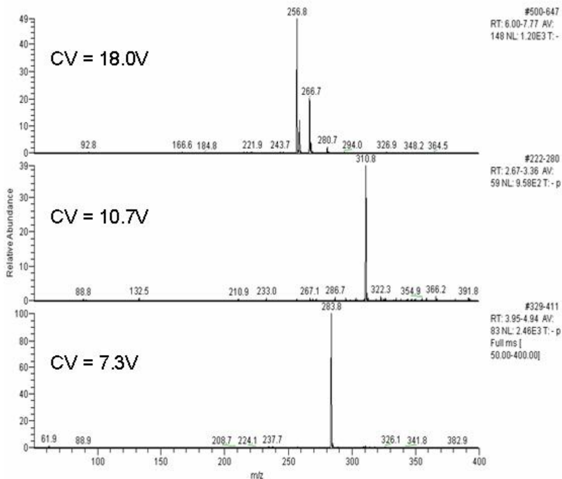
Figure 3-14. RDX mass spectra at 0.5 mm. Figure 3-14 displays the mass spectra corresponding to the three CV peaks in the previous figure. These are similar to those with the smaller electrode distance, as each ion is well resolved.
