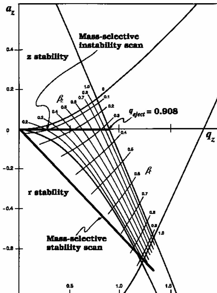
Figure 1-7. Mathieu stability diagram. [Reprinted from McLachlan, N. W. 1947. Theory and Application of Mathieu Functions, Dover].
