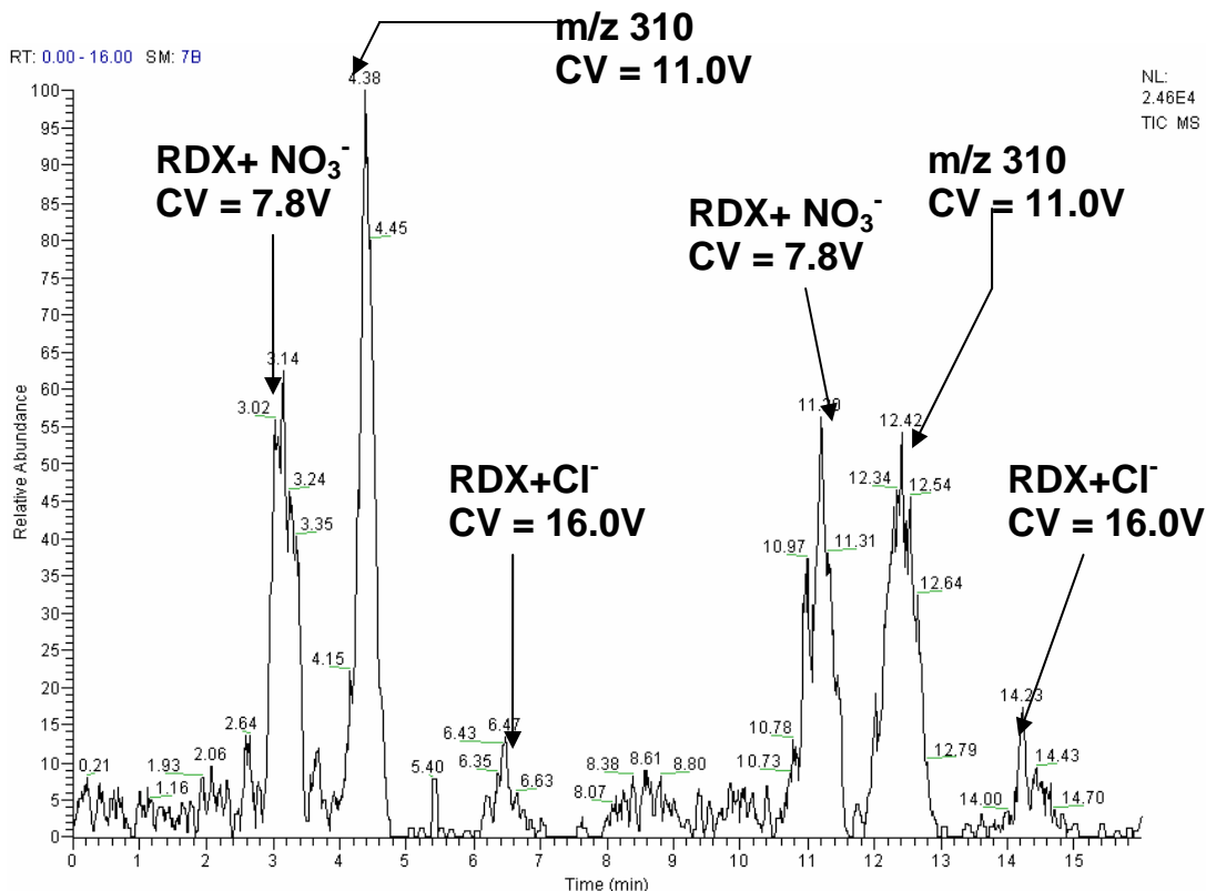
Figure 3-11. RDX CV spectrum at 0.5 mm. The first trial was at a relatively small gap of 0.5 mm (Figure 3-11). The CV was scanned from 0-20V over 8 minutes twice. On the figures, ion count is seen after “NL.” This figure shows three peaks. One of these (m/z 310) is probably a solvent cluster. A second (m/z 283) is the nitrate adduct of RDX. The third (m/z 257) is the RDX chloride adduct. In this case, the RDX analyte of interest is the smallest peak compared to the solvent. Probability of transmission of RDX molecules relative to solvent indicates that when the electrode gap is smallest, most RDX molecules collide with the electrodes and are lost. The maximum ion signal is 2.46 \times 10^4 counts.
