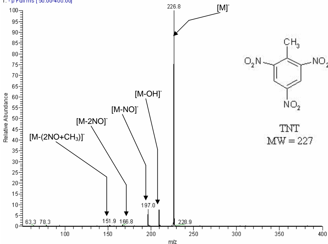
Figure 2-6. FAIMS/APCI mass spectrum of TNT: measured for 2 min at CV = 6.6V Figure 2-6 shows a 2 min spectrum taken at a CV of 6.6V, which is when the most TNT [M] - ion passes through the FAIMS. This spectrum is similar to that in the previous figure; the only difference is that instead of averaging one of the CV peaks, data points were taken for a stationary CV. As a result, this spectrum is improved further from that in figure 2-4.
