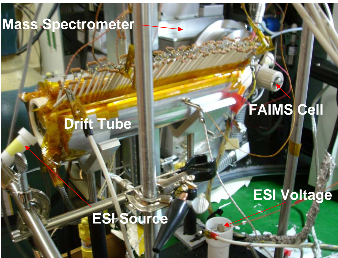
Figure 3-5. WSU apparatus. A photograph of the entire WSU apparatus including ESI source, IMS drift tube, and FAIMS cell can be seen in Figure 3-5. The waveform generator is not connected to the FAIMS cell so that it is easily visible.
