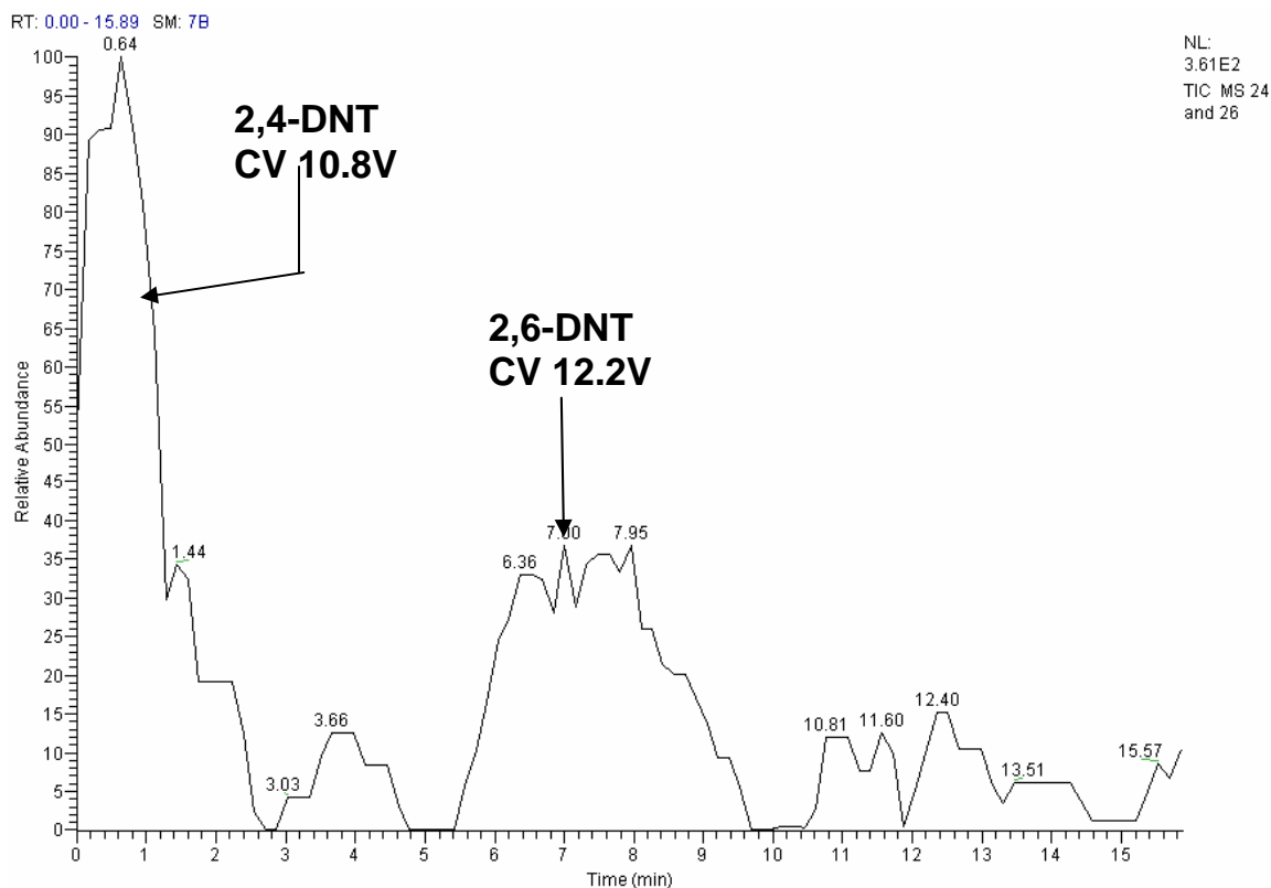
Figure 3-10. CV spectrum of both isomers of DNT. A mixture was created using about 20 ppm of both isomers in equal proportion. This is a relatively small amount, hence the low ion transmission. The CV scan was conducted slowly from only 10-15V over 16 minutes. Both isomers are clearly resolved from each other, as shown in Figure 3-10. It should be noted that there was a [2,6-DNT-NO] - fragment peak that appeared during the characterization (as discussed in Chapter 2, section 2.6). This fragment did not appear while using the high-resolution setup in the 10-15V CV range.
