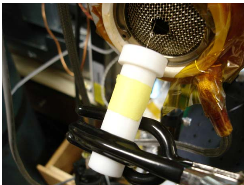
Figure 3-2. WSU electrospray ionization source photograph. Figure 3-2 is a photograph of the WSU ESI source. Note that the tip of the capillary extends through the screen of the IMS. This was done so that the ions would not be deflected backwards by the electric field.
