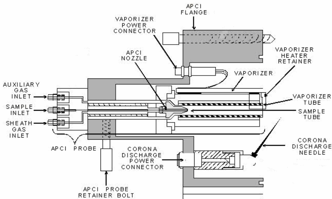
Figure 1-1. Finnigan LCQ APCI source. [Reprinted from Thermo-Electron Corp. 2004. Finnigan LCQ Series APPI/APCI Combination Probe Operator's Manual, Rev. A , Thermo-Electron Corp.]
