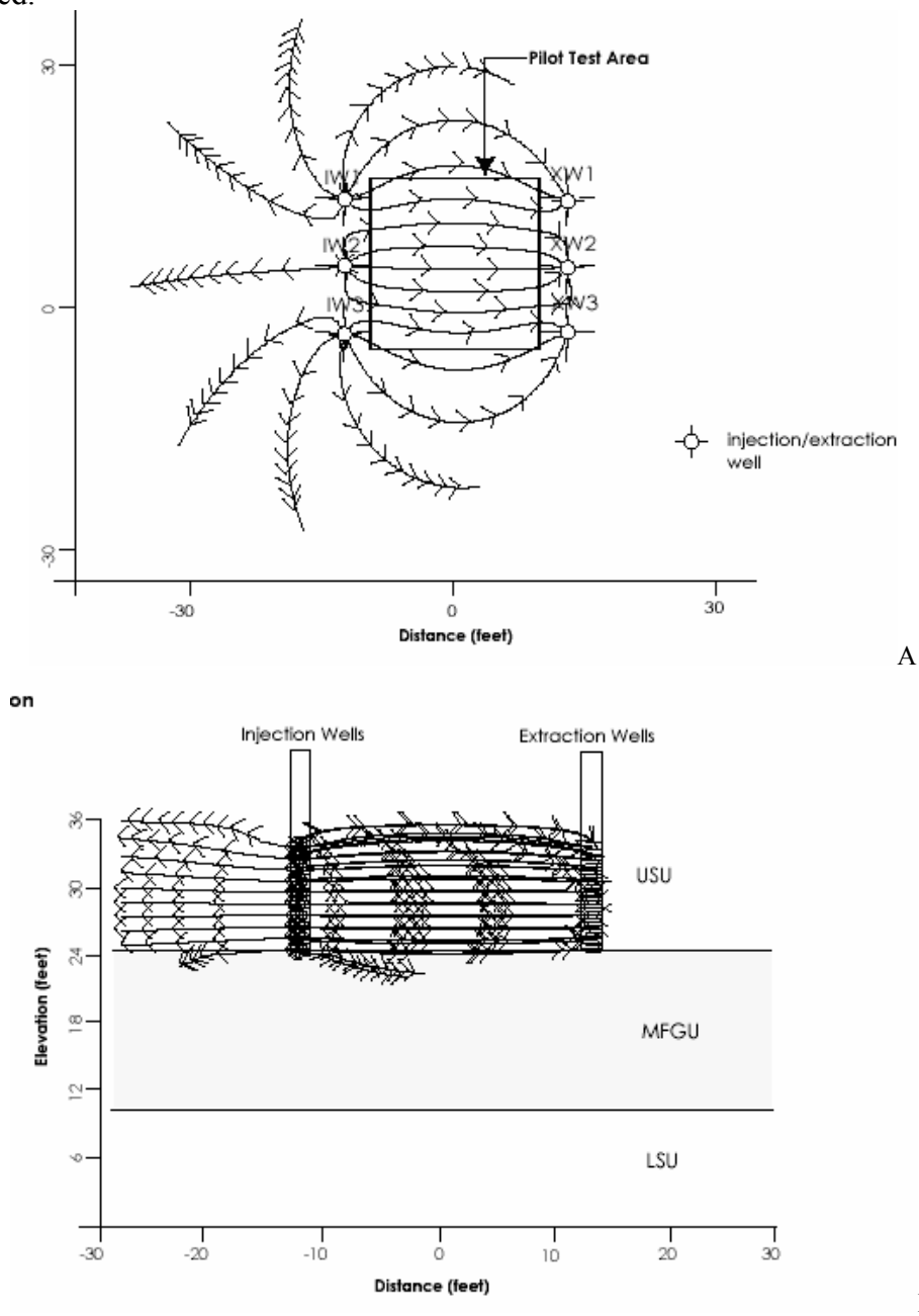
Figure 4-38. Simulated Groundwater Flow at pilot test area (PTA), 0.5 GPM per pump, 1.5 GPM total. A) Plan view. B) Lateral view
