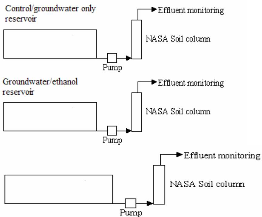
Figure 4-17. Schematic of column setups including control.
