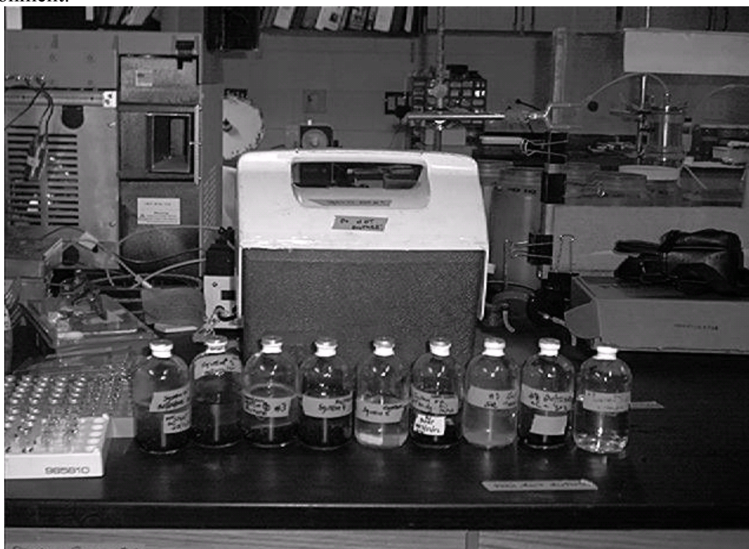
Figure 4-7. Series B oxygen-limited setup, 8 batch systems
