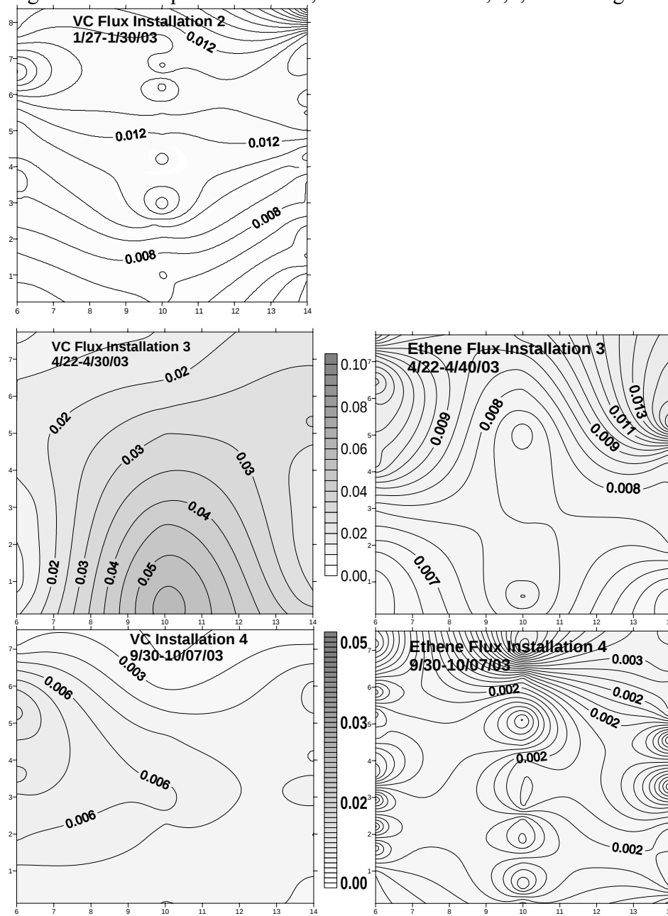
Figure 4-55. Comparison of VC and Ethene contaminant flux for Phase 2,3,4, no vinyl chloride at phase 1, ethene appears at phase 3,4 only. Flux \text{mg}/\text{cm}^2/\text{hr} .
