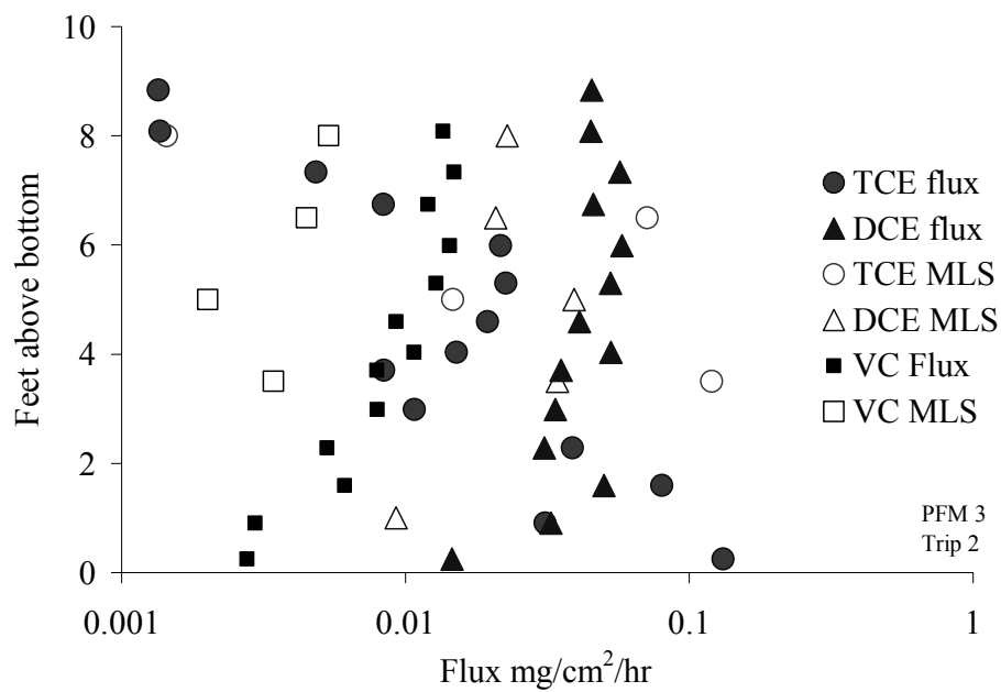
Figure 4-45. Phase 2 PFM#3 TCE, DCE measured PFM Flux, calculate MLS Flux.
