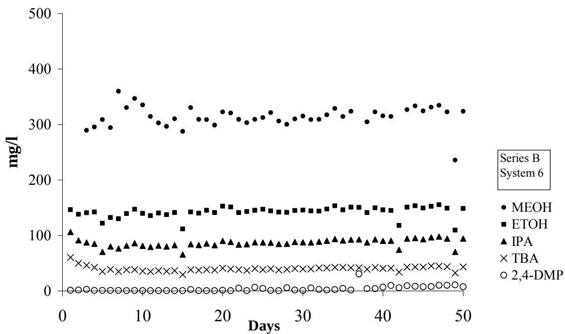
Figure 4-13. Series B System 6: 7.5 g silver AC, 100 g NASA GW, 0.6g NASA soil, 500 \mu l Lact., alcohol spike
