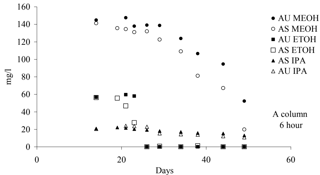
Figure 4-27. 6 hour batch for column A, alcohol concentration
