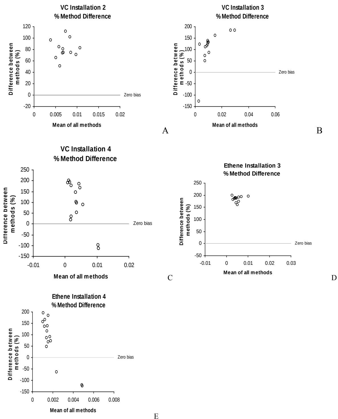
Figure 4-57. Bland Altman VC ethene bias plots using MLS as reference A) VC installation 2. B) VC installation 3. C) VC installation 4. D) Ethene installation 3. E) Ethene installation 4.
