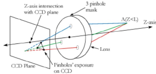
Figure 6. 3-Pinhole DDPIV mask arrangement (Kajitani and Dabiri 2005)
