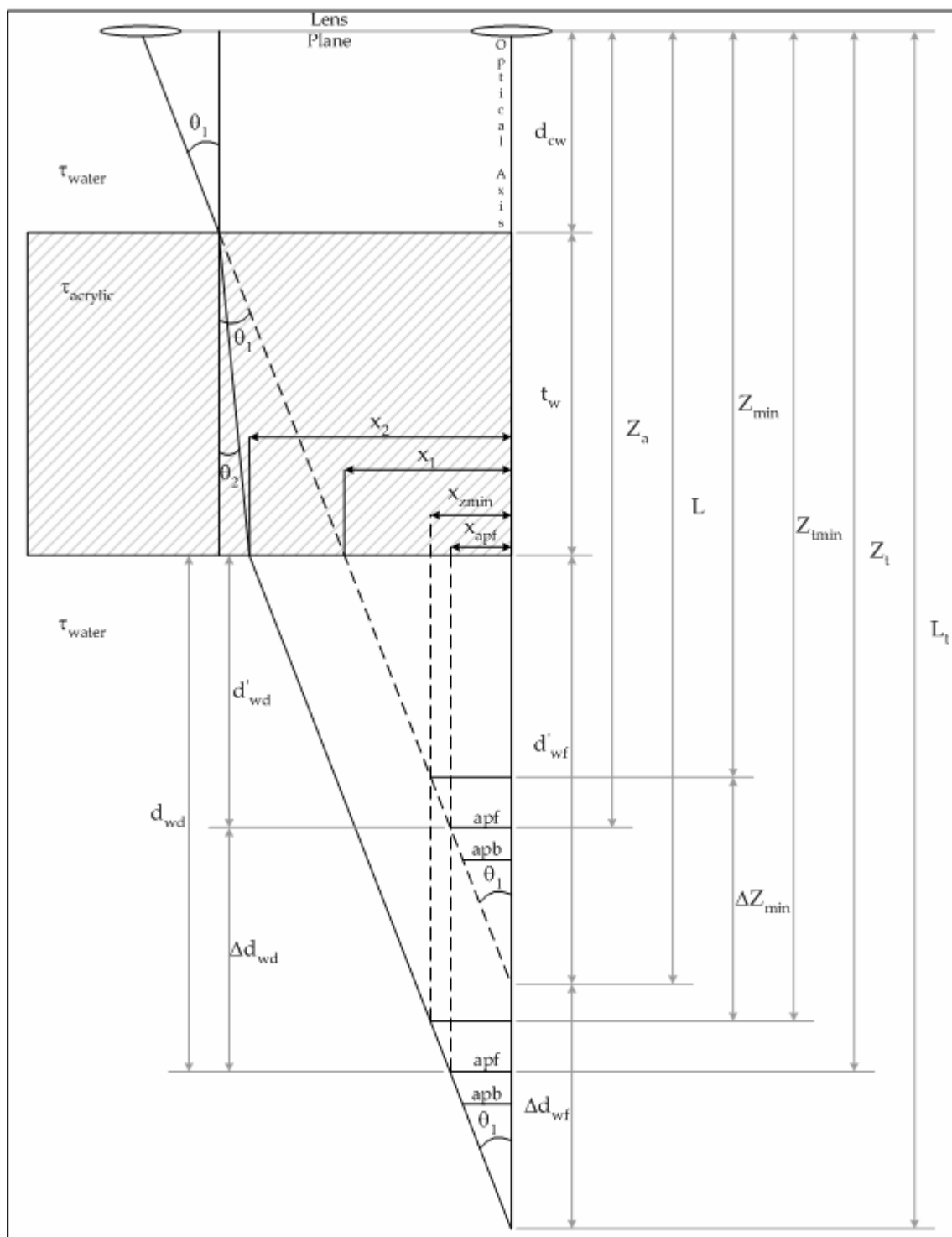
Detailed prism optics schematic
