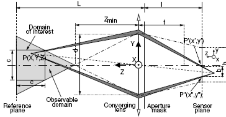
Figure 5. 2-D defocusing geometric model (Pereira and Gharib 2002)
