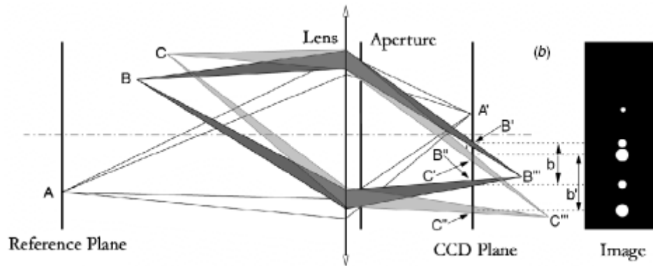
Figure 4. Two-aperture defocused imaging (Kajitani and Dabiri 2005)
