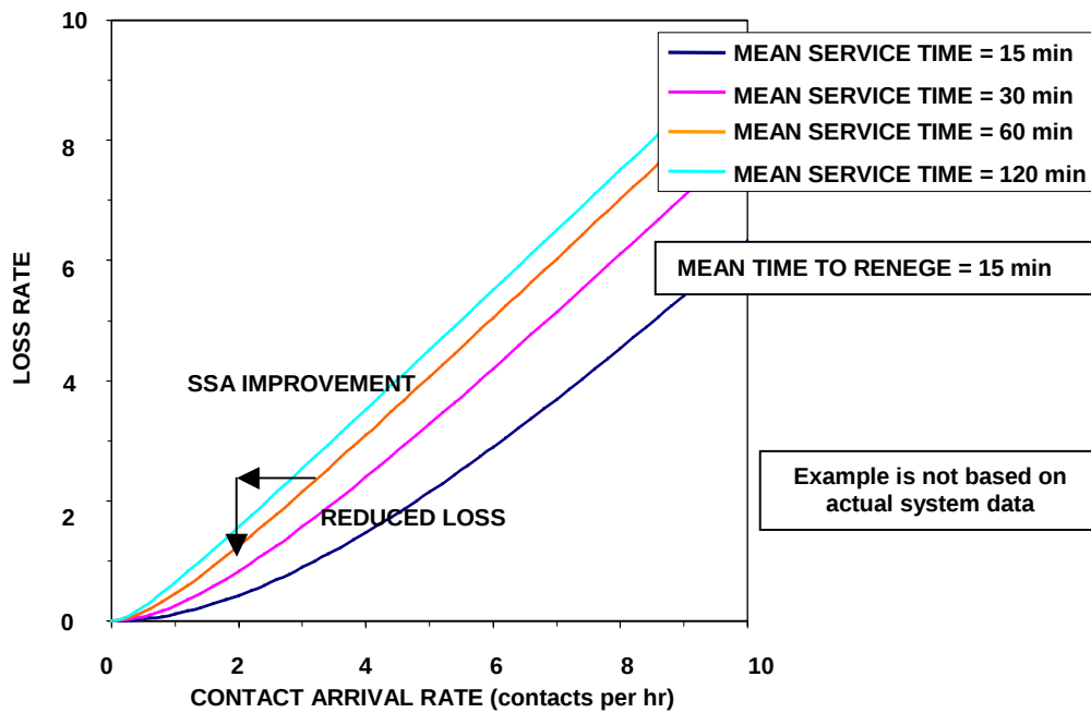
Figure 6: Effect of Improved SSA on Loss Rate, LR
