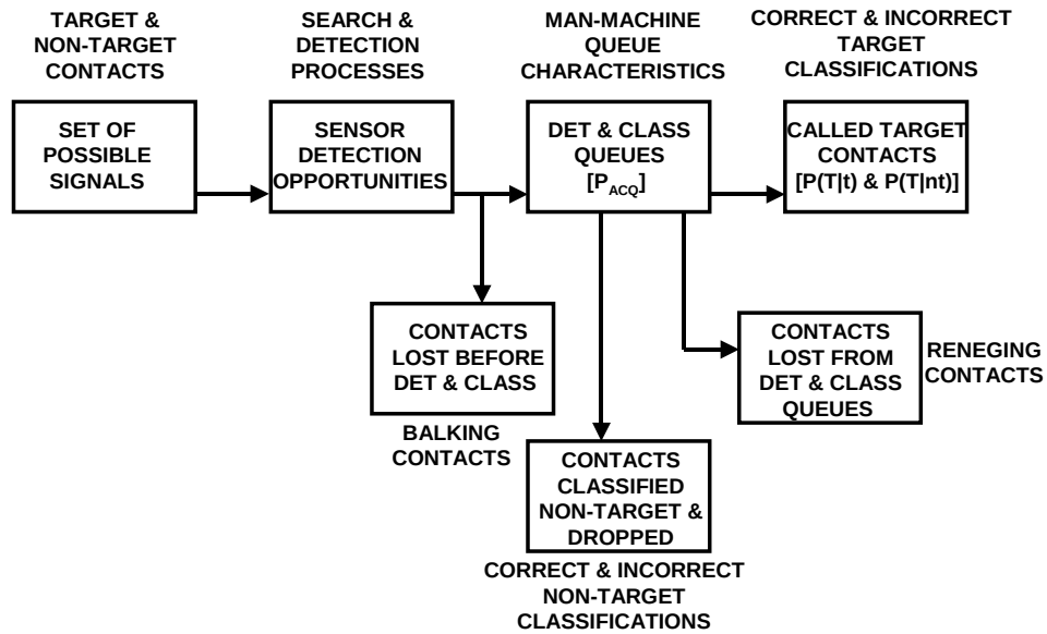
Figure 3: Method to Calculate Probability of Acquisition, P_{ACQ}
