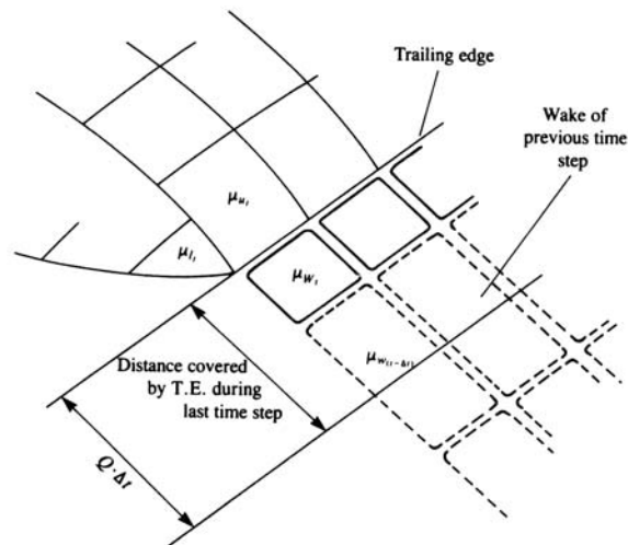
Figure 2: Unstationary free wake vortex (cf. [11])
