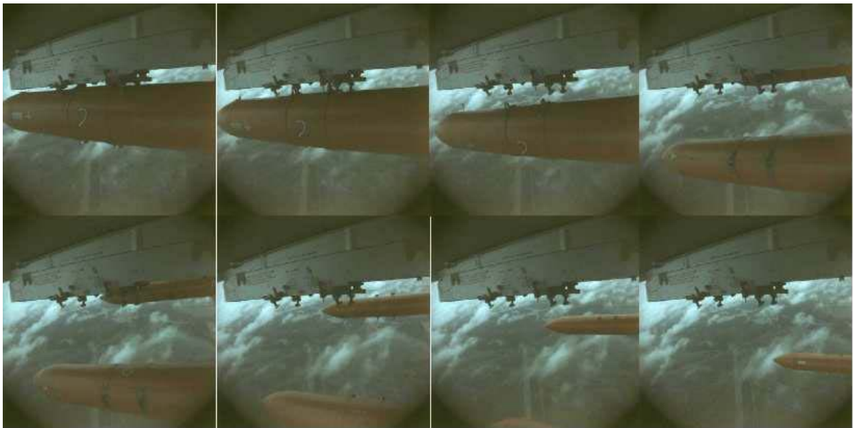
Figure 20: Frame photos of airdrop (on-board high-speed camera)
