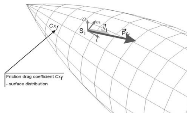
Figure 3: Method of allowing for skin friction drag
