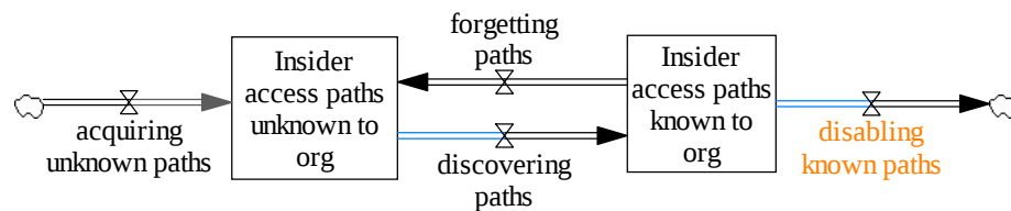
Figure 10: Access Path Stocks and Flows
