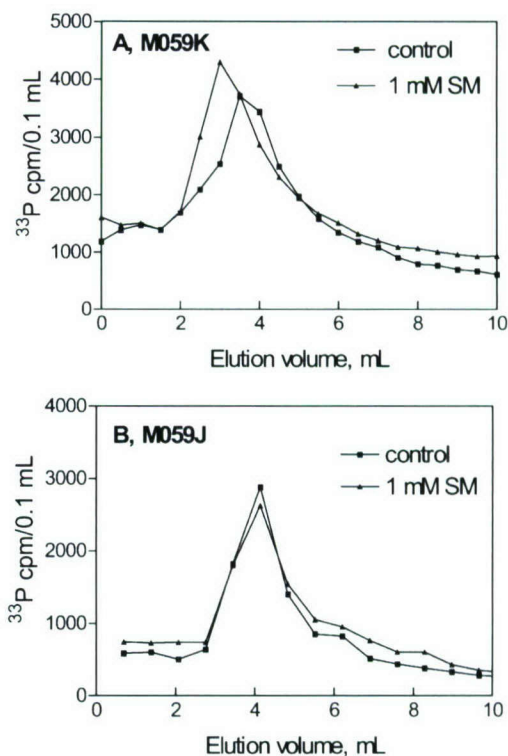
FIGURE 8: Elution profiles from affinity chromatography (DNA ligase I antibody column) of in vivo ^{33}\text{P} -labeled DNA ligase I from M059K (DNA-PK + ) and M059J (DNA-PK - ) cells. (A) M059K; (B) M059J.
