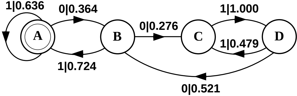
Figure 11 The Misiurewicz machine: the \epsilon -machine reconstructed from a binary sequence of k = 10^7 iterates of the logistic map f(x) = rx(1 - x) at the Misiurewicz parameter value r = r_M \approx 3.9277370017867516 \dots . The symbols 0 and 1 of the measurement alphabet correspond to the left and right halves, respectively, of a binary partition of the unit interval x \in [0, 1] with partition divider at x = 0.5 .
