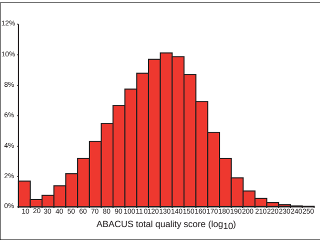
Figure 1 ABACUS quality scores for base calls in B. anthracis . A quality score measures the difference, in log 10 units, between the likelihood support level for the best base-call model minus that for the second-best model [32]. Of the bases, 92.6% possess quality scores that exceeded the threshold (31) used for this study.
