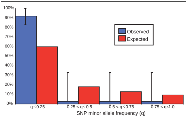
Figure 2 B. anthracis SNP frequency spectrum. An excess of rare SNPs are observed in our sample. Ninety-two percent of the SNPs that we discovered have a minor allele frequency less than or equal to 0.25. This finding (92%) is significantly different from the neutral theory expectation (60%). This excess can arise as a consequence of rapid, population expansion from a small founder population and/or the action of natural selection.
