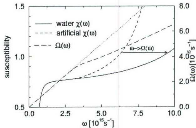
Figure 2 Real water susceptibility and an artificially constructed susceptibility that departs for the real at high frequencies well outside the initial pulse spectral bandwidth.
