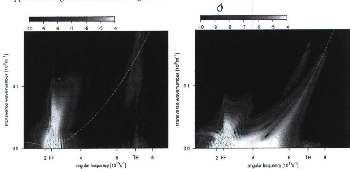
Figure 4 Left: On- and off-axis emission spectra for a tightly focused intense femtosecond pulse in water. The fundamental (FF) and third harmonic (TH) don't overlap spectrally. Right: Strongly admixed FF and TH spectral components due to strong SC generation subsequent to critical collapse in weakly focused geometry.
