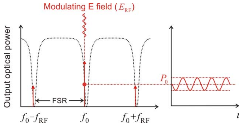
Figure 3 E-O Modulation.
