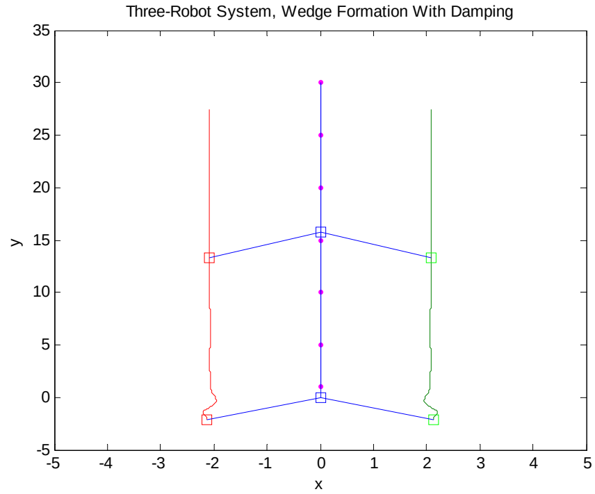
Figure 6-4: Results for a three-robot system with damping in a wedge formation (blue:leader, green:follower 1, red:follower 2).
