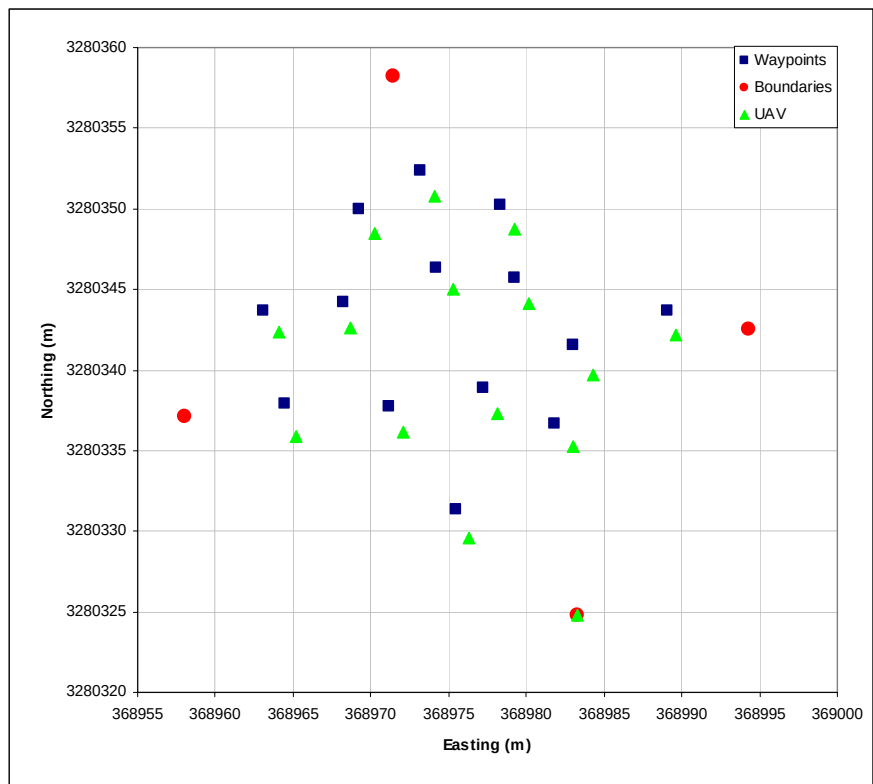
Figure 3-16: UAV vs. differential GPS
