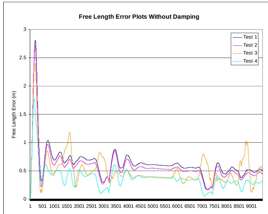
Figure 4-10: Free length error plot comparisons across each test without damping.
