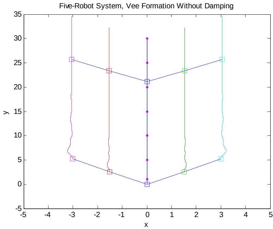
Figure 6-8: Results for a five-robot system in a wedge formation (blue:leader, green:follower 1, red:follower 2, cyan:follower 3, purple:follower 4).
