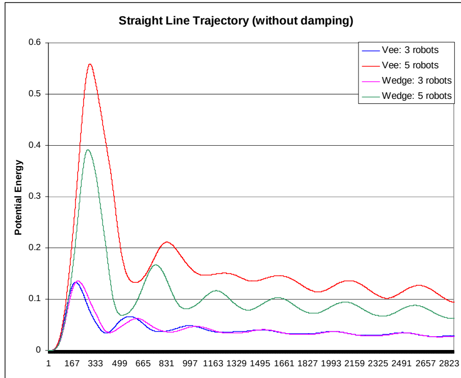
Figure 6-20: Potential energy plots for the straight line trajectory without damping.
