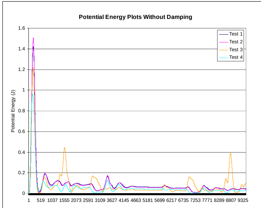
Figure 4-8: Potential energy plot comparisons across each test without damping.
