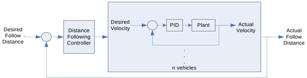
Figure 3-9: Distance following control strategy diagram.
