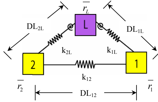
Figure 4-3: Desired and actual vectors and angles for follower robot.
