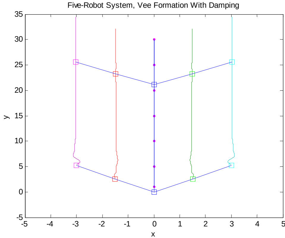
Figure 6-11: Results for a five-robot system with damping in a vee formation (blue:leader, green:follower 1, red:follower 2, cyan:follower 3, purple:follower 4)
