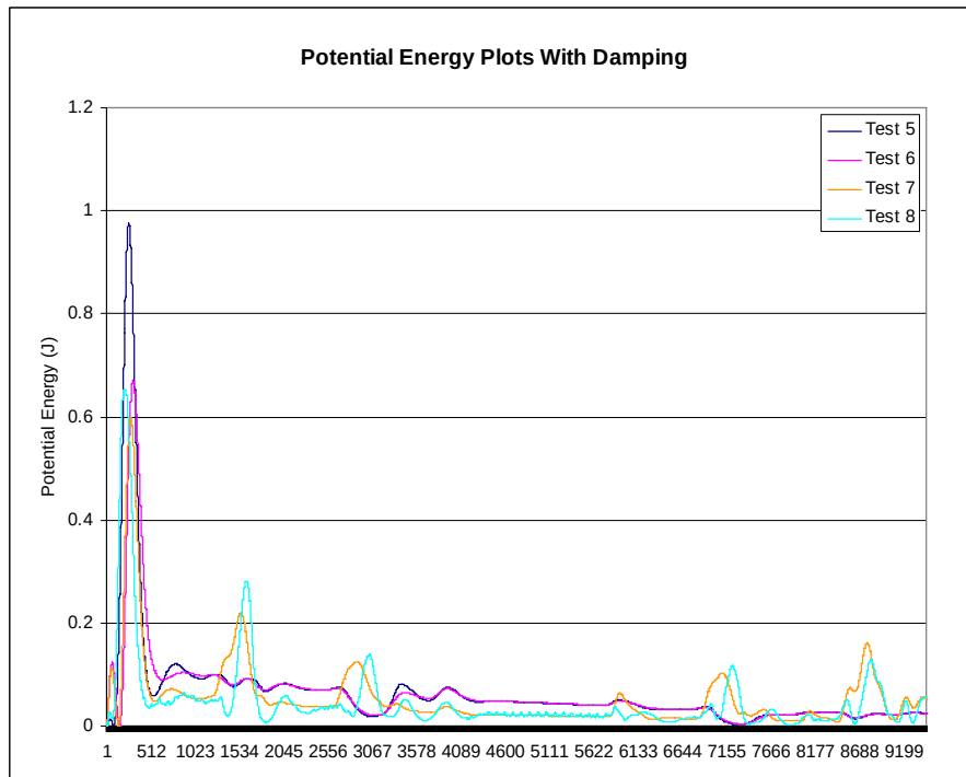
Figure 4-9: Potential energy plot comparisons across each test with damping.
