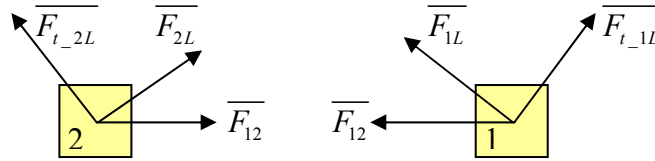
Figure 4-5: Free body diagrams of robot 1 and 2.
