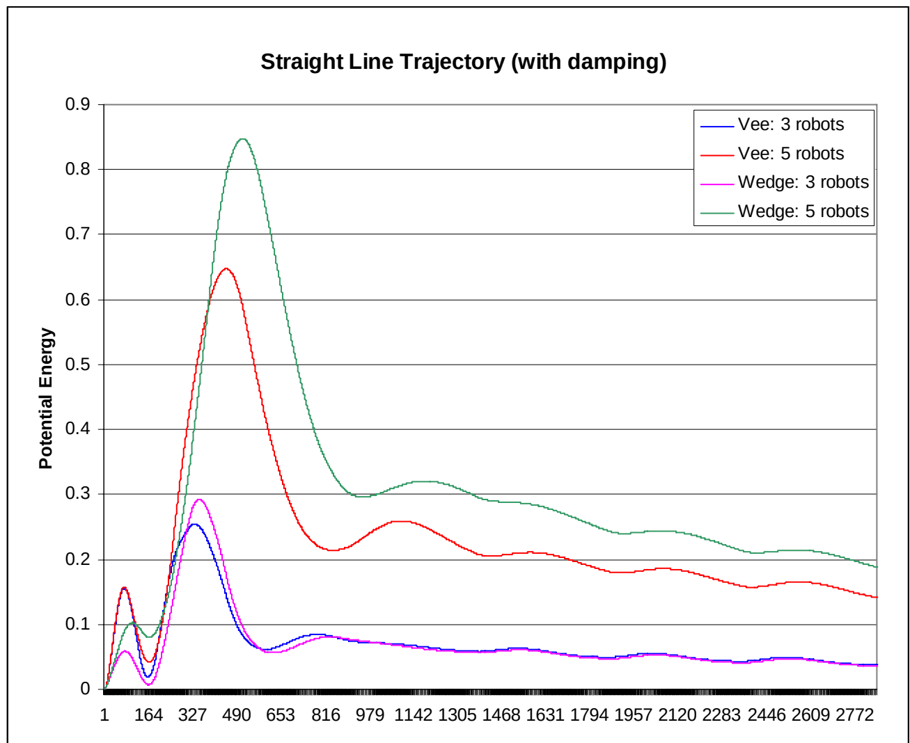
Figure 6-22: Potential energy plots for the straight line trajectory with damping.
