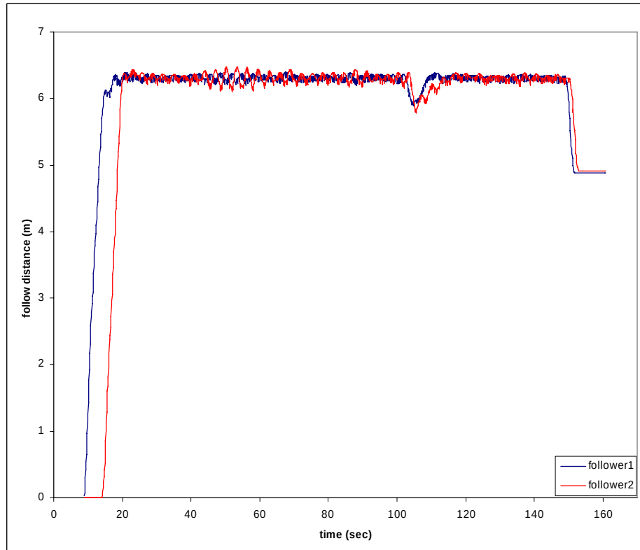
Figure 3-10: Following distances for each vehicle (simulation).
