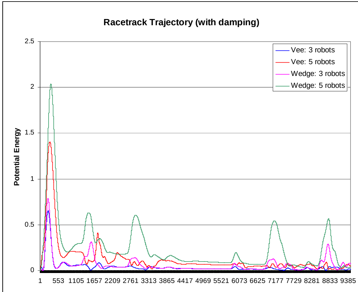
Figure 6-23: Potential energy plots for the racetrack trajectory with damping.
