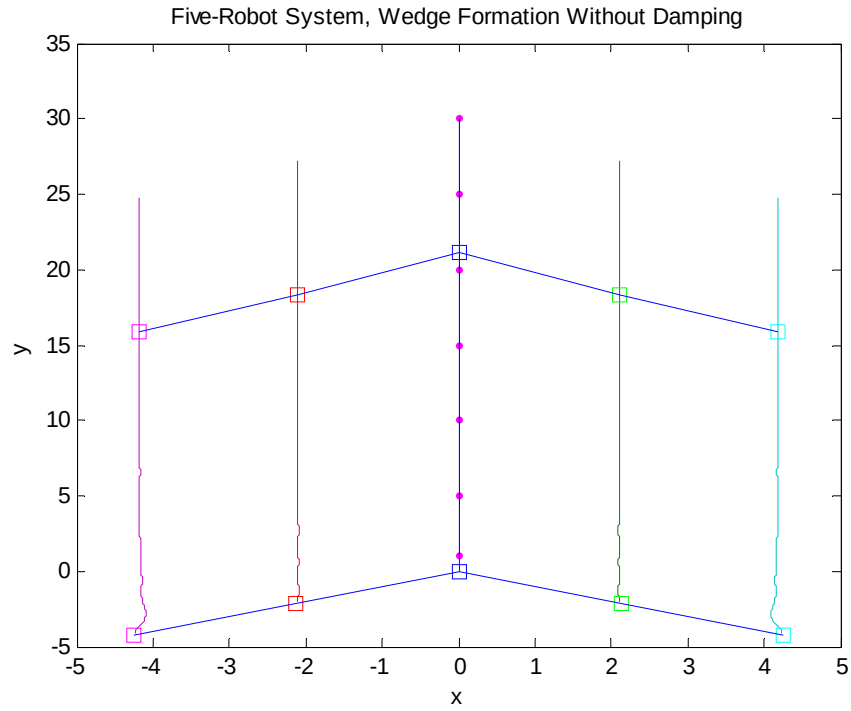
Figure 6-7: Results for a five-robot system in a wedge formation (blue:leader, green:follower 1, red:follower 2, cyan:follower 3, purple:follower 4).
