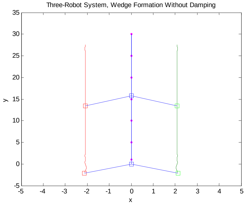
Figure 6-2: Results for a three-robot system in a wedge formation (blue:leader, green:follower 1, red:follower 2).
