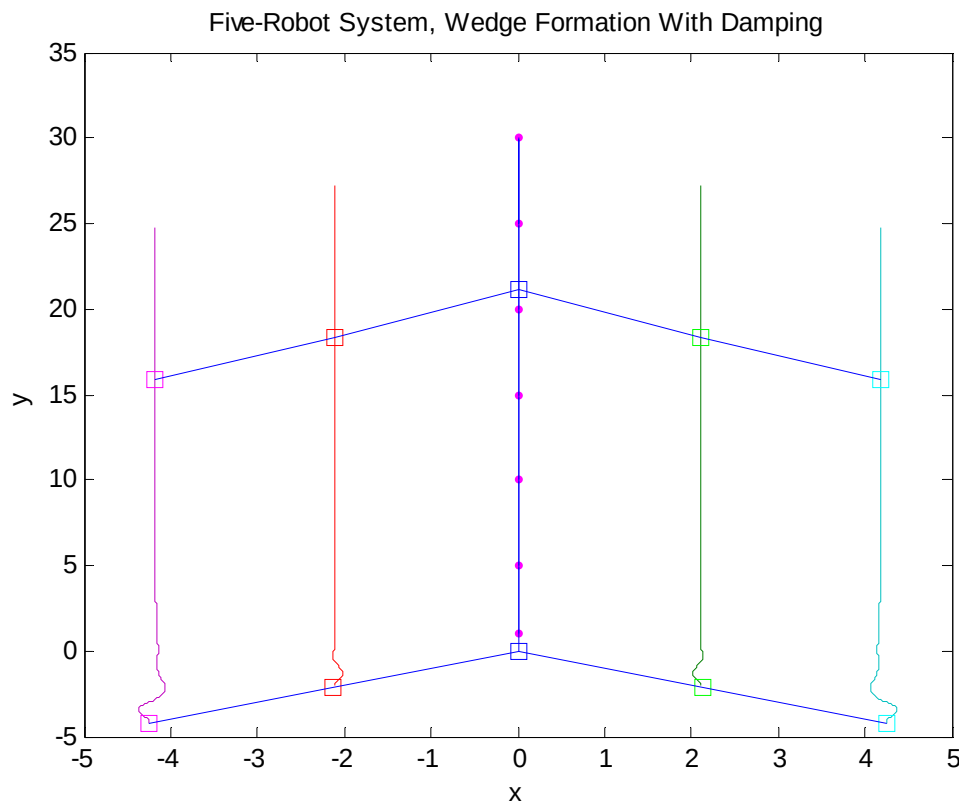
Figure 6-10: Results for a five-robot system with damping in a wedge formation (blue:leader, green:follower 1, red:follower 2, cyan:follower 3, purple:follower 4).
