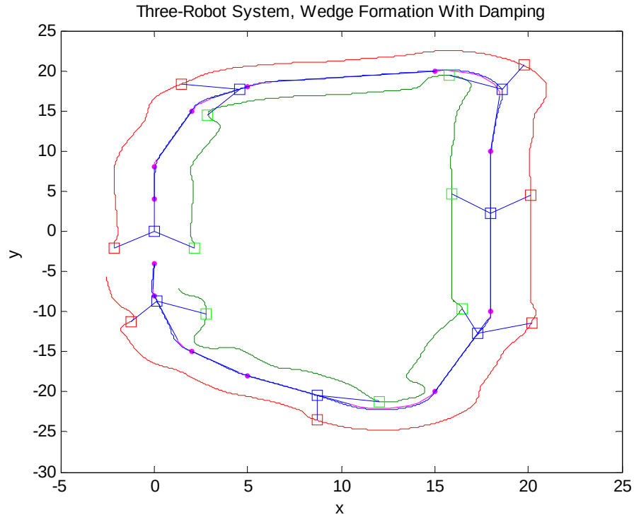
Figure 6-15: Results for a three-robot system with damping in a wedge formation (blue:leader, green:follower 1, red:follower 2).
