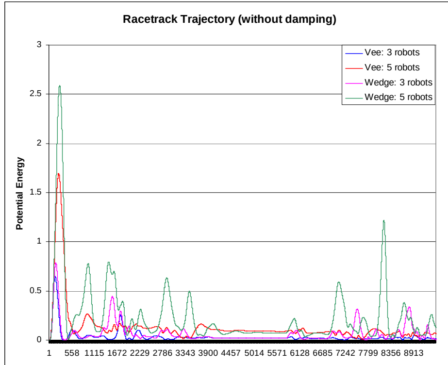
Figure 6-21: Potential energy plots for the racetrack trajectory without damping.
