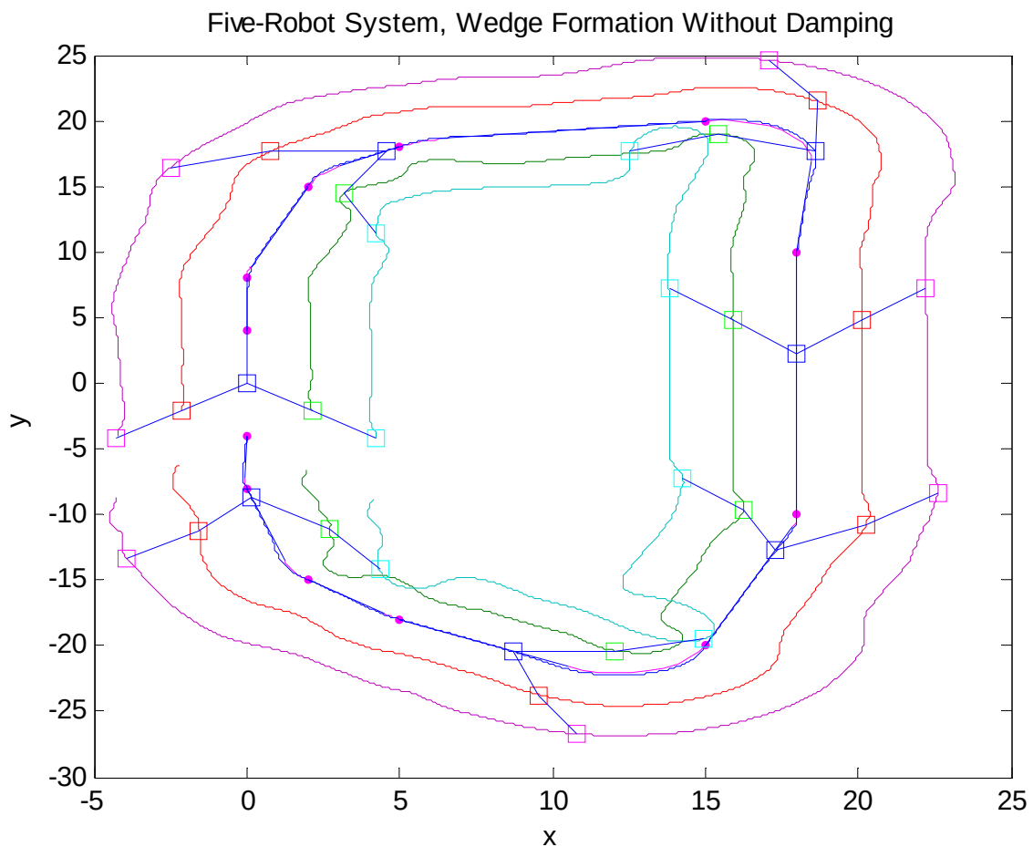
Figure 6-17: Results for a five-robot system in a wedge formation (blue:leader, green:follower 1, red:follower 2, cyan:follower 3, purple:follower 4).
