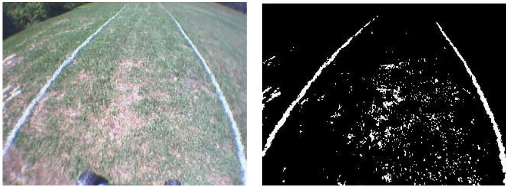
Figure 3-5: Sample image and ML processed image.
