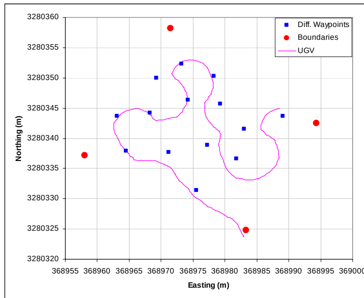
Figure 3-15: A comparison of the UGV's path to the differential waypoints
