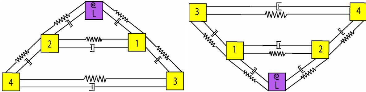
Figure 6-9: Five robots in a wedge and vee formation with damping.
