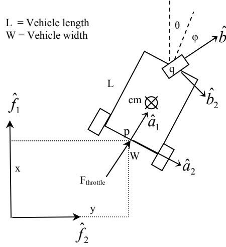
Figure 4-1: Vehicle geometry and coordinate systems.
