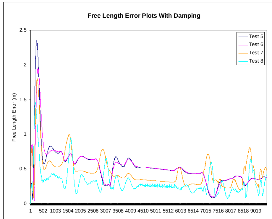
Figure 4-10: Free length error plot comparisons across each test with damping.
