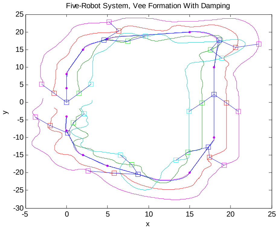
Figure 6-19: Results for a five-robot system with damping in a vee formation (blue:leader, green:follower 1, red:follower 2, cyan:follower 3, purple:follower 4).
