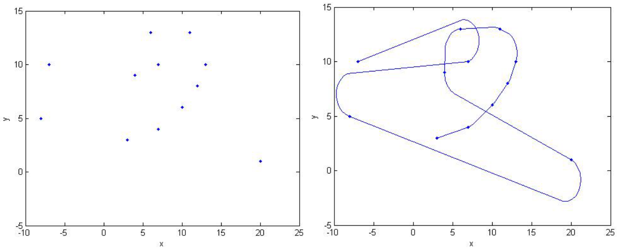
Figure 5-11: A plot of a set of complex waypoints and the corresponding trajectory.
