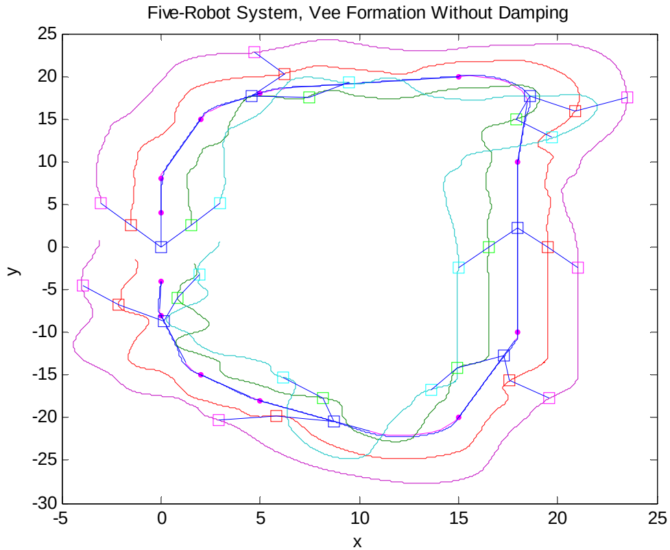
Figure 6-18: Results for a five-robot system in a vee formation (blue:leader, green:follower 1, red:follower 2, cyan:follower 3, purple:follower 4).
