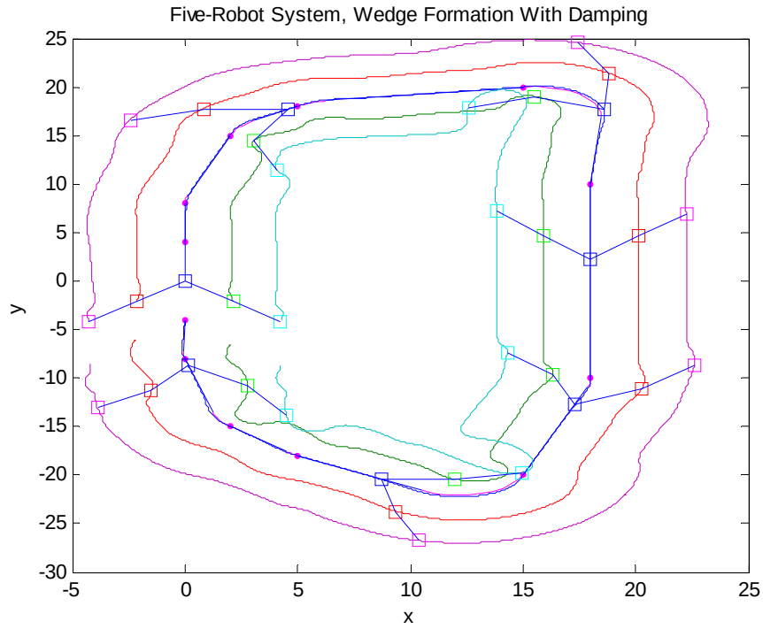
Figure 6-19: Results for a five-robot system with damping in a wedge formation (blue:leader, green:follower 1, red:follower 2, cyan:follower 3, purple:follower 4).
