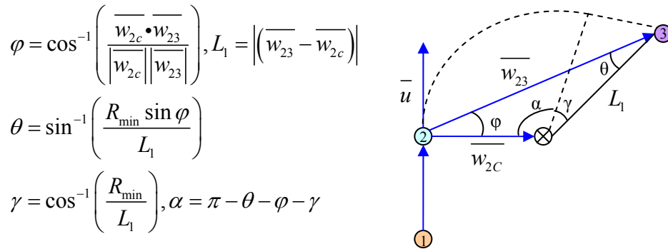
Figure 5-9: Vectors and angles required to determine the sweep angle.
