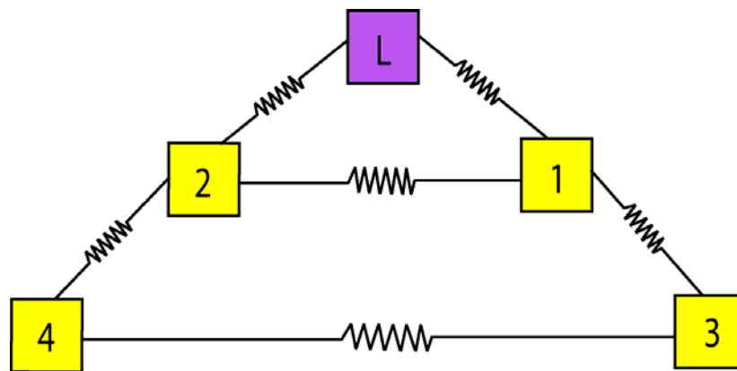
Figure 6-6: Five robots in a wedge formation.
