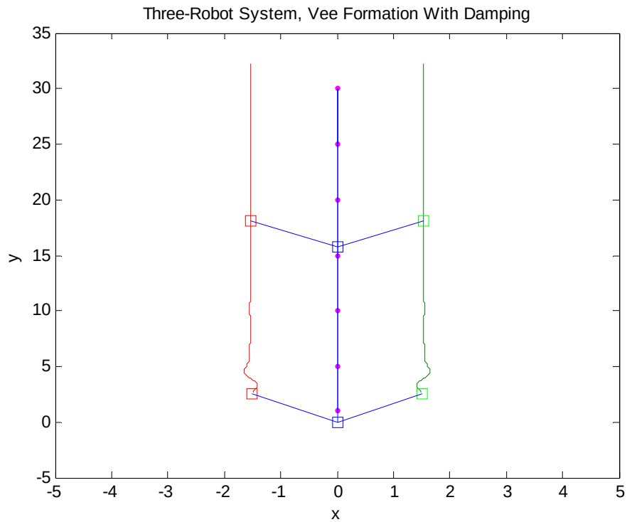
Figure 6-5: Results for a three-robot system with damping in a vee formation (blue:leader, green:follower 1, red:follower 2).
