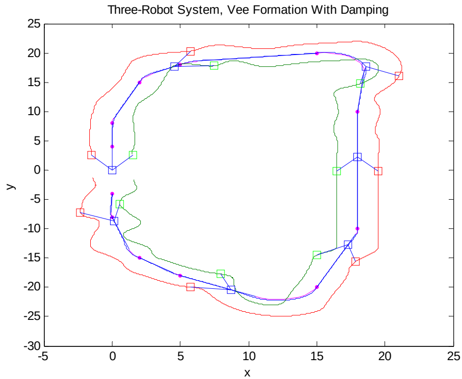
Figure 6-16: Results for a three-robot system with damping in a vee formation (blue:leader, green:follower 1, red:follower 2).
