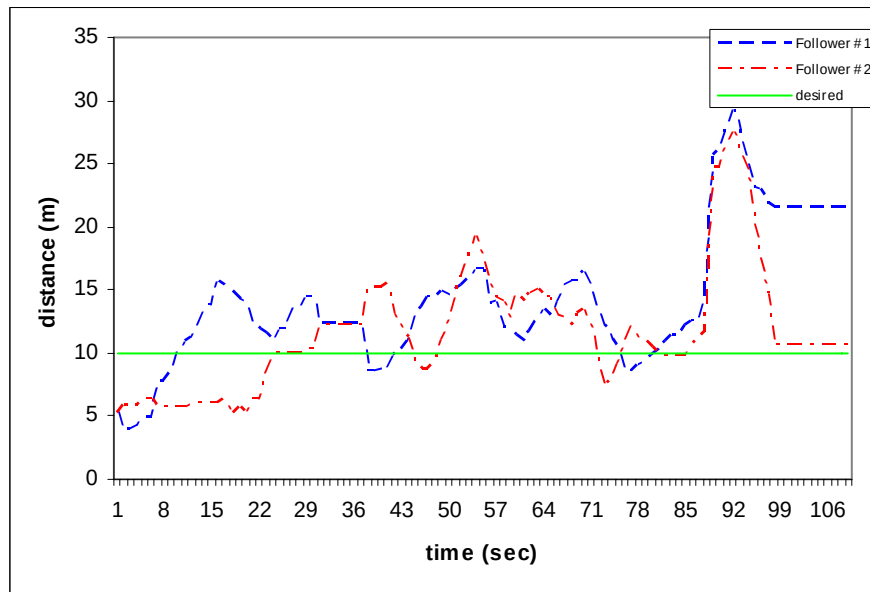
Figure 3-11: Vehicle follow distance on an actual system.
