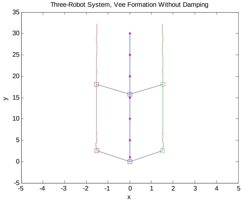
Figure 6-3: Results for a three-robot system in a vee formation (blue:leader, green:follower 1, red:follower 2).
