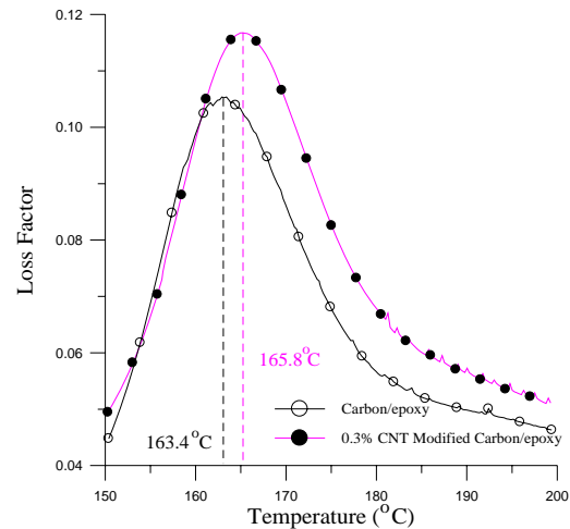
Figure 10 Loss factor vs. temperature curves of neat and nanophased carbon/epoxy composite
