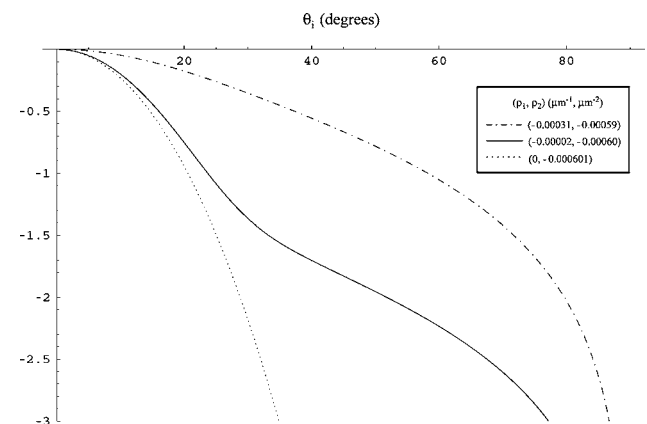
Fig. 7. Derived monostatic radiant intensities due to three surfaces with the same autocorrelation lower bound and \sigma_h = 7 \mu\text{m} illuminated with \bar{\lambda} = 0.6328 \mu\text{m} . The logarithms of the derived radiant intensities are plotted following independent normalizations.
