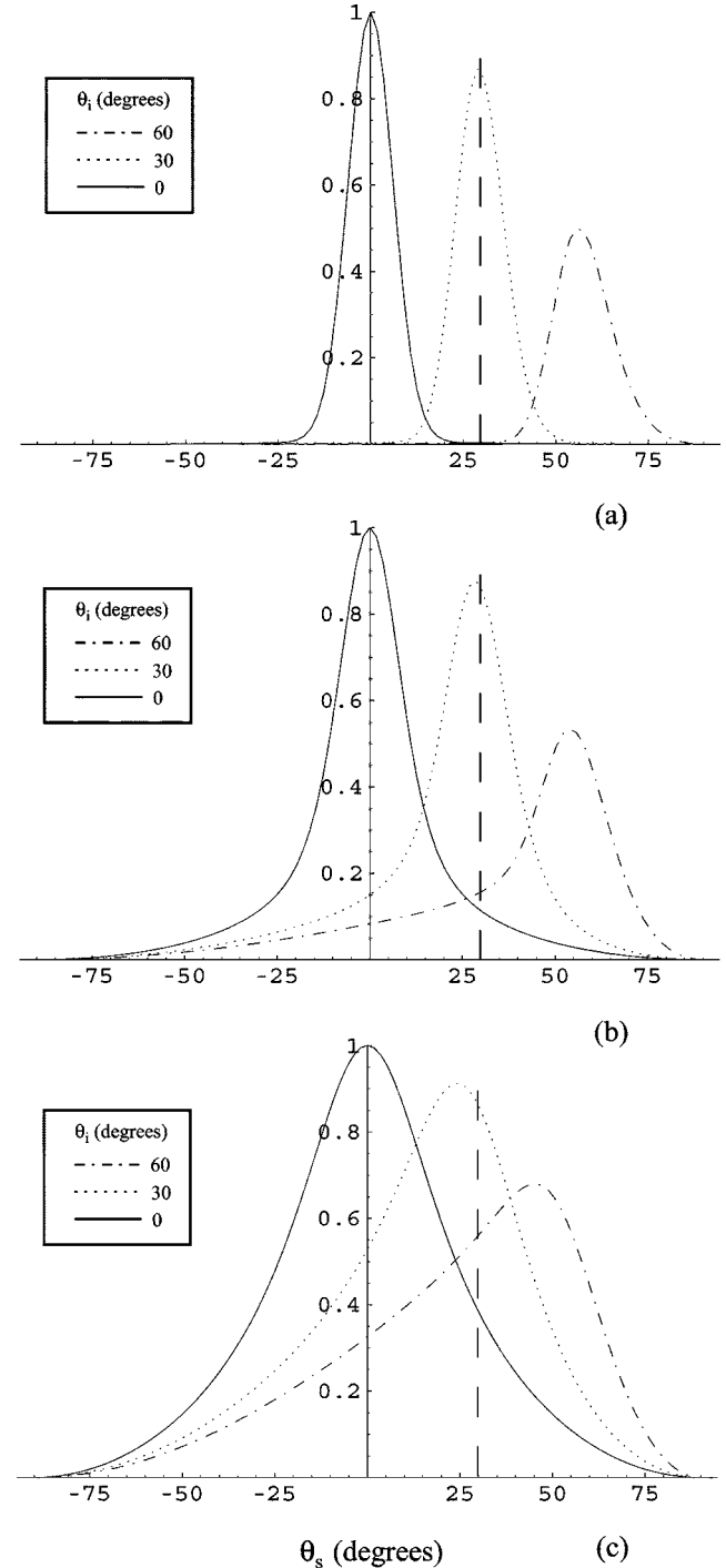
Fig. 5. Variation with incident angle \theta_i of the general solution for the radiant intensity in the specular plane due to (a) a Gaussian-like ( \rho_1=-0.0001 \mu\text{m}^{-1} ), (b) an intermediate ( \rho_1=-0.005 \mu\text{m}^{-1} ), and (c) a Cauchy-like ( \rho_1=-0.02 \mu\text{m}^{-1} ) surface. The units on the vertical axes are normalized across the plots, and \rho_2=-0.005 \mu\text{m}^{-2} , \sigma_h=0.75 \mu\text{m} , and \bar{\lambda}=1 \mu\text{m} are fixed. The vertical dashed lines mark the specular direction for \theta_i=30^\circ .
