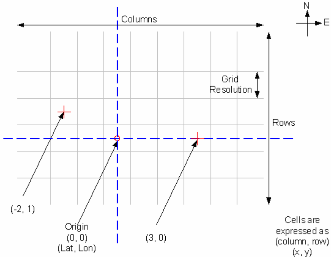
Figure 4-1. Definition of raster grid parameters and coordinate system
