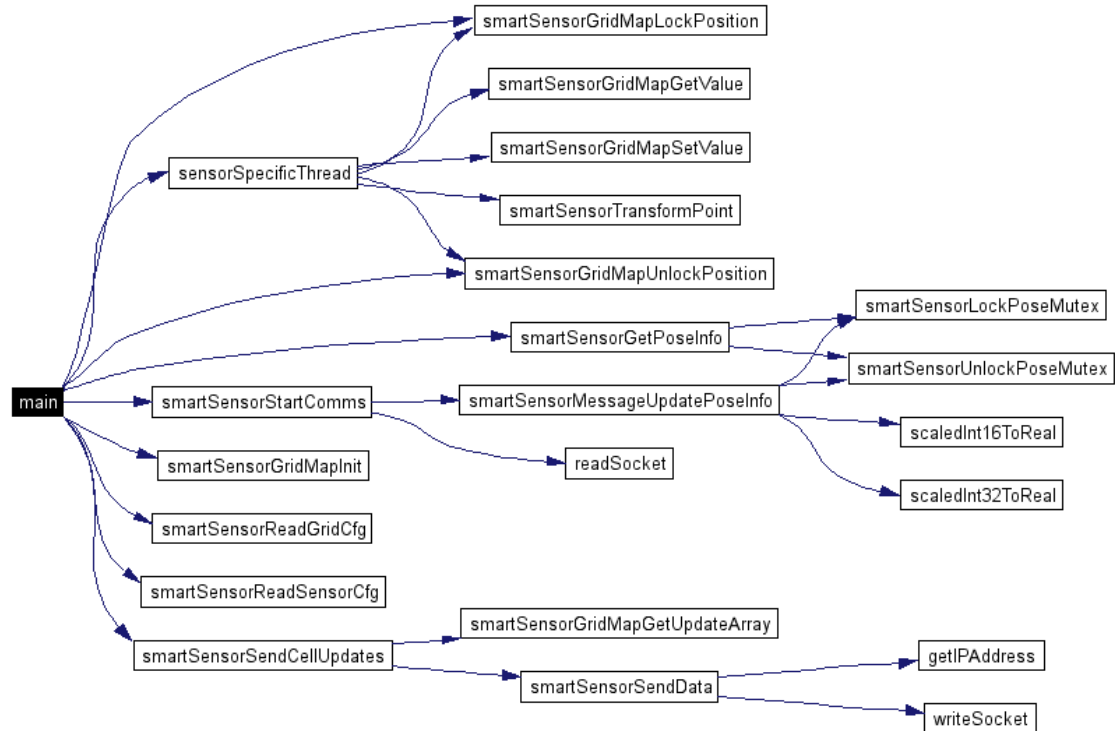
Figure 3-8. Call graph for all functions within the base smart sensor API.
