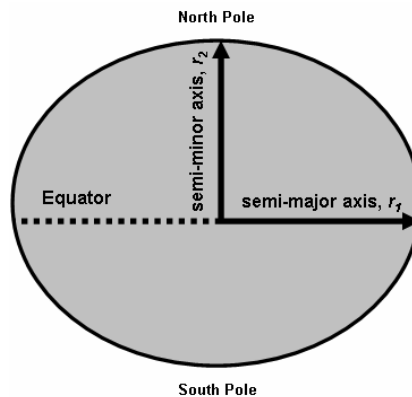
Figure 2-3. Ellipsoidal model of Earth
