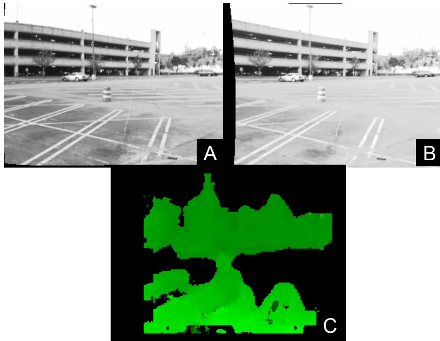
Figure 3-14: Source data and results from stereo correlation. A) Left image. B) Right image. C) Disparity image.
