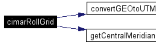
Figure 3-10. Call graph for function that determines number of rows and columns to shift the traversability grid based on the current and previous positions
