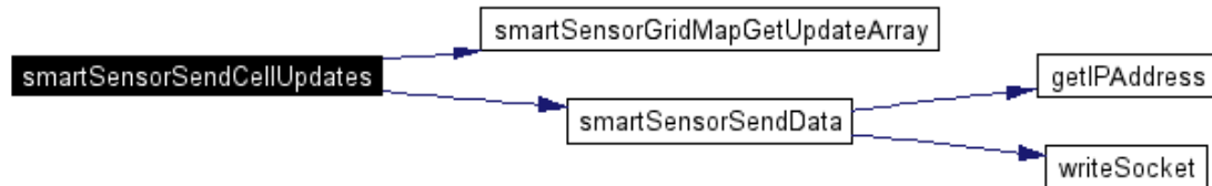
Figure 3-12. Call graph for function used to detect changes in the traversability grid and transmit these changes to the smart sensor arbiter
