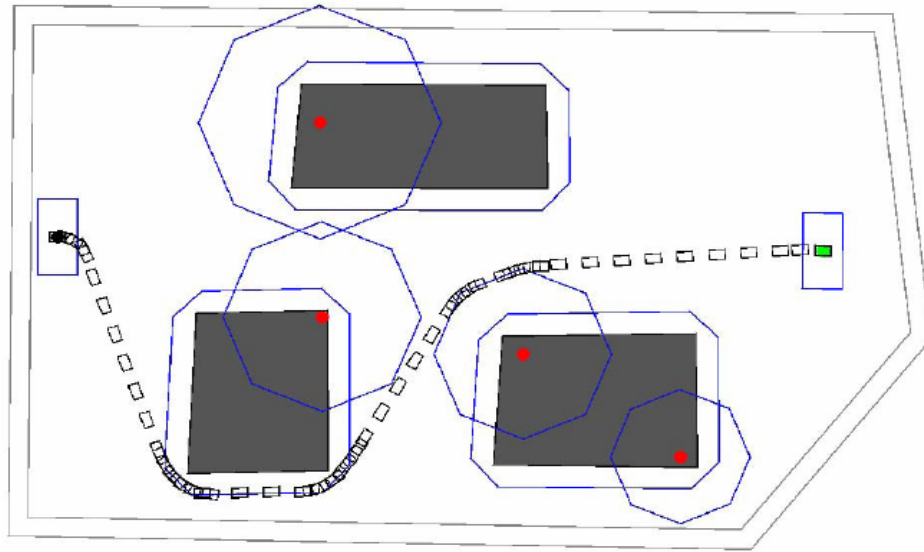
Figure 2-2. Path planning in a bounded radiation environment (Source: A. Pasha, "Path Planning for Nonholonomic Vehicles and Its Application to Radiation Environments," Master of Science Thesis. Department of Mechanical Engineering: University of Florida, 2003, p. 59, Figure 6-9)
