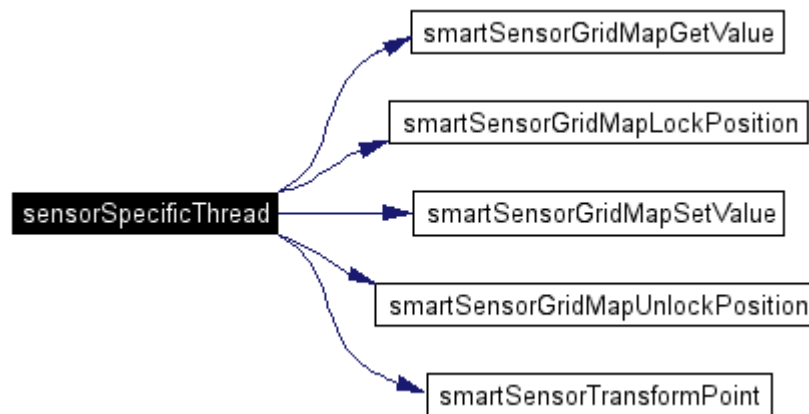
Figure 3-11. Call graph for sensor specific interface thread.
