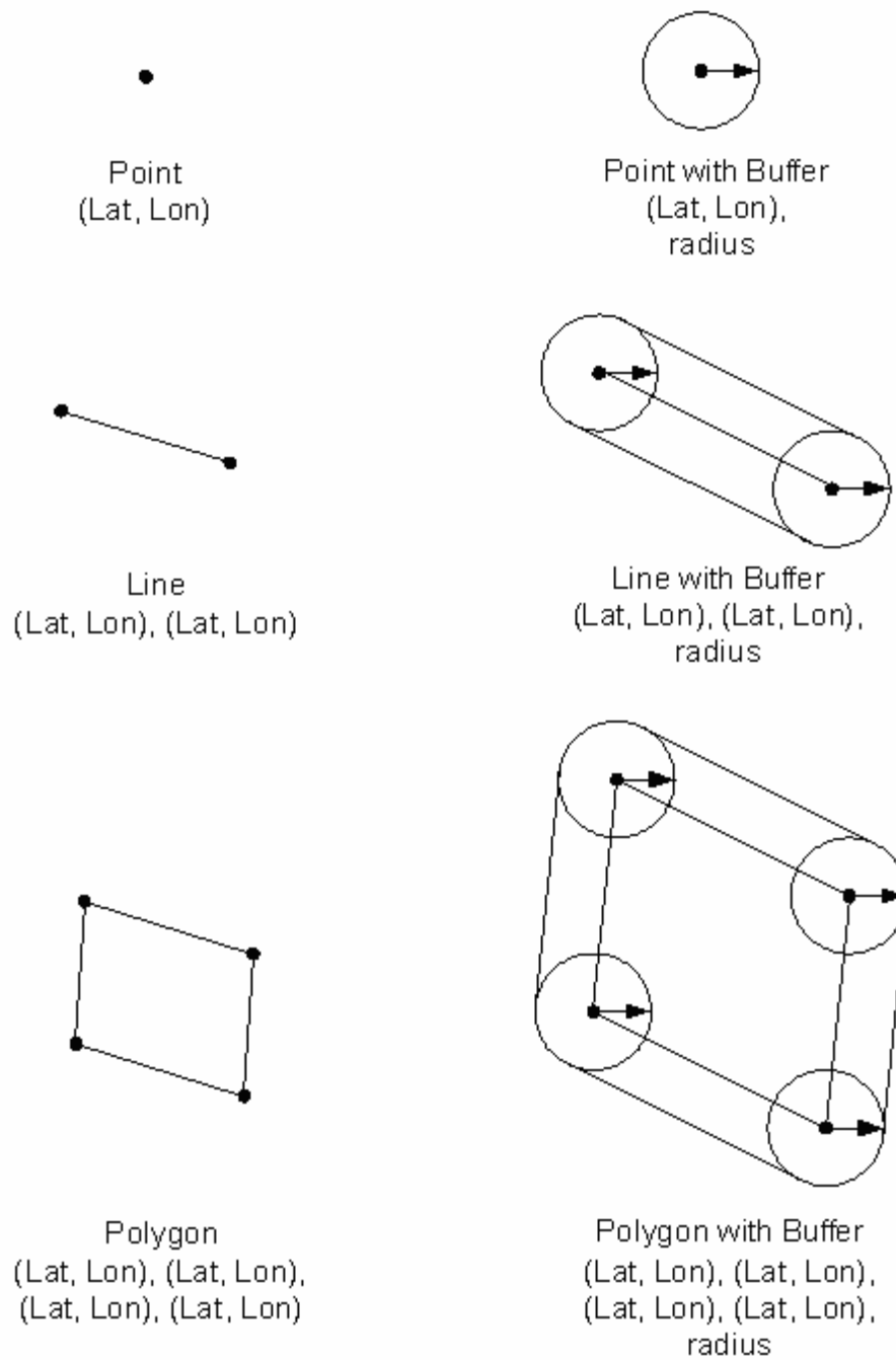
Figure 4-2. Definition of vector objects and parameters
