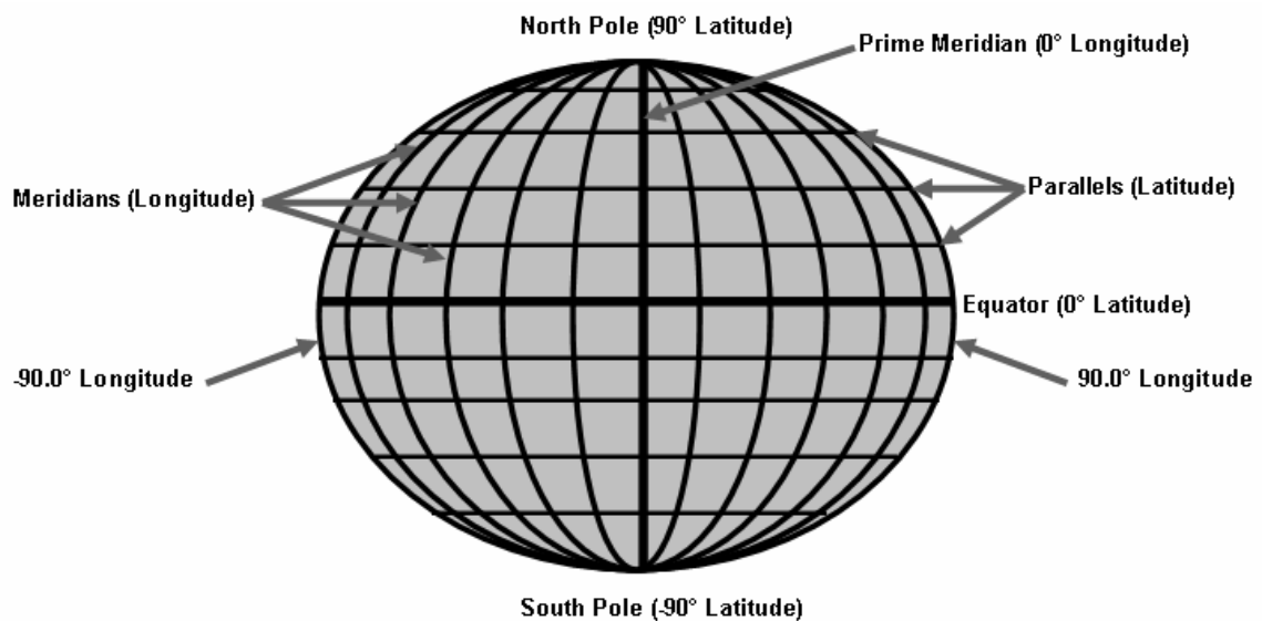
Figure 2-4. Earth-centered global coordinate system
