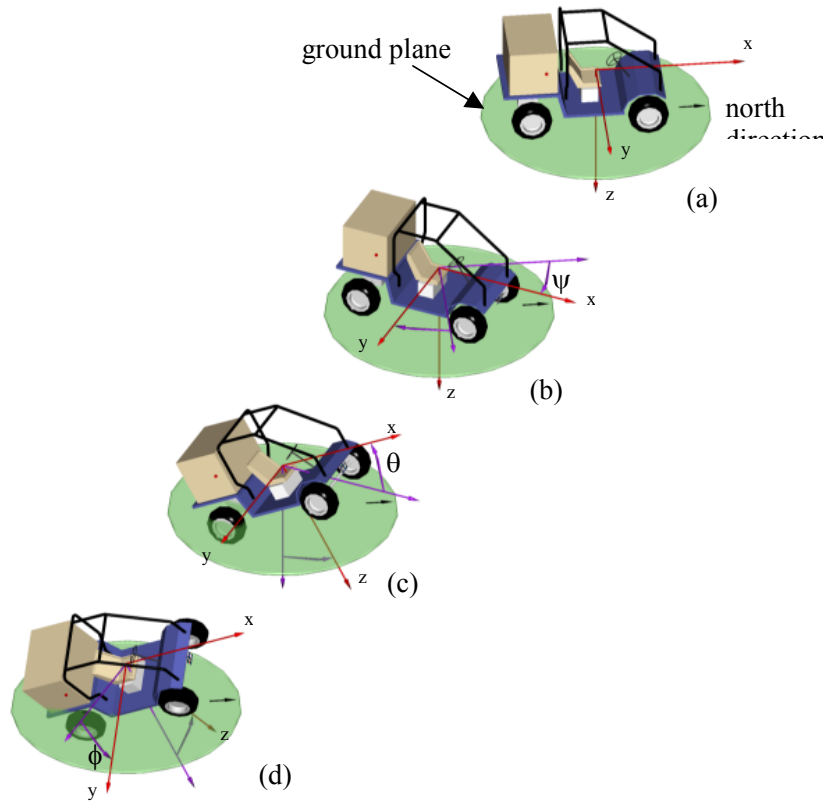
Figure 3-5. Unmanned system coordinate system defined by JAUS
