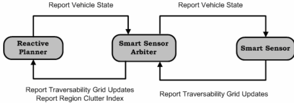
Figure 3-3. Minimally complete smart sensor-based perception system consisting of one instance of the core component.
