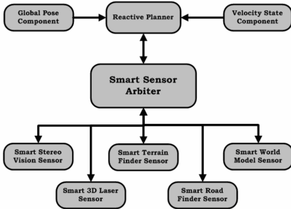
Figure 3-2. Organization of the smart sensor-based perception system
