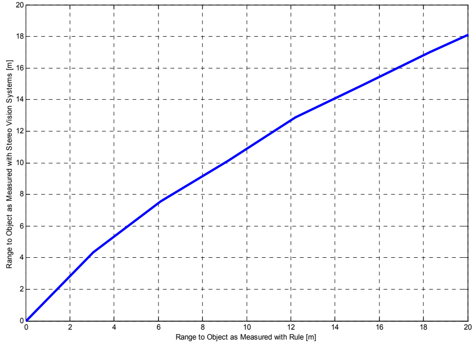
Figure 3-15. Graph of range determined from stereo vision system vs. actual measured range
