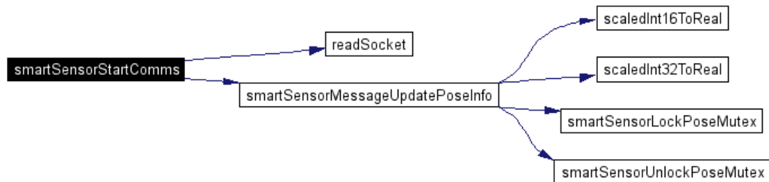
Figure 3-9. Call graph for smart sensor communications receive thread
