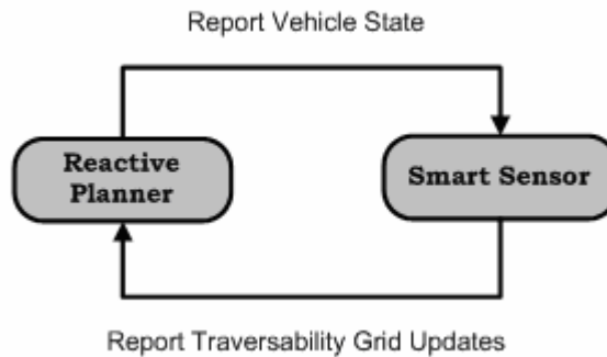
Figure 3-4. Single sensor implementation of smart sensor-based perception system consisting of a single smart sensor synchronizing data with the reactive planner.
