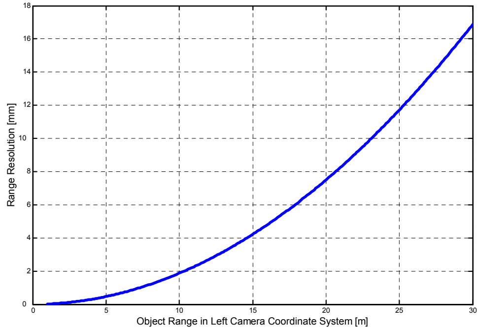
Figure 3-16. Plot of range resolution vs. range for the Videre Design STH-MD1-C with 12.5mm focal length lenses
