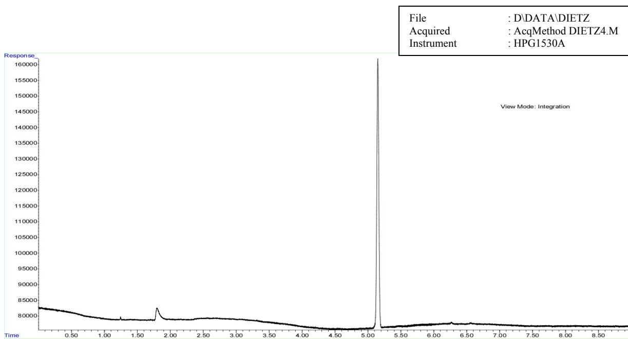
Figure C.6 Sample TAME Chromatograph
