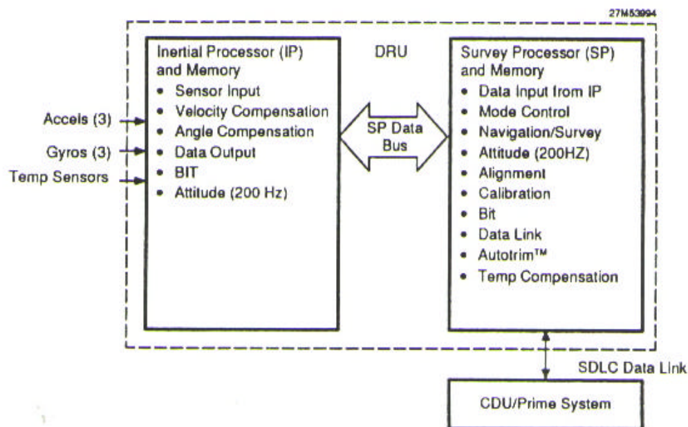
Figure 3.6: Inertial Processor (IP) and Survey Processor (SP) Commands.
