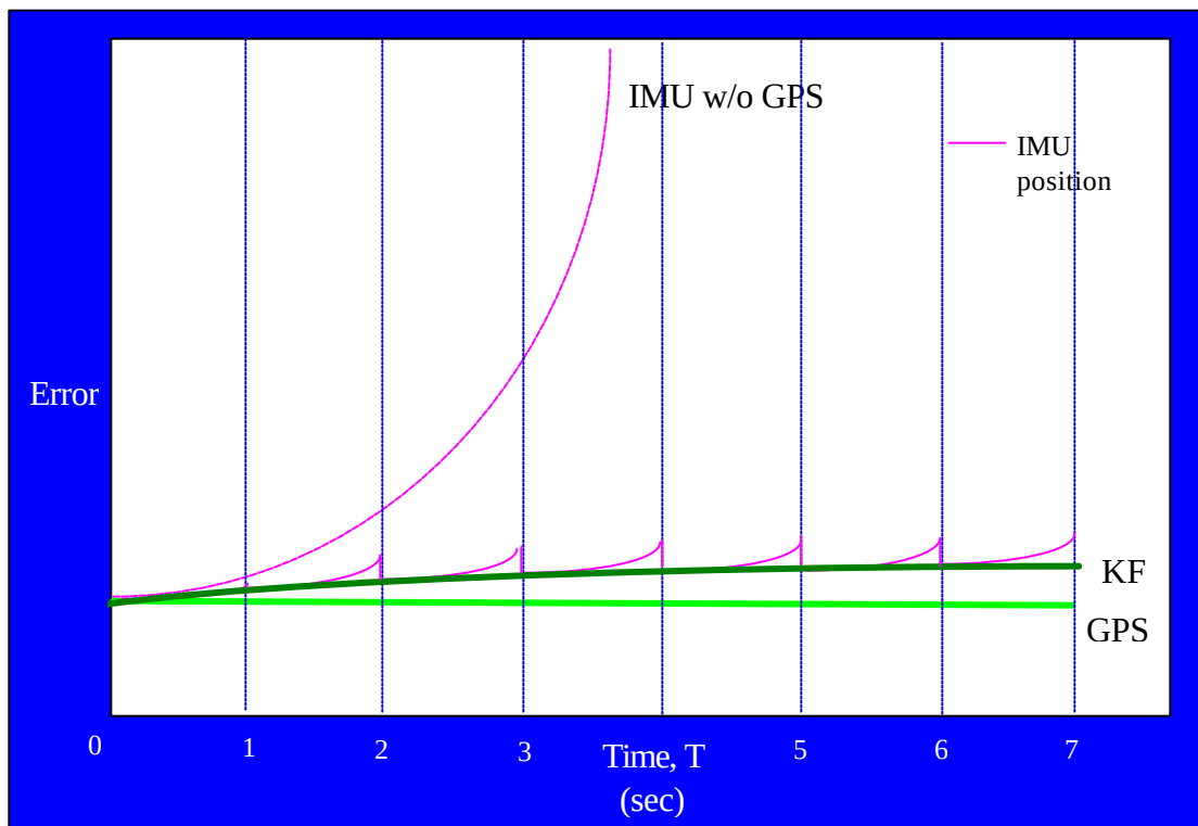
Figure 5.29: Detailed Error Curve for IMU/GPS.
