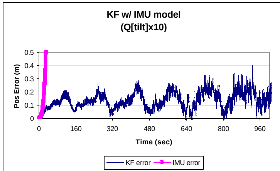
Figure 5.42: Tuned KF w/ Q = 10 \times [tilt rates].
