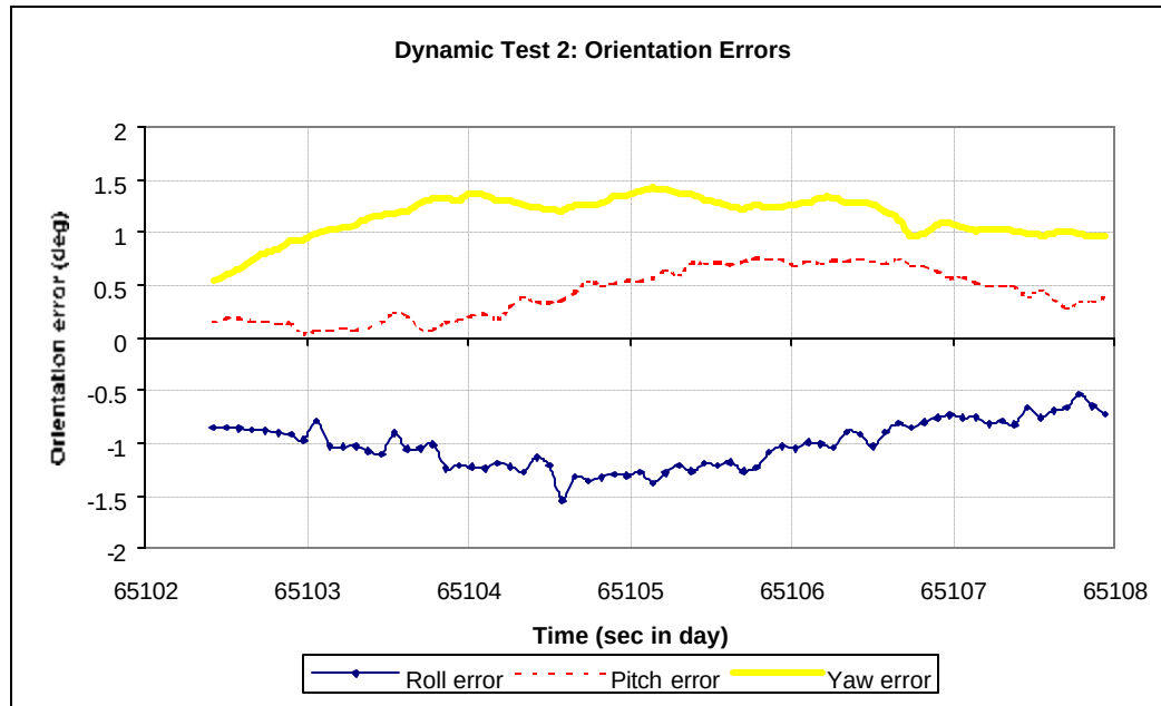
Figure 5.62: Dynamic Test 2 – Orientation Errors
