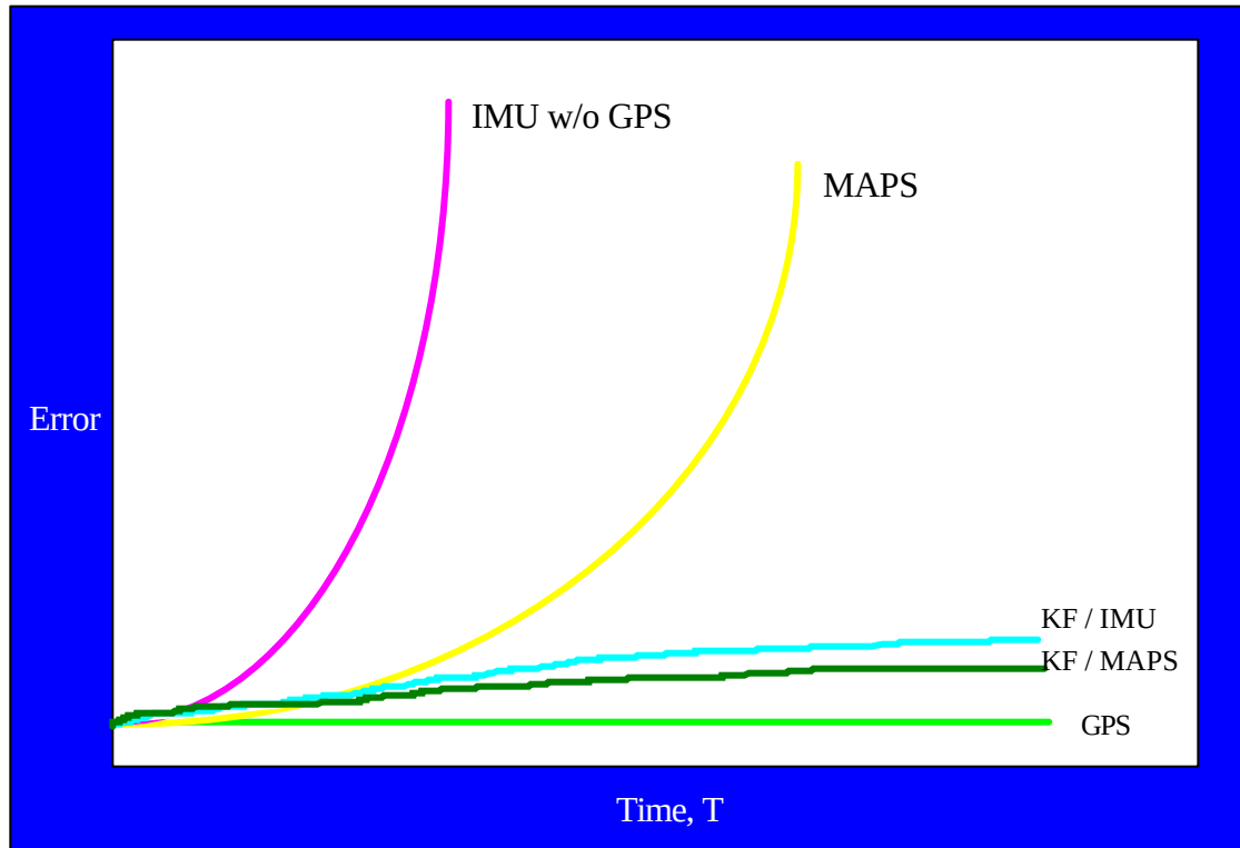
Figure 5.28: General Error Curves for MAPS/GPS and IMU/GPS.
