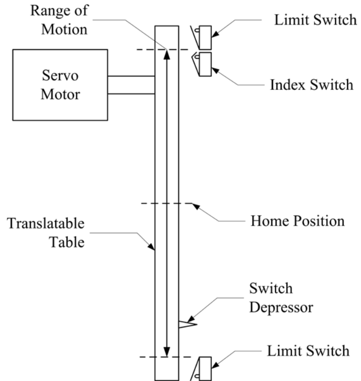
Figure 3-7: Typical Configuration of Index and Limit Switches in a Servo System
