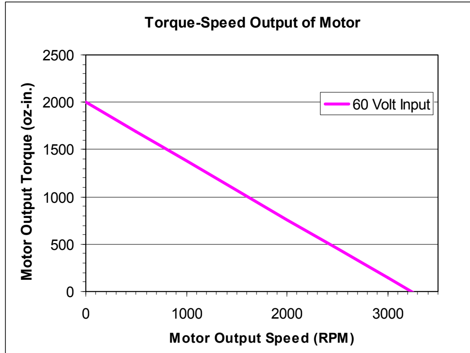
Figure 4-10: Torque-Speed Curve for U12M4H Servodisk Motor
