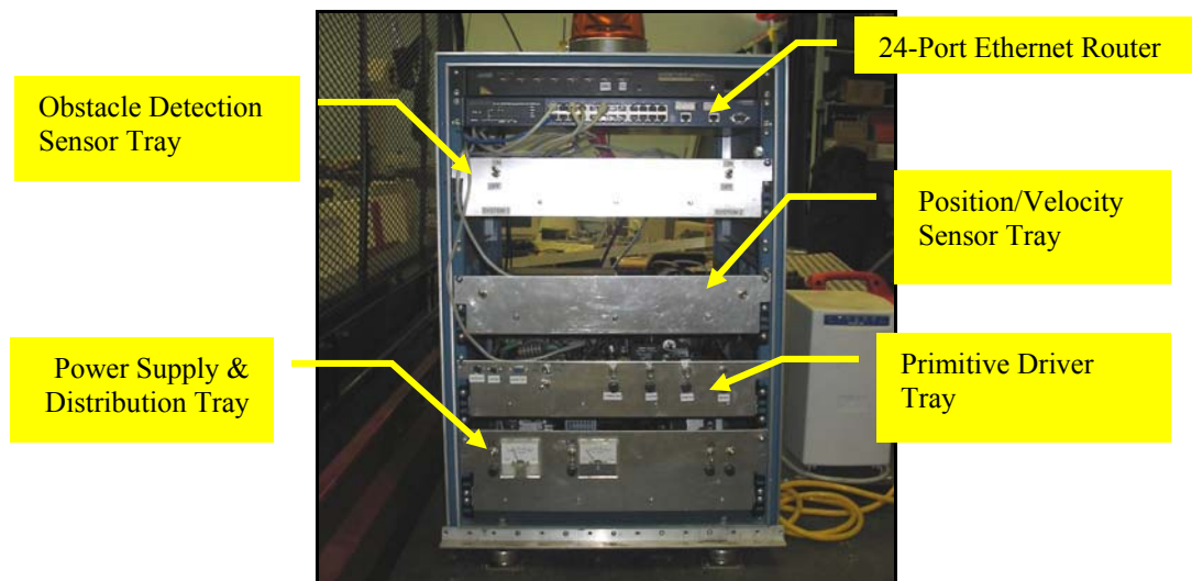
Figure 2-1: Electronics Rack for Tray Modules
