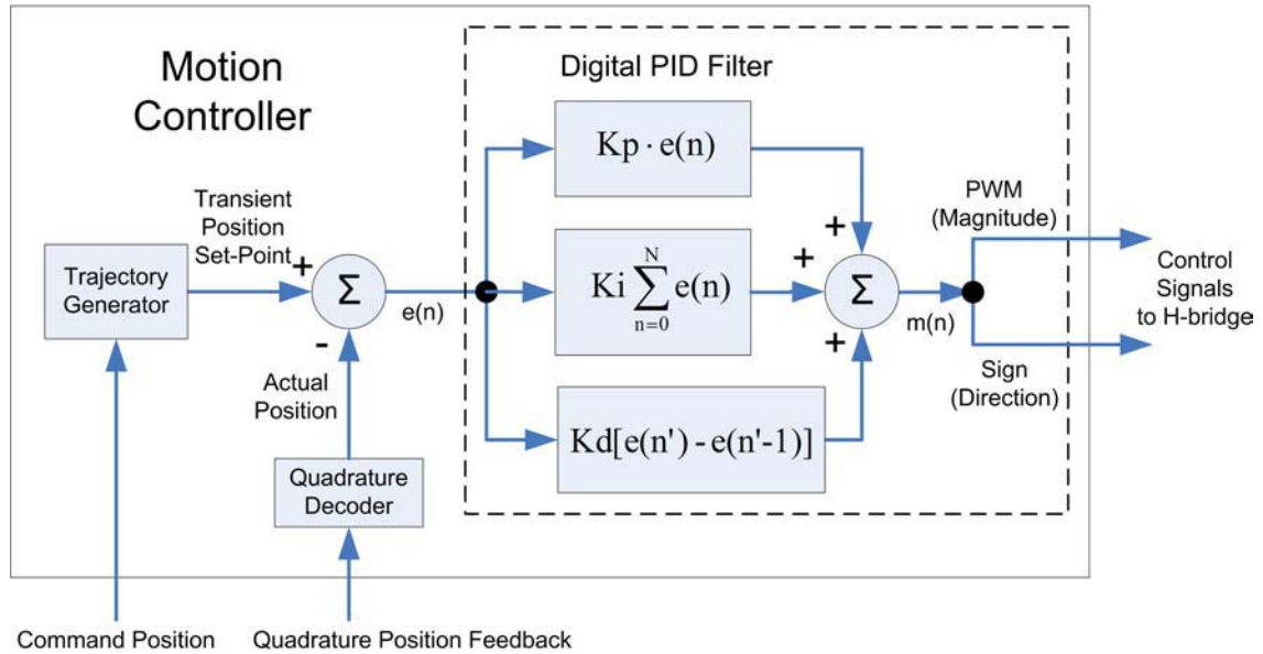
Figure 5-3: PID Filter Block Diagram
