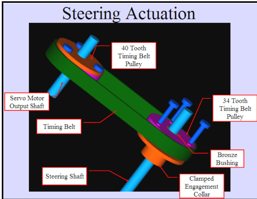
Figure 4-8: CAD Rendering of Steering Actuator Configuration
