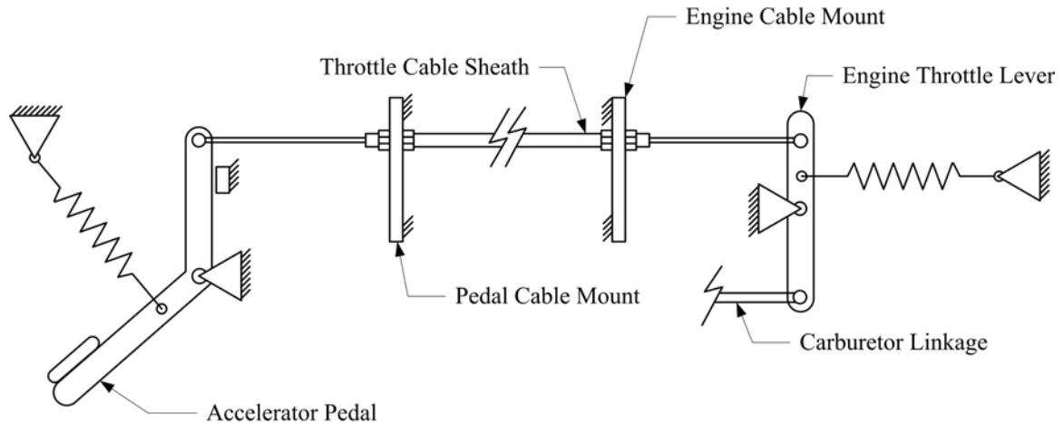
Figure 4-1: Stock Mule Throttle Control System
