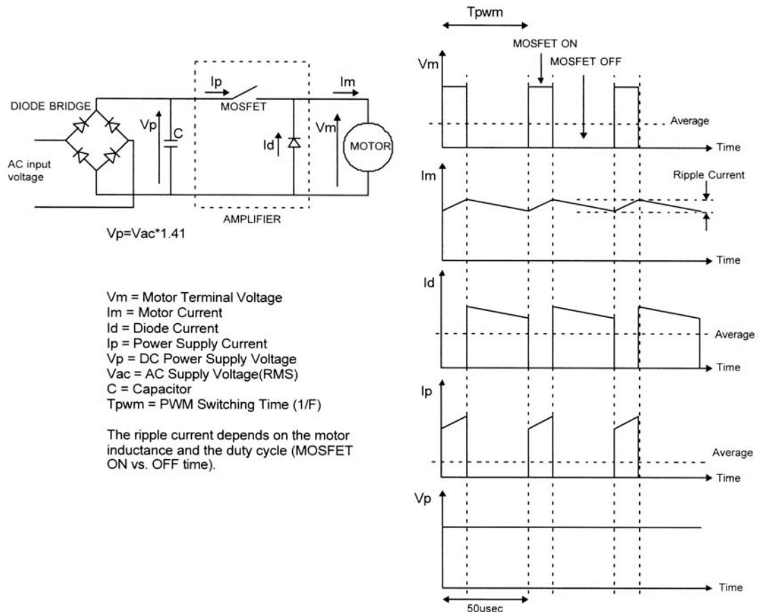
Figure 3-4: Simplified PWM Amplifier Circuit [Adv04a]
