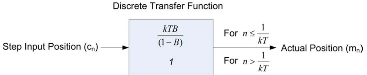
Figure 5-6: Discrete Transfer Function for Modeling Mule Actuator Systems
