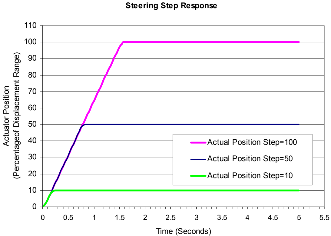
Figure 5-9: Steering Step Response to 10, 50, and 100 Percent Step Inputs
