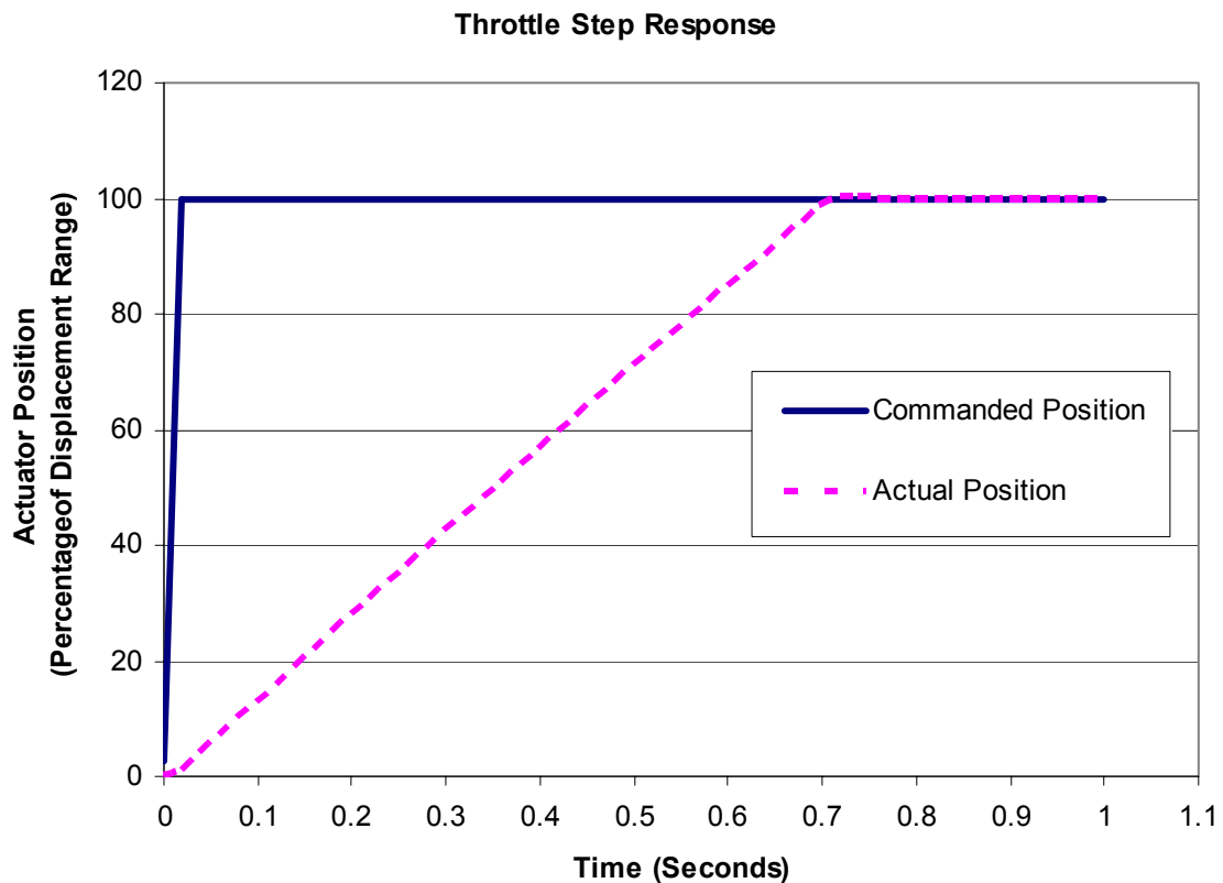
Figure 5-5: Step Input Produced by Throttle System Trajectory Generator
