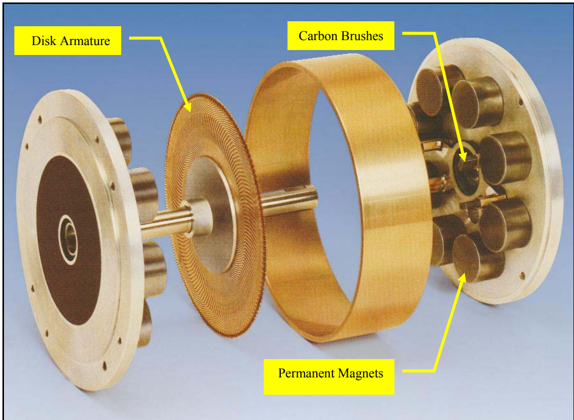
Figure 4-9: Exploded View of a Kollmorgen Servodisk Motor [Kol04]
