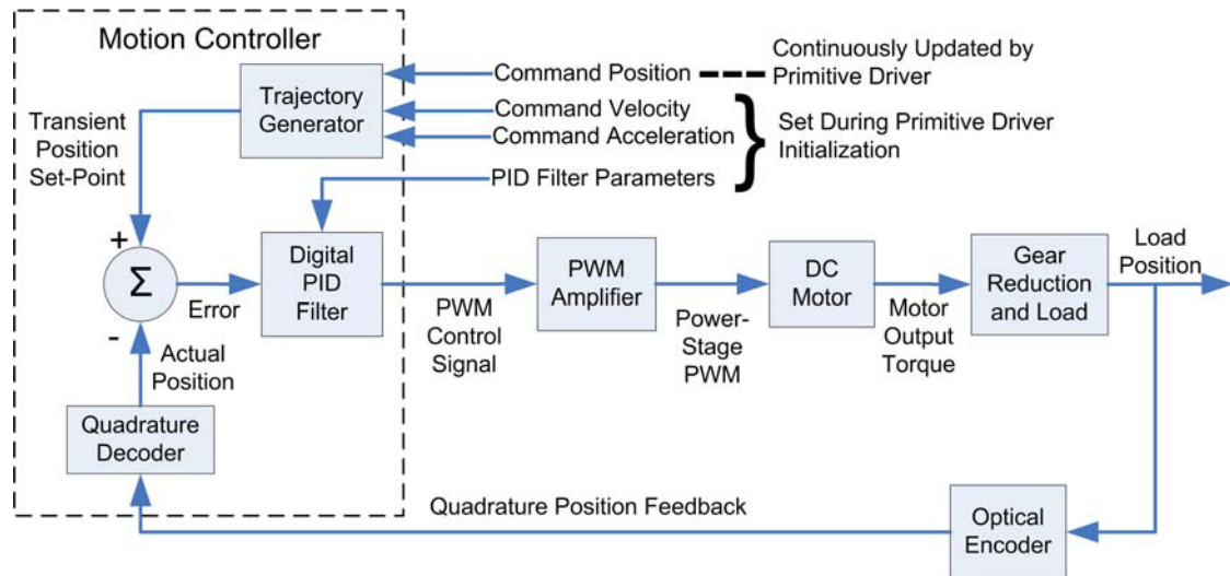
Figure 5-1: Block Diagram of Servo Systems Implemented on the Mule Actuators
