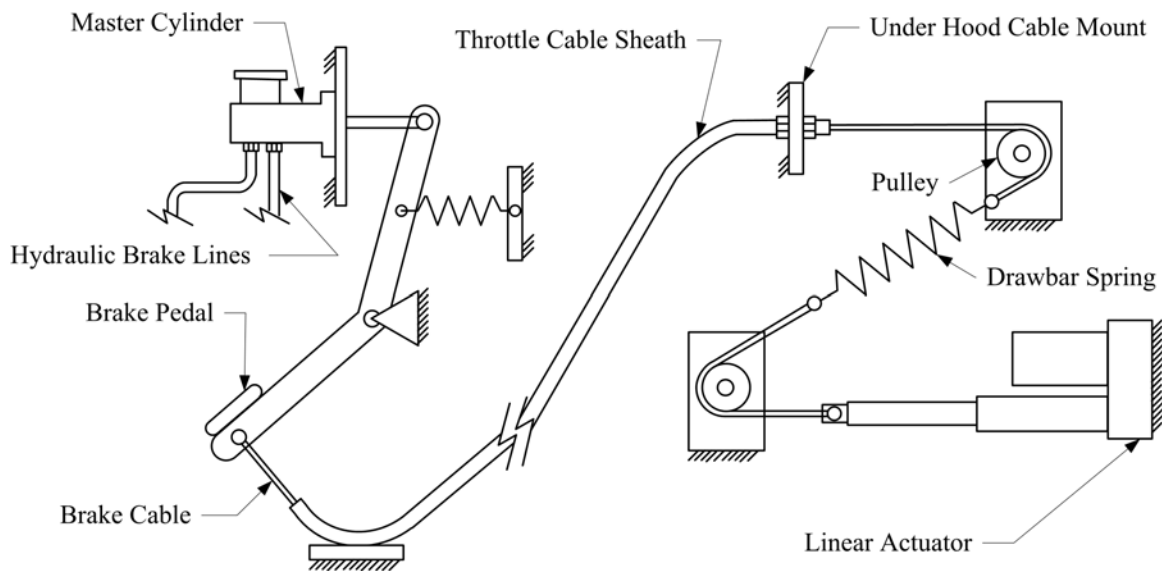
Figure 4-15: Functional Diagram of the Brake Actuator System
