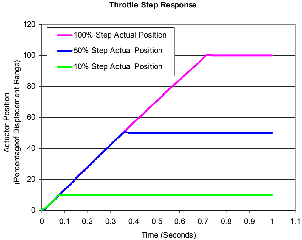
Figure 5-7: Throttle Step Response to 10, 50, and 100 Percent Step Inputs
