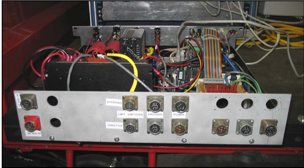
Figure 2-6: Primitive Driver Hardware Tray Module
