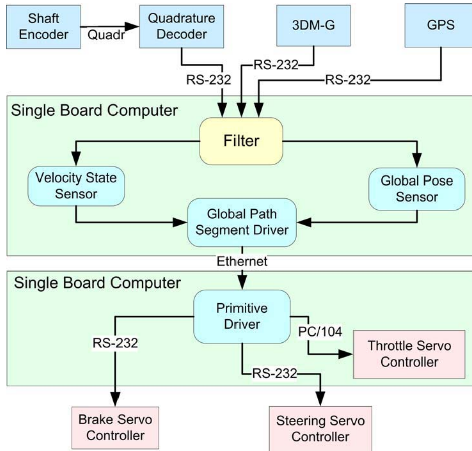
Figure 2-7: Current Mule Component Interface Configuration
