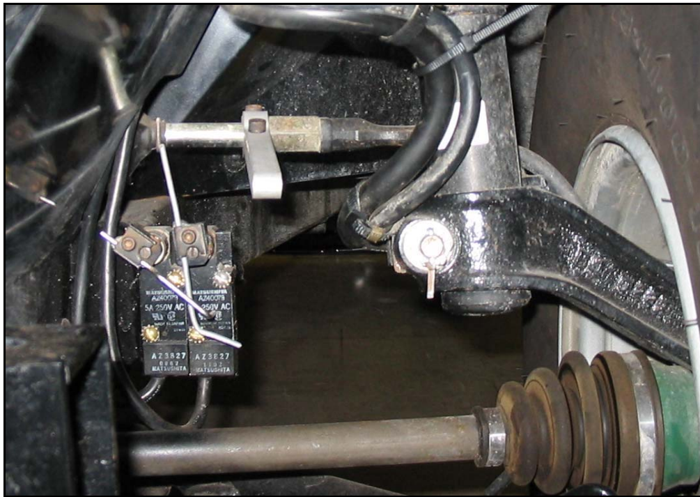
Figure 4-12: Steering Limit and Index Switches
