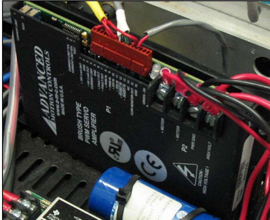
Figure 4-11: AMC PWM Amplifier
