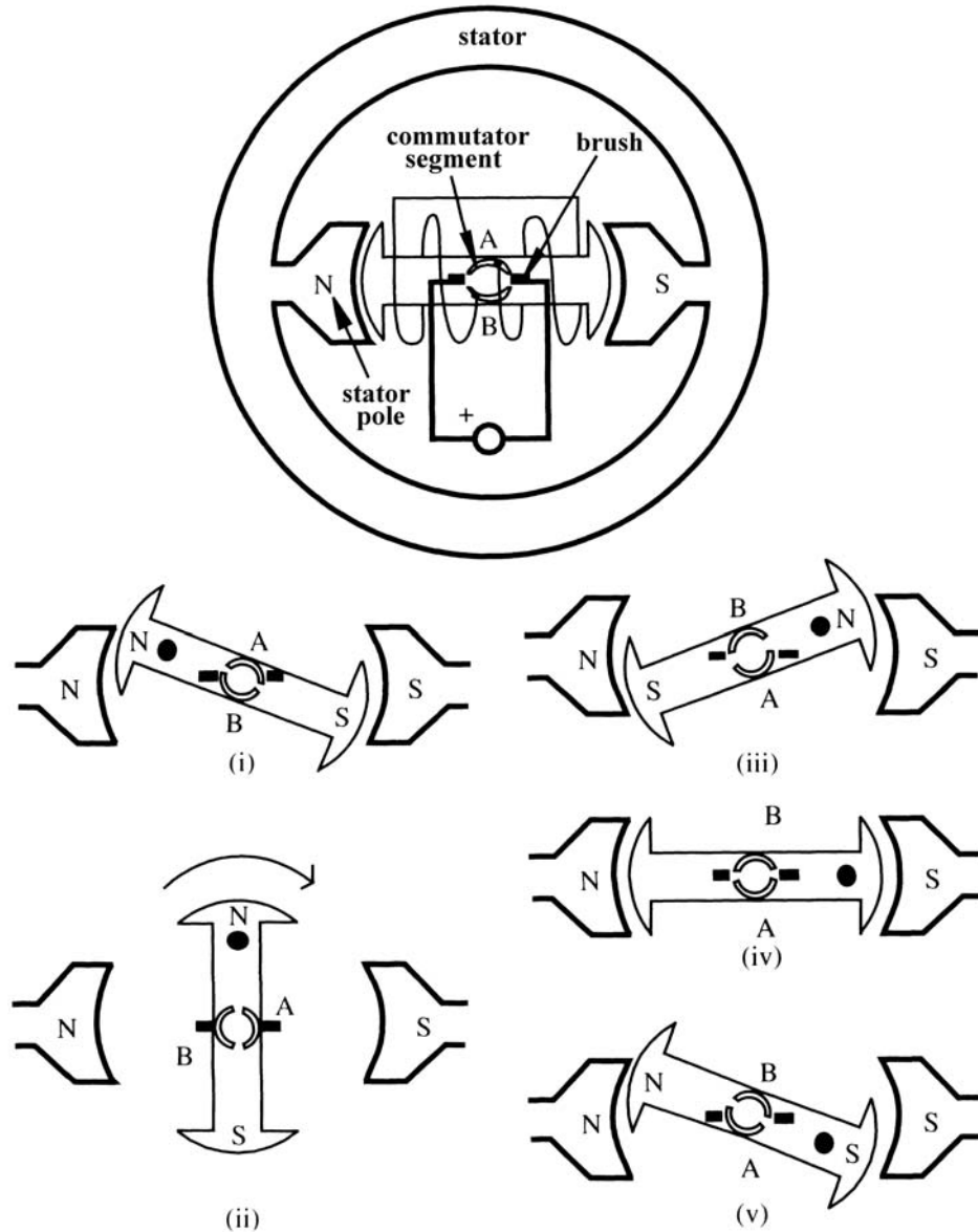
Figure 3-2: DC Motor Operational Theory [His98]
