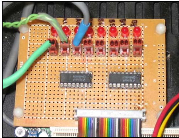
Figure 2-5: Digital Input Board
