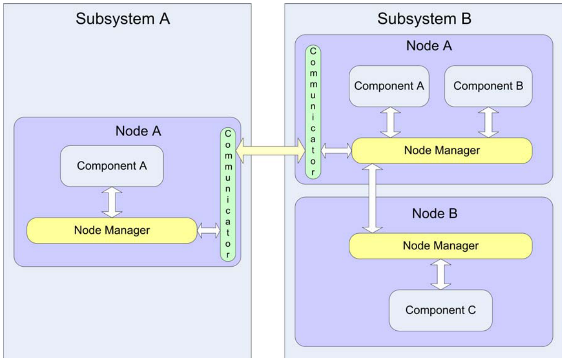
Figure 2-2: JAUS Communicator and Node Manager Interaction
