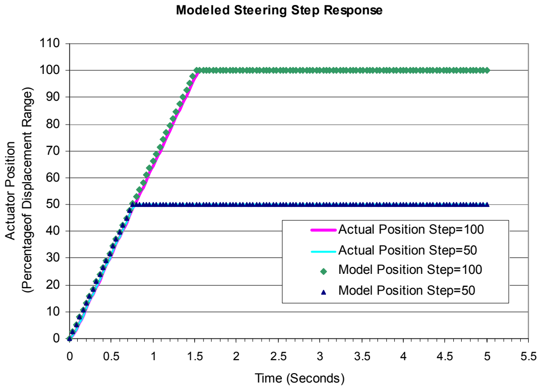
Figure 5-10: Discrete Transfer Function Model Plotted with Actual Steering Actuator Responses to Step Inputs of 50 and 100 Percent Displacement
