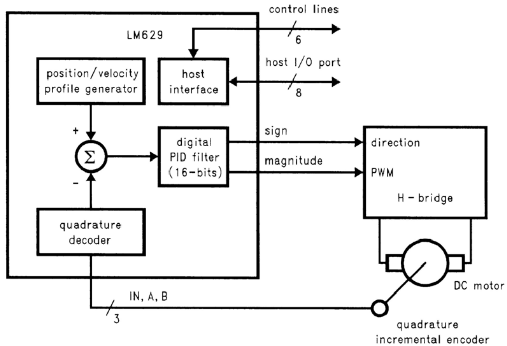
Figure 4-5: Typical LM629 Based Servo Motor Control System [Nat99]
