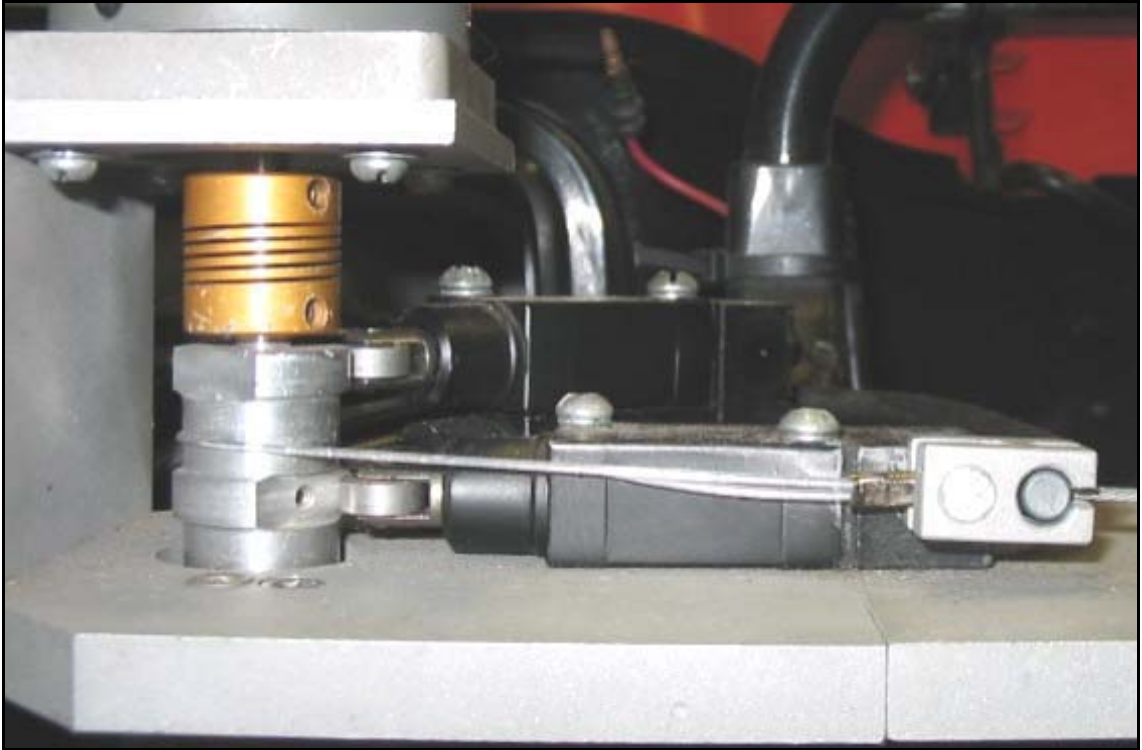
Figure 4-6: Servo Boss with Cam Tracks
