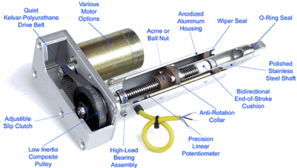
Figure 4-18: The Bug Actuator [Ult04]
