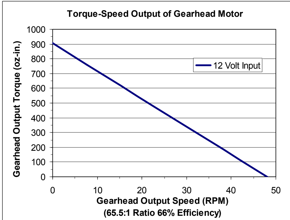
Figure 4-4: Torque-Speed Curve for the Gearhead Output
