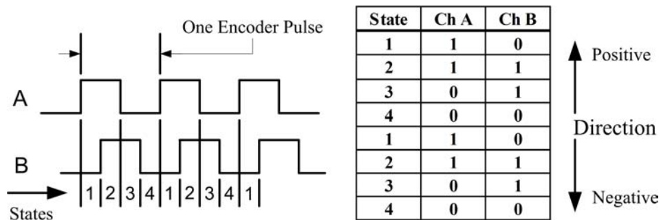
Figure 3-6: Encoder Output Signals and Quadrature States [Fre95]
