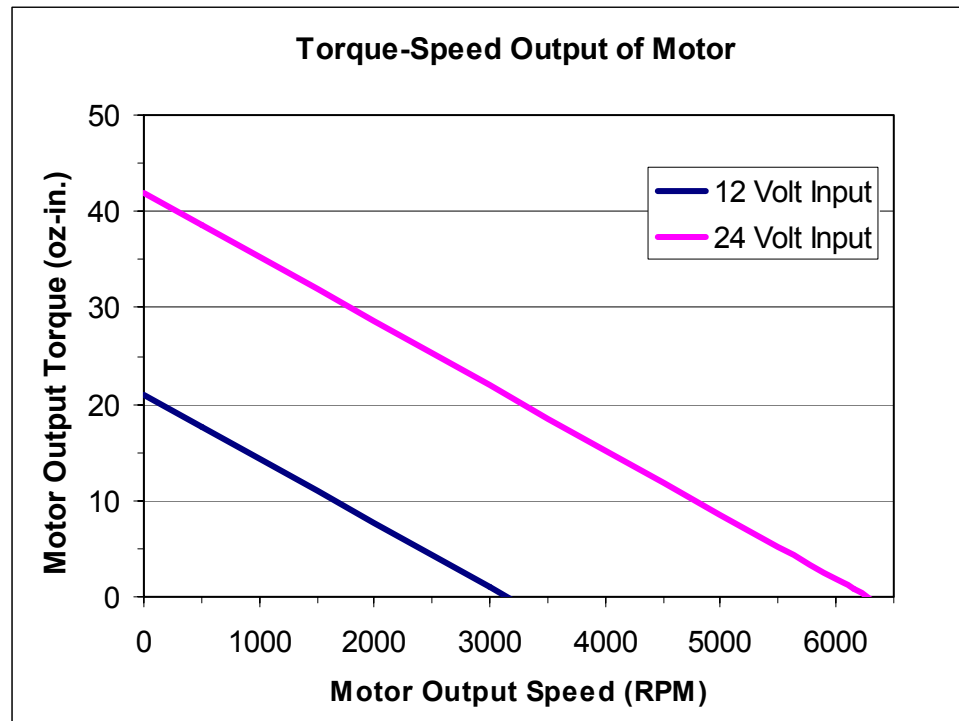
Figure 4-3: Torque-Speed Curve for Throttle Servo Motor
