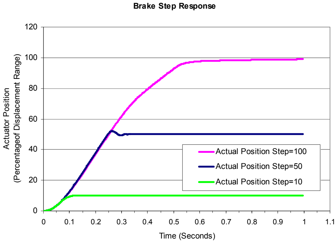
Figure 5-11: Brake Step Response to 10, 50, and 100 Percent Step Inputs
