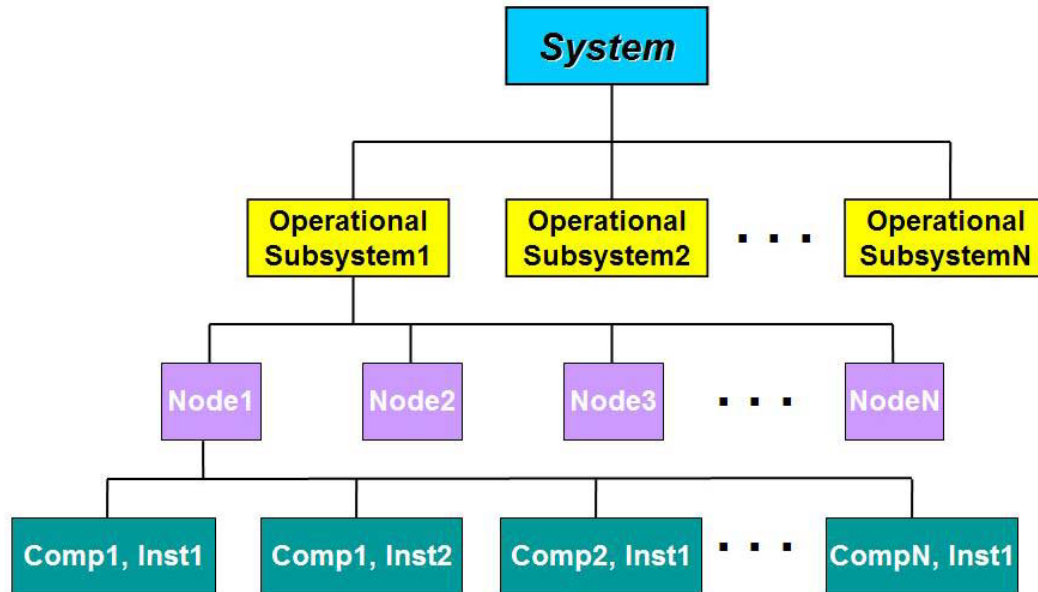
Figure 1-7: Diagram of JAUS Topology [Jau04]
