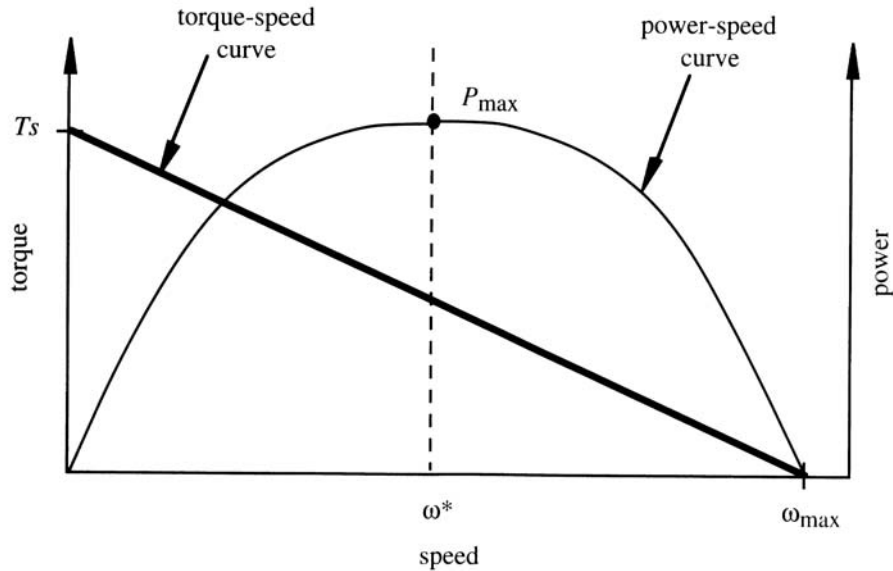
Figure 3-3: Typical Torque-Speed and Power Curves for a PMDC Motor [His98]
