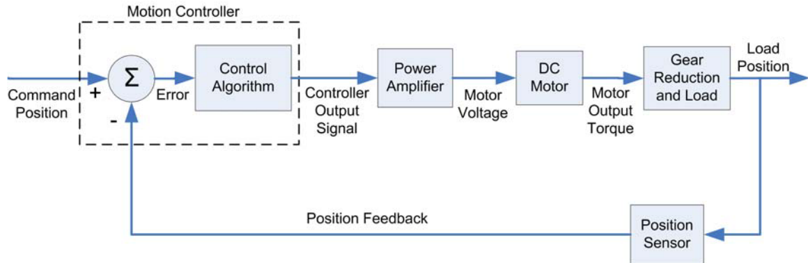
Figure 3-1: Typical Servo Control System
