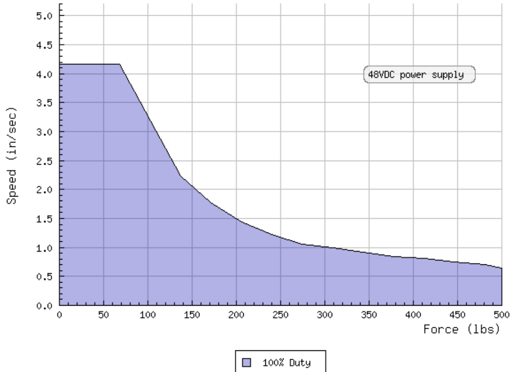
Figure 4-19: Thrust-Speed Curve for Smart Bug operated at 48 VDC
