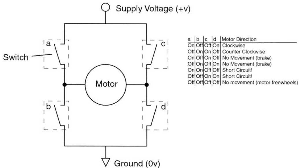
Figure 3-5: Simple H-bridge Circuit [Big03]
