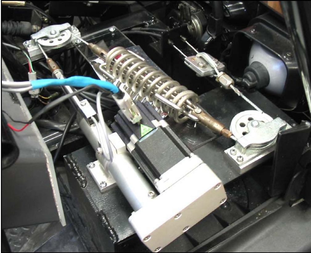
Figure 4-17: Brake Actuator System
