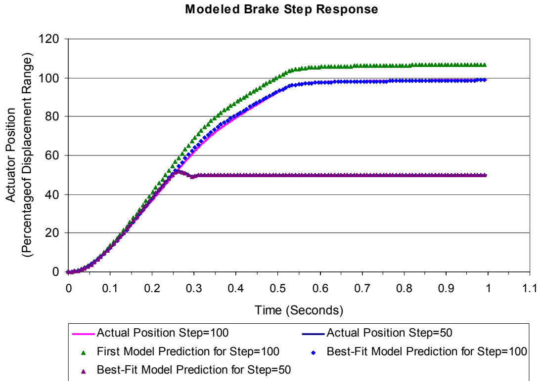
Figure 5-12: Discrete Transfer Function Models Plotted with Actual Brake Actuator Responses to Step Inputs of 50 and 100 Percent Displacement
