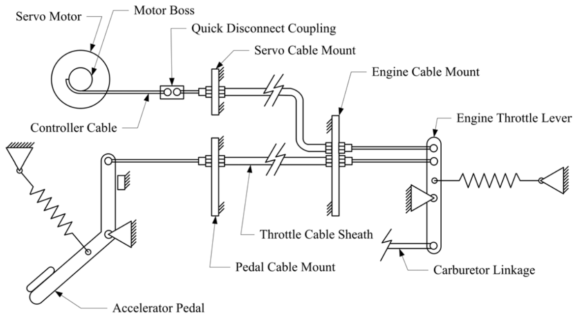
Figure 4-2: Actuated Mule Throttle Control System
