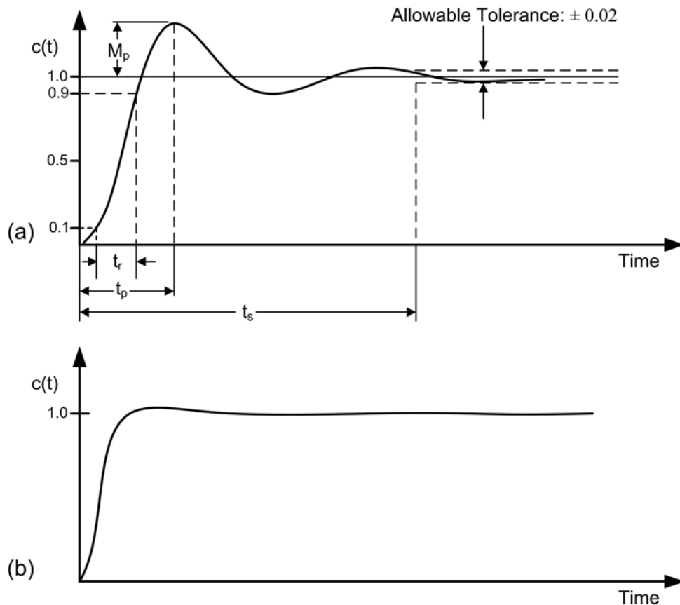
Figure 5-4: Unit Step Response Plots (a) Response Showing Transient Response Attributes (b) Response of a Critically Damped System
