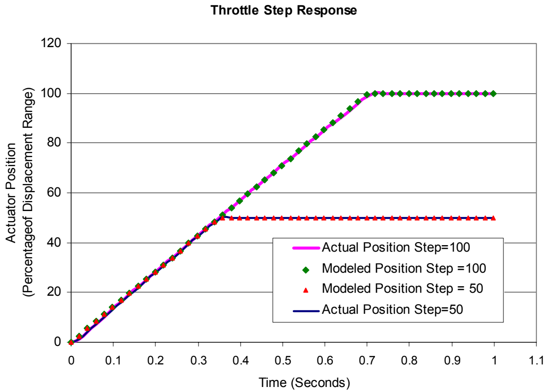
Figure 5-8: Discrete Transfer Function Model Plotted with Actual Throttle Actuator Response of for Step Inputs of 50 and 100 Percent Displacement
