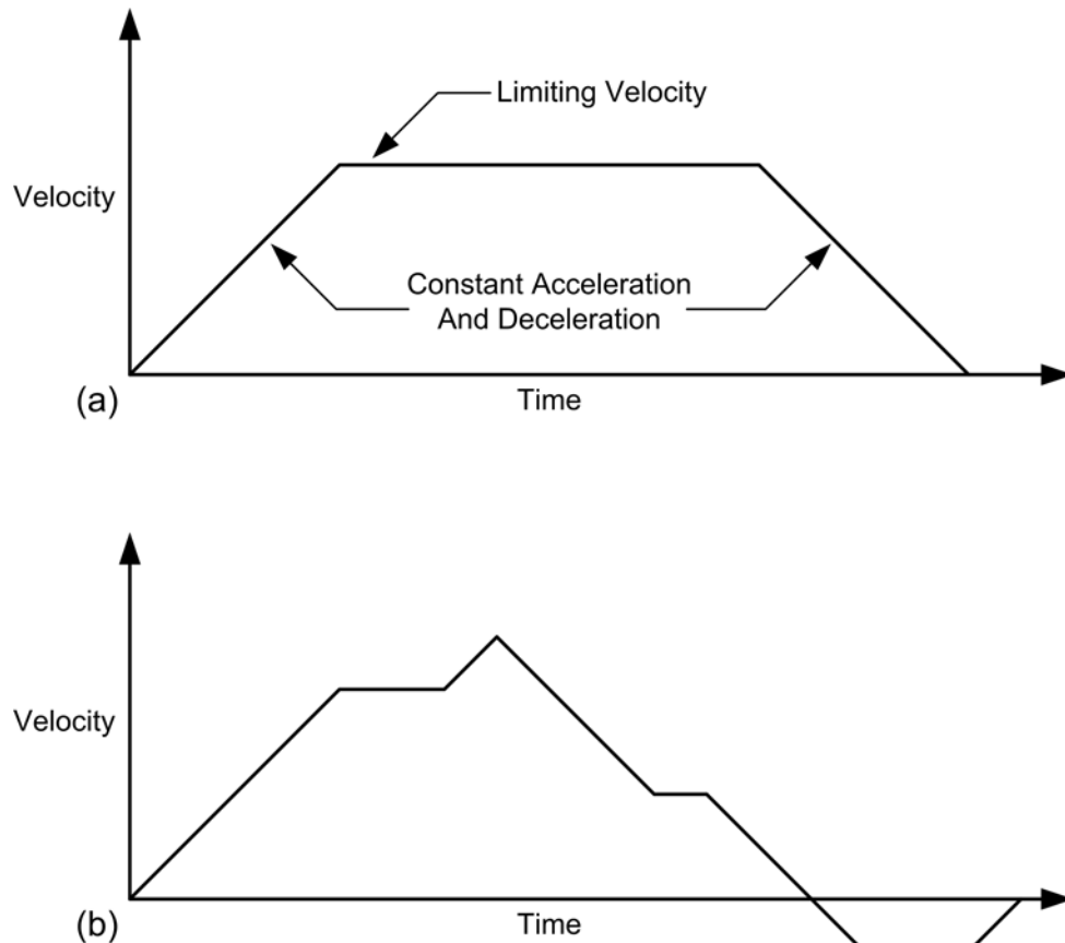
Figure 5-2: Trapezoidal Velocity Profile Graphs (a) Standard Profile (b) Modified Profile
