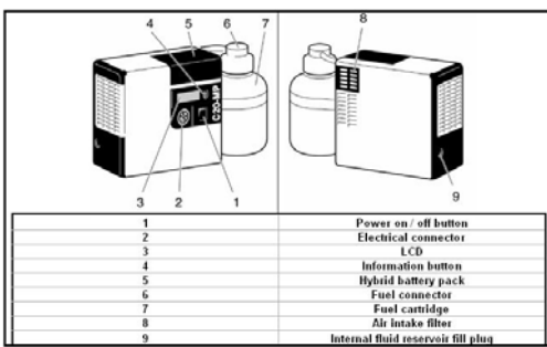
Figure 1. SFC Diagram
