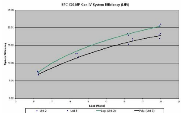
Figure 2. Efficiency Graph
