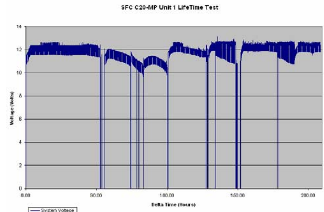
Figure 5. Unit 1 Lifetime Testing Graph
