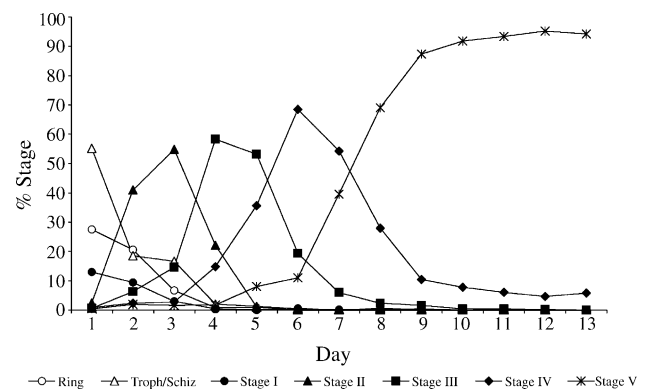
Fig. 1. Percentages of stages present at each day in the NF54 gametocyte development time course were monitored using Giemsa-stained blood smears. RNA was isolated on each day from Day 1 to Day 13 for hybridization to the microarray.
