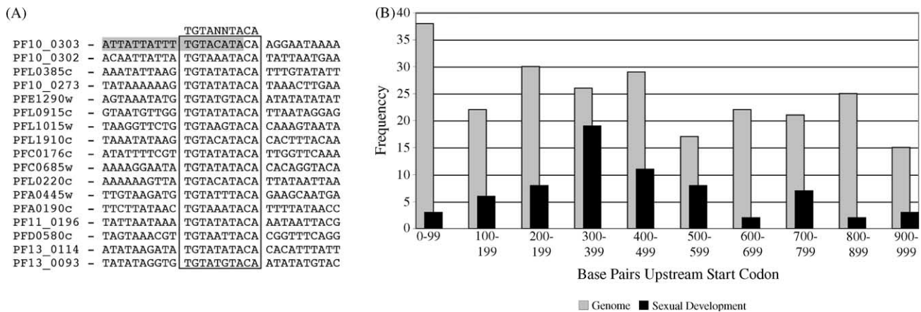
Fig. 5. (A) Alignment of examples of sequences from genes in the OPI sexual development cluster containing the TGTANNTACA motif in their promoter regions. Gray highlight indicates the 3'-most end of the promoter region upstream of pfs25 (PF10_0303) deleted by Dechering et al. (exo5 construct) that resulted in a reduction of luciferase reporter activity to ~5% that of the full-length promoter construct [30]. B) Distribution of the TGTANNTACA motif in the 1000 base pair upstream regions relative to the start codon of genes in the OPI sexual development cluster (black) vs. genes in the remainder of the genome (gray). The motif frequency is highest between 200 and 600 bases for genes in the sexual development cluster, but relatively even across the upstream 1000 bases for genes not in the sexual development cluster.
