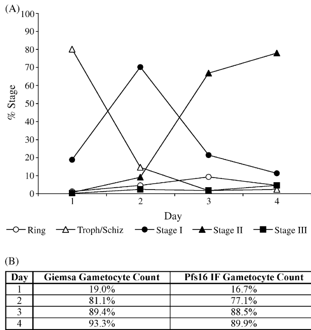
Fig. 2. (A) Percentages of stages present in the CS magnetic affinity column purified 3D7 time course were monitored using Giemsa-stained blood smears. Column separation was conducted to remove contaminating asexual stages immediately after Day 1 sample collection. RNA was isolated on each day for hybridization to the microarray. (B) Giemsa-stained blood smear counts of early-stage gametocytes were confirmed to within 5% for each day using immunofluorescence. Antibody against the gametocyte-specific protein Pfs16 allowed a comparison between the abundance of sexual parasites (Pfs16 fluorescent) vs. overall infected erythrocytes (DAPI fluorescent).
