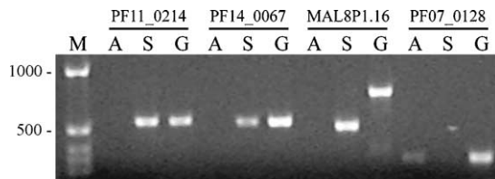
Fig. 4. Validation of microarray data with semi-quantitative RT-PCR. Lanes: M: DNA marker; A: asexual stage cDNA template (from NF54 mixed asexual population); S: sexual stage cDNA template (from NF54 Day 7 gametocytes); G: NF54 genomic DNA template (positive control). Products in lanes S and absent from lanes A for the hypothetical genes PF11_0214, PF14_0067 and MAL8P1.16 demonstrate sexual stage specific expression, as shown by microarray analysis. Likewise, product in lane A and absent in lane S for eba-175 (PF07_0128) demonstrates asexual-specific expression as previously reported. For MAL8P1.16, primers were designed such that they spanned an intron to allow for the detection of any possible contaminating genomic DNA template, of which none was observed. All product sizes were as expected.
