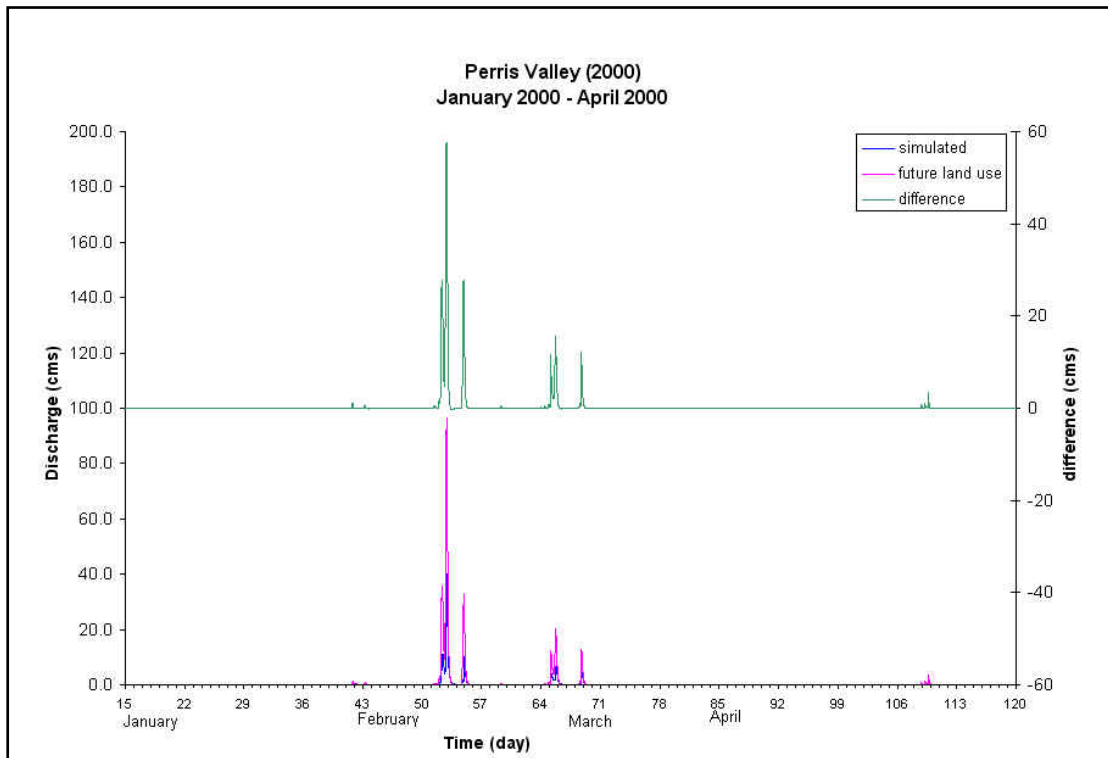
Figure 11. Streamflows and their differences for current and projected land use conditions.
