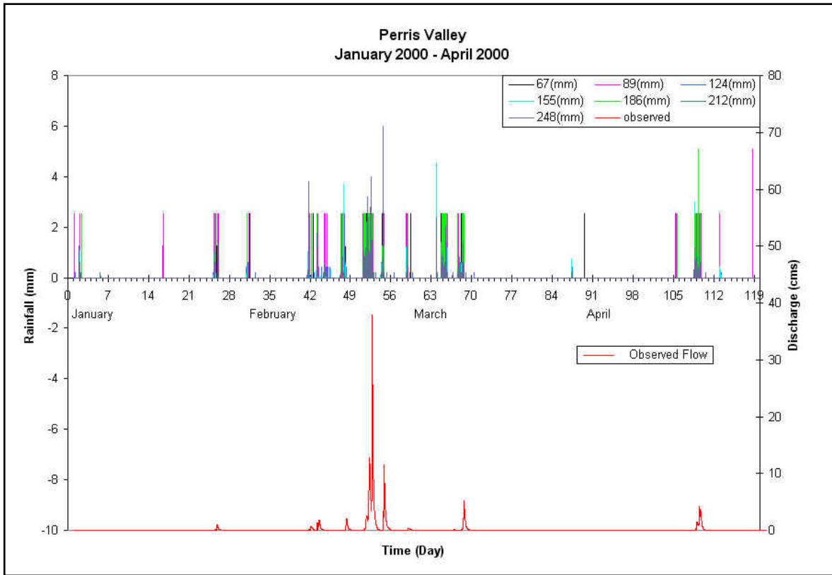
Figure 7. Observed stream flow data with associated rainfall data from all gaging stations.
