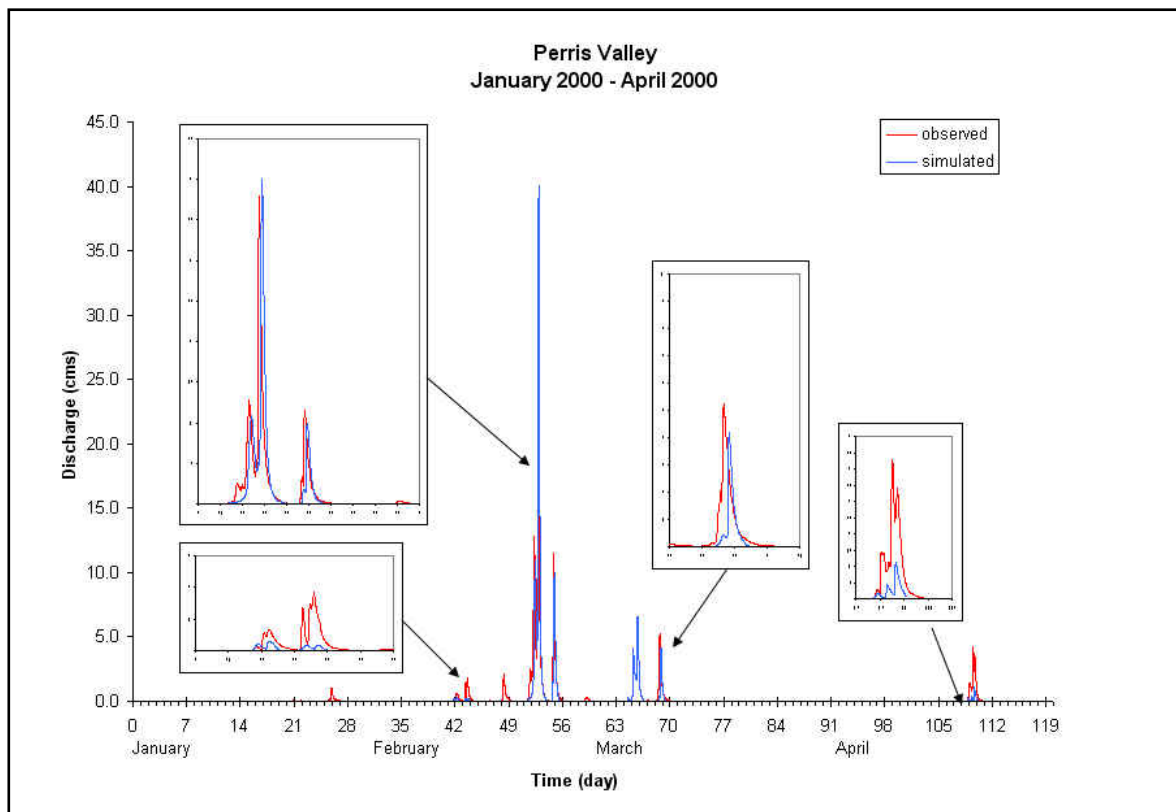
Figure 8. Observed and simulated streamflow data.
