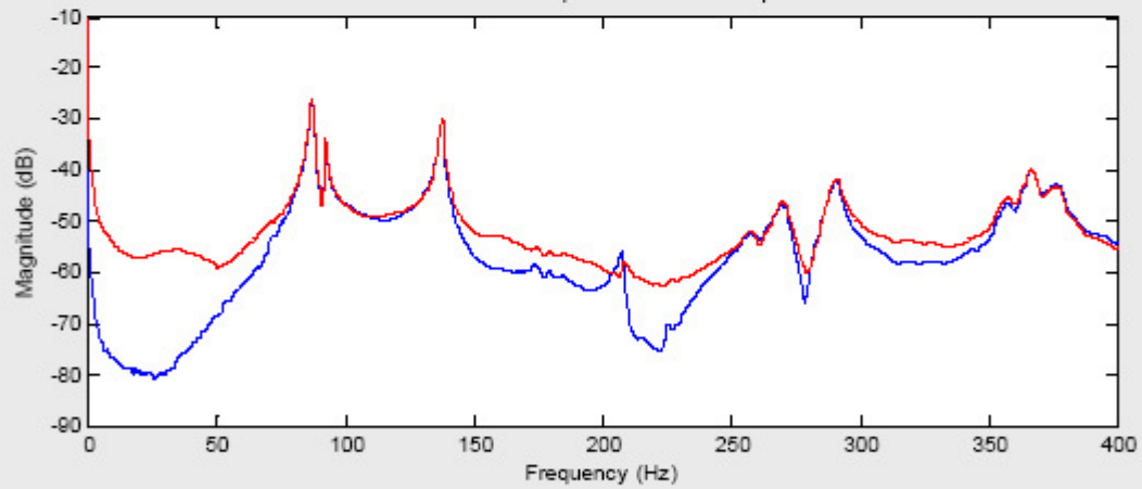
Mode Determination for SimpleSAT - Trial #8 Experimental Data
