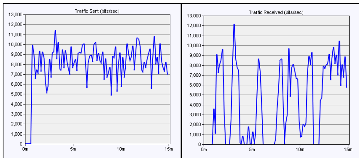
Figure 4.1 Goodput for AODV Routing Protocol Only
