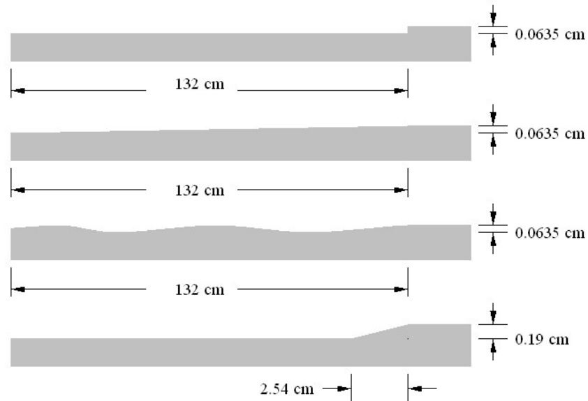
Figure 10 - Examples of Possible Rail Asperities
