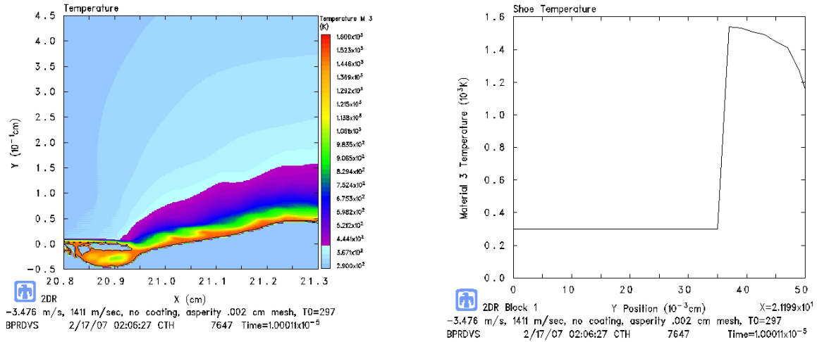
Figure 62 - Temperature for 1,411 m/s, Asperity, No Coating, Initial Ambient Temperature
