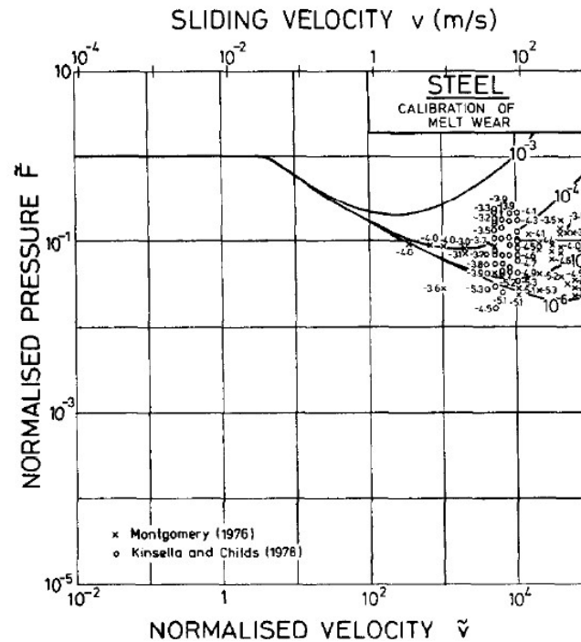
Figure 27 - Lim and Ashby Model for Melt Wear [18:13]
