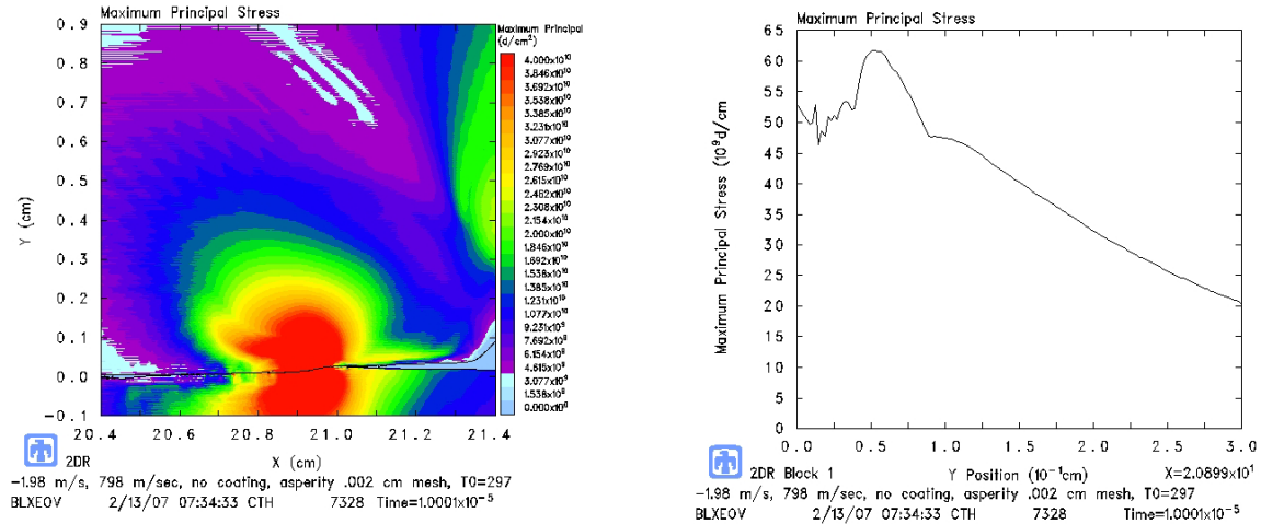
Figure 59 - Maximum Principal Stress for 798 m/s, Asperity, No Coating, Initial Ambient Temperature
