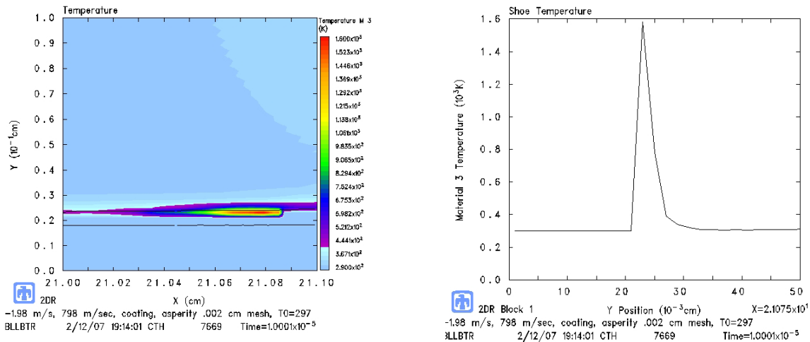
Figure 50 - Temperature for 798 m/s, Asperity, Coating, Initial Ambient
