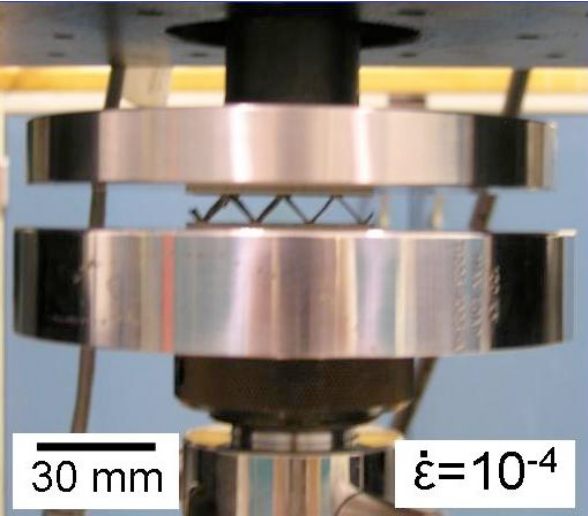
Figure 2: Set-up of flatwise compression testing.
