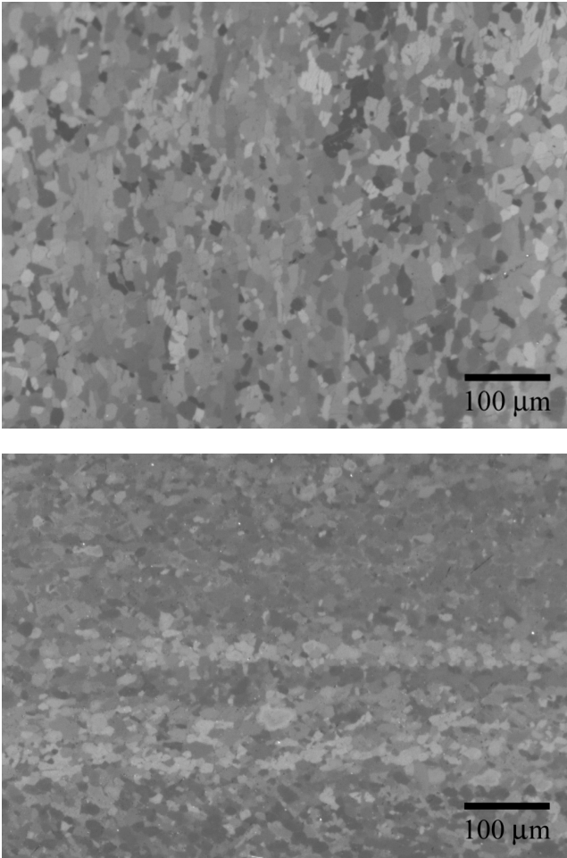
Figure 3: (Top) Monolithic Ti-6Al-4V microstructure, (Bottom) Weld + HIP Ti-6Al-4V microstructure.
