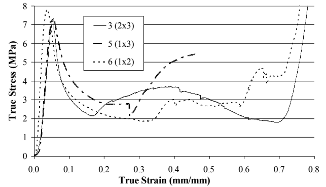
Figure 6: True stress-strain results for core compression tests (Strut Failure)
