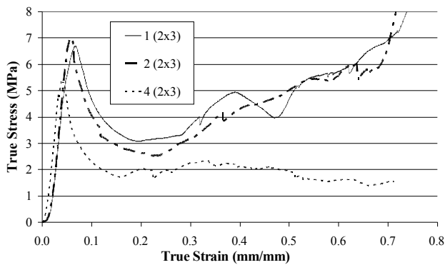
Figure 5: True stress-strain results for core compression tests (Joint Failure)
