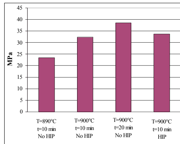
Figure 7: Double-lap shear strength results for CP titanium brazed with BRAZ1954 for described thermal cycles.
