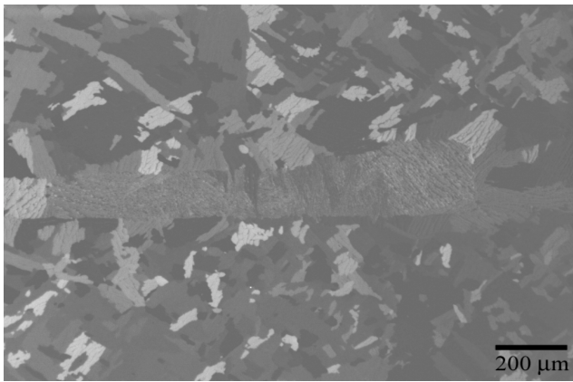
Figure 4: (Top) DB + HIP Ti-6Al-4V higher magnification image, (Bottom) Braze + HIP Ti-6Al-4V higher magnification image.
