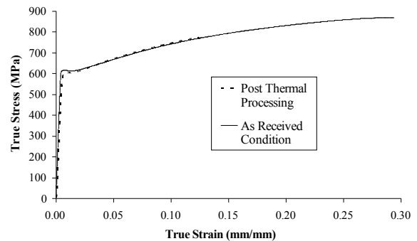
Figure 8: True stress-strain results for as-received and post thermally processed CP titanium (0.024 mm thick sheet perpendicular to the rolling direction)
