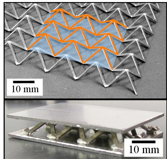
Figure 1: Examples of the geometry of titanium pyramidal core with and without brazed facesheets.
