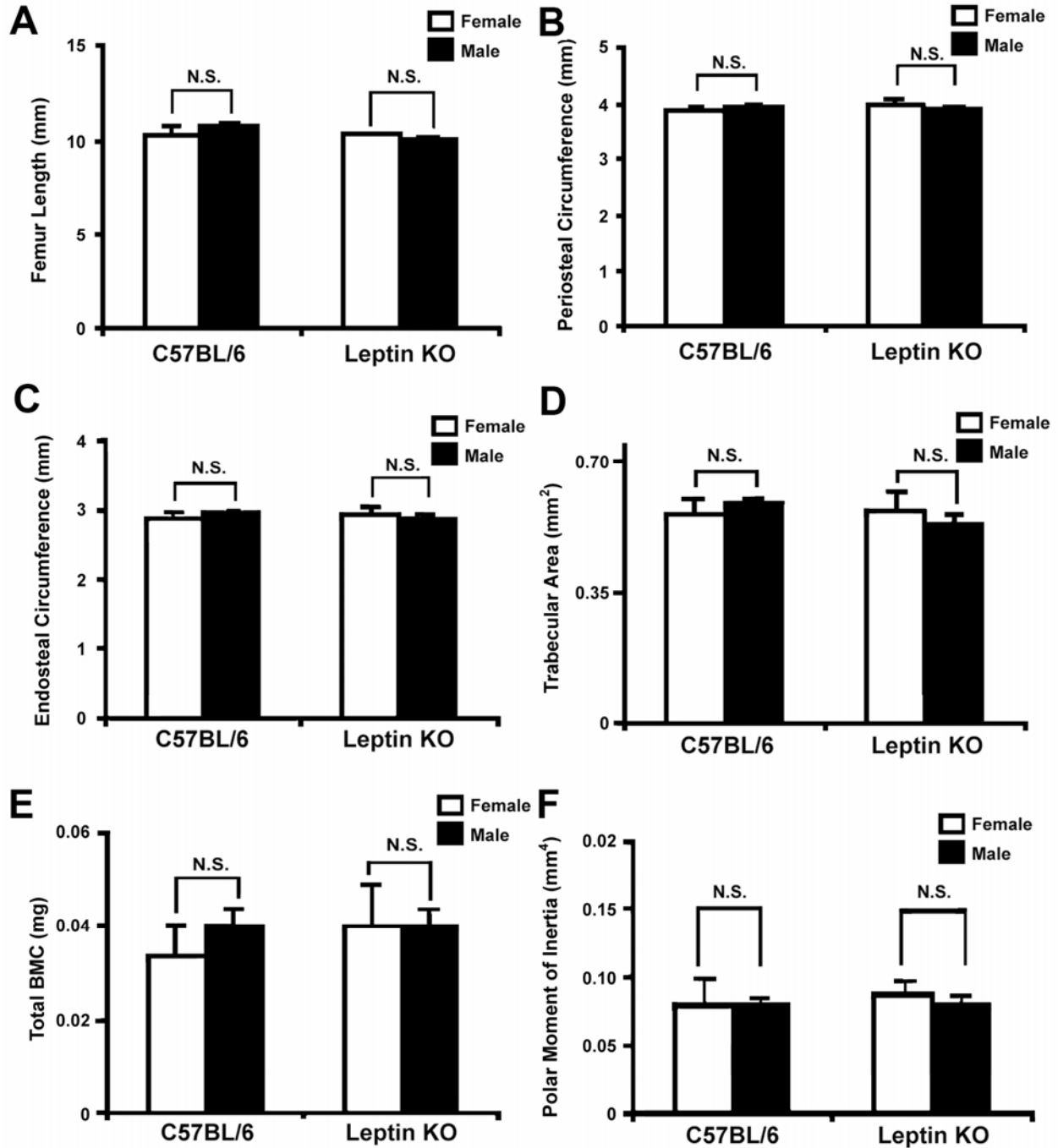
Figure 3. Summary of the phenotypic comparison of femurs from pre-pubertal male and pre-pubertal female leptin knockout (KO) and C57BL/6 wild-type mice. The measurements determined were those of the 10-week-old mice, (A) length, (B) PC, (C) EC, (D) TA, (E) total BMC and (F) polar moment of inertia. Values are expressed as mean \pm Standard Error of the Mean (SEM). Statistical analysis was performed by two-way ANOVA with a post-hoc Newman-Kuels Test. Differences were deemed significant if p < 0.05 .
