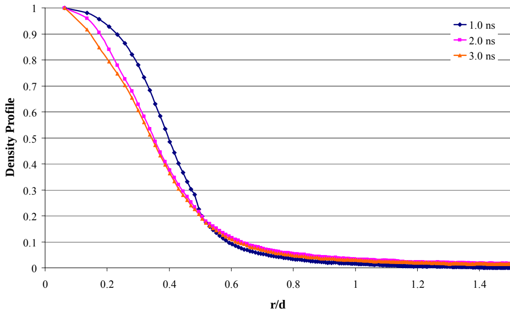
Figure 46. Radial Density Profile at z/d=0 , U_0 = 0 m/s, Acoustic Interference Model
