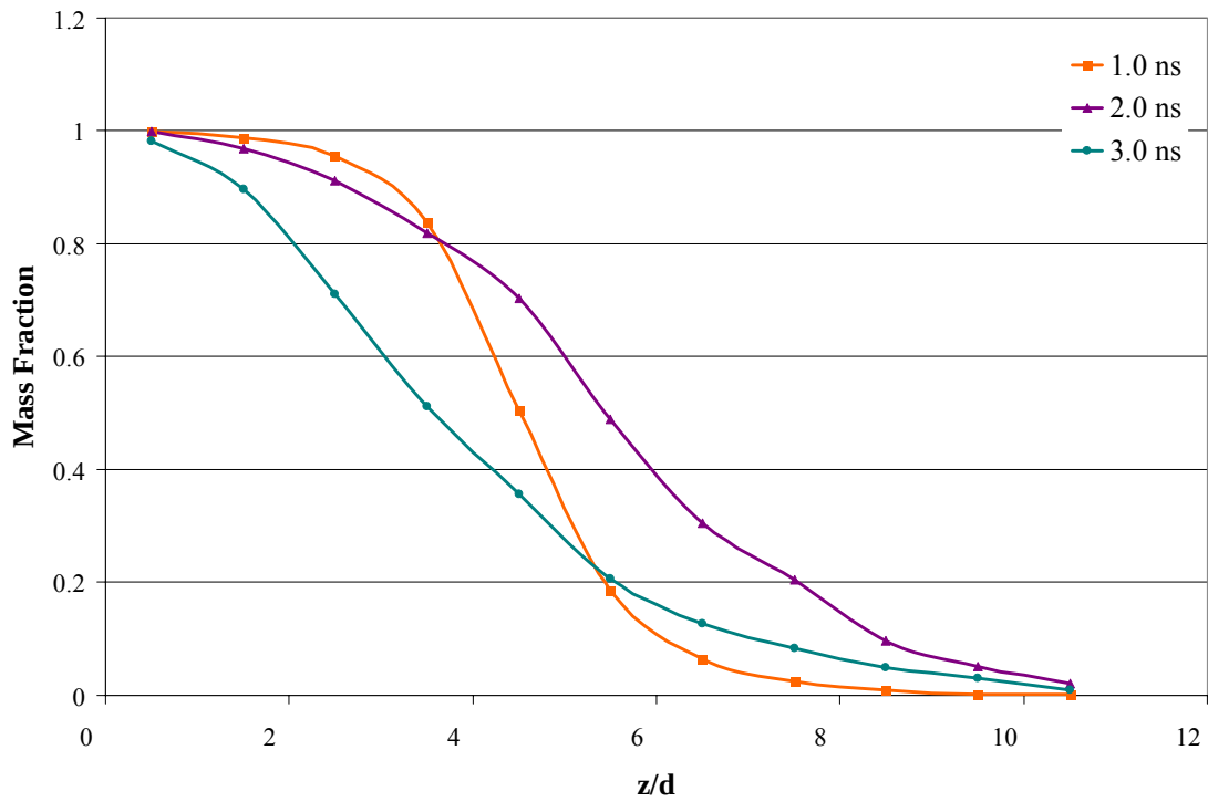
Figure 28. Mixing Along Centerline, U_0=300 m/s, Acoustic Interference Model
