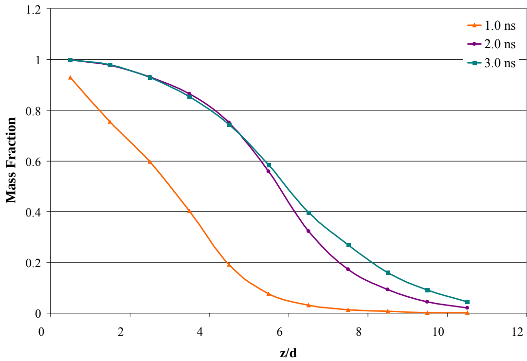
Figure 27. Mixing Along Centerline, U_0=300 m/s, Acoustic Free Model
