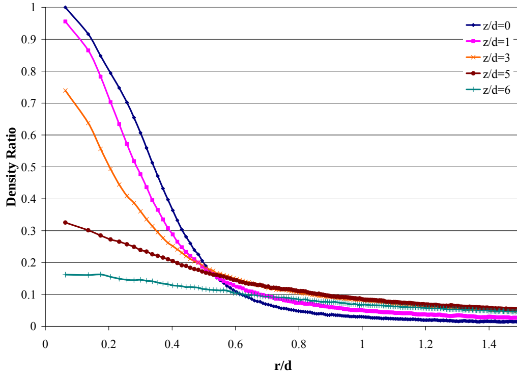
Figure 45. Radial Density Profile at 3.0 ns, U_0 = 0 m/s, Acoustic Interference Model
