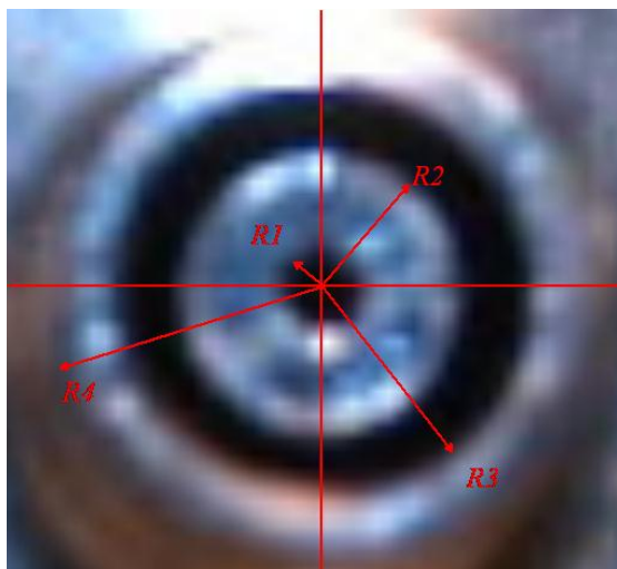
Figure 5. Close-up image of the coaxial injector tip area, the dimensions of the injector are: R_1 = 0.25 mm, R_2 = 0.79 mm, R_3 = 1.21 mm and R_4 = 1.59 mm. (Davis and Chehroudi, 2006)
