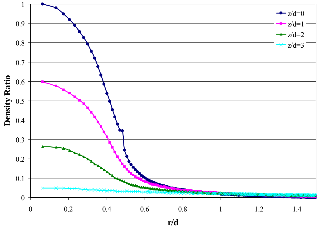
Figure 53. Radial Density Profile, 1.0 ns, U_o = 50 m/s, Acoustic Interference Model
