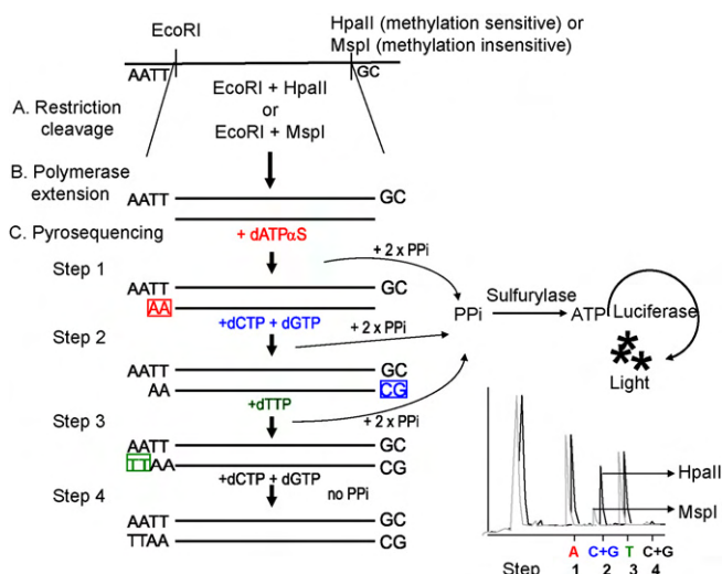
Fig. 9. Procedures for analysis global DNA methylation with luminometric methylation assay (LUMA). Genomic DNA is digested with combinations of restriction enzymes, EcoRI / MspI or EcoRI / HpaII , to leave the TTAA ( EcoRI ) and CG ( HpaII [methylation-sensitive] or MspI [methylation-insensitive]) overhangs. Next, the extent of the cleavage is determined by a polymerase extension assay based on a four-step pyrosequencing reaction. Inorganic pyrophosphate (PPi) is generated at each nucleotide addition in the polymerase extension assay. Signals are generated based on the utilization of PPi in a luciferase-based reaction. The amount of light generated is directly proportional to the number of overhangs produced by respective restriction enzymes. The A and T peaks represent signals from Steps 1 and 3. The C + G peaks resulting from Step 2 illustrate HpaII or MspI cleavage. The second C + G peak originating from Step 4 is an internal control for the completion of Step 2. Unmethylated CG is cleaved by HpaII , and a CG overhang is left after the cleavage and amplified in polymerase extension. Methylation status can be determined by analyzing the HpaII / MspI ratio at CG peaks from Step 2. The HpaII / MspI ratio is close to 1 in the unmethylated sample but close to zero in the methylated sample.
