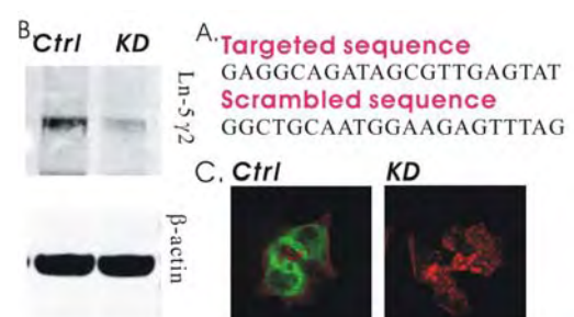
Fig. 1. shRNA knockdown of Rat \gamma 2 chain in 804G cells. A. The targeted and the corresponding scrambled sequences . B. Western blot analysis by using Ln-5 antibody 2778. C. 804G- \gamma 2 -kd and 804G- \gamma 2 -ctrl were stained by Ln-5 antibody 2778 (green) and phalloidin(red)
