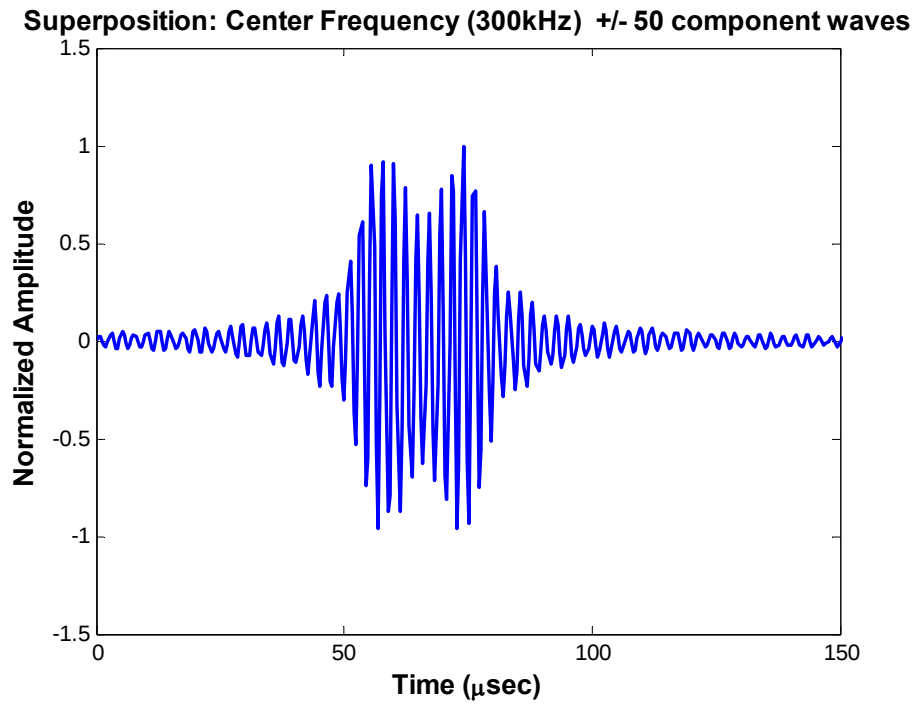
Figure 9: Superposition of 100 Component Waves
