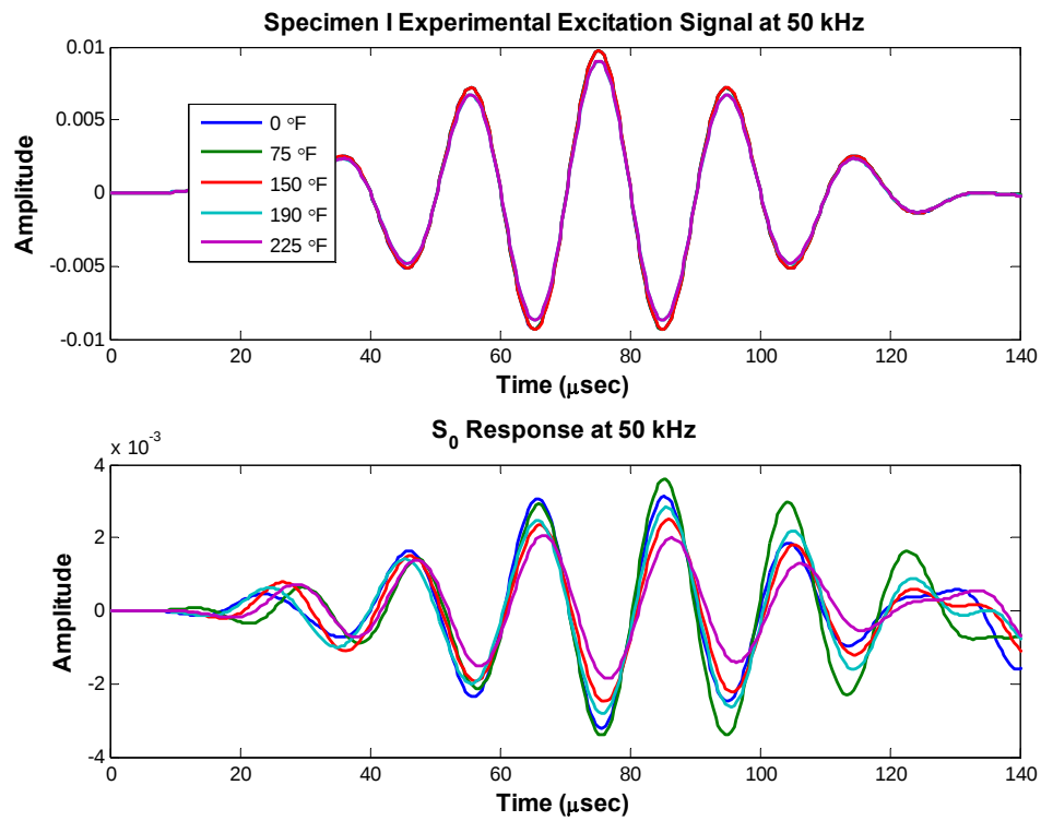
Figure 92: Specimen I Raw Signals at 50 kHz
