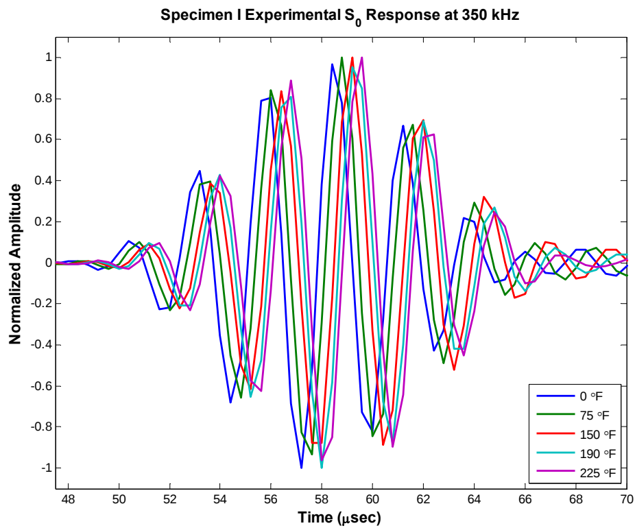
Figure 103: Specimen I Experimental S_0 Response at 350 kHz
