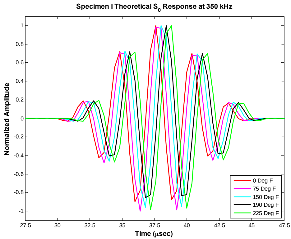
Figure 88: Specimen I Theoretical S_0 Response at 350 kHz
