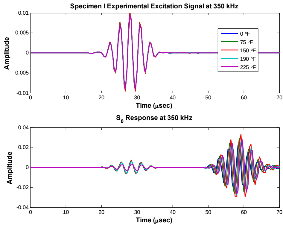
Figure 102: Specimen I Raw Signals at 350 kHz
