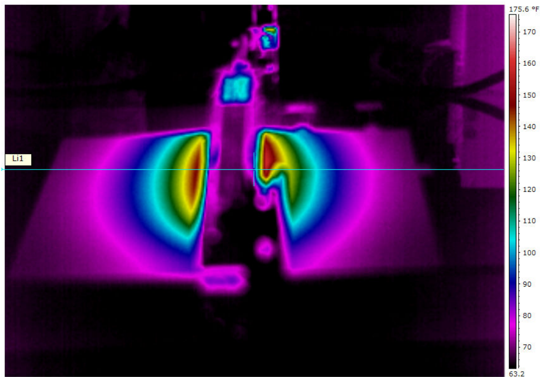
Figure 52: Specimen II Infrared Image II
