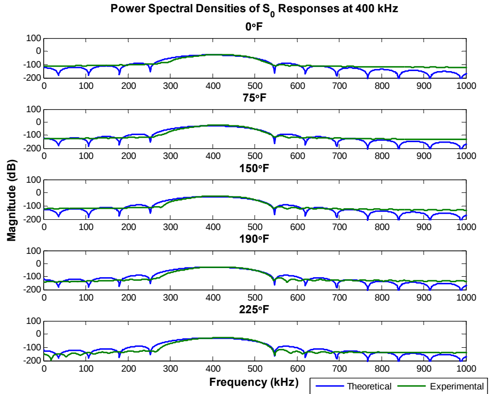
Figure 82: Power Spectral Densities of S_0 Responses at 400 kHz
