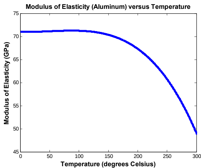
Figure 1: Modulus versus Temperature (2; 9; 10)
