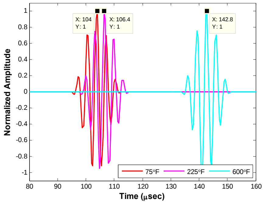
Figure 117: Theoretical Thermal Gradient S_0 Responses over 500 mm
