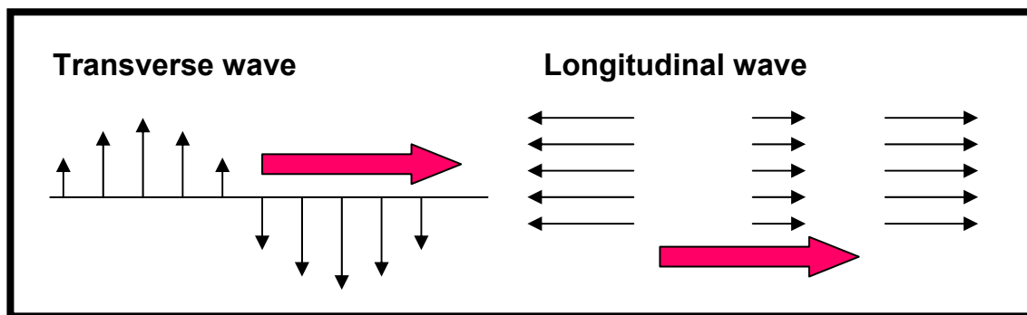
Figure 5: Transverse and Longitudinal Waves (11)
