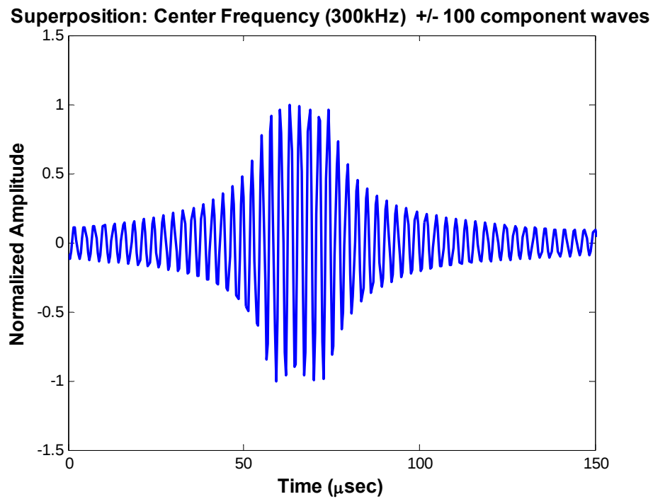
Figure 10: Superposition of 200 Component Waves
