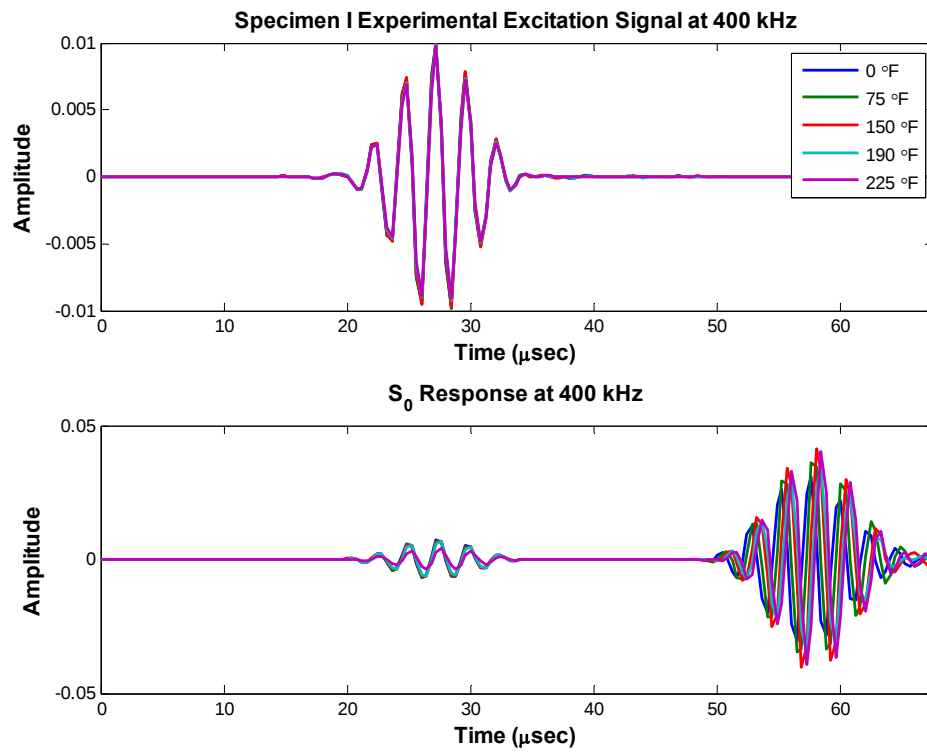
Figure 104: Specimen I Raw Signals at 400 kHz
