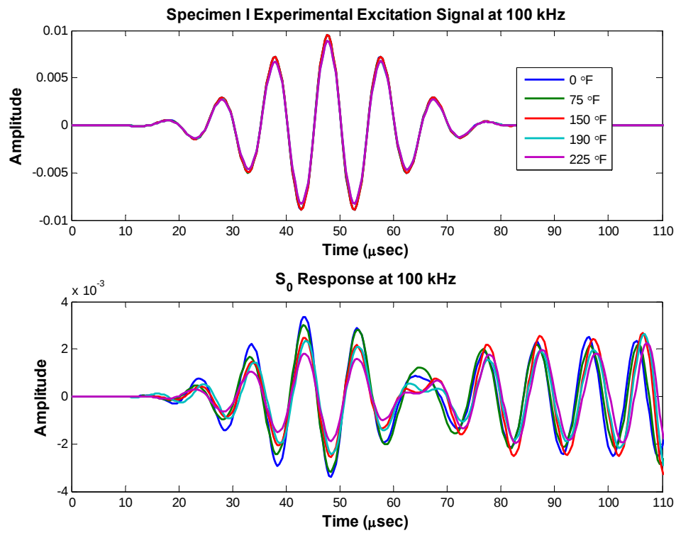
Figure 94: Specimen I Raw Signals at 100 kHz
