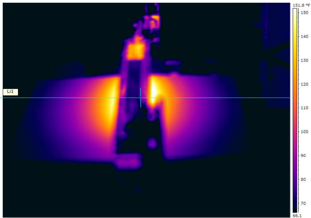
Figure 51: Specimen II Infrared Image I
