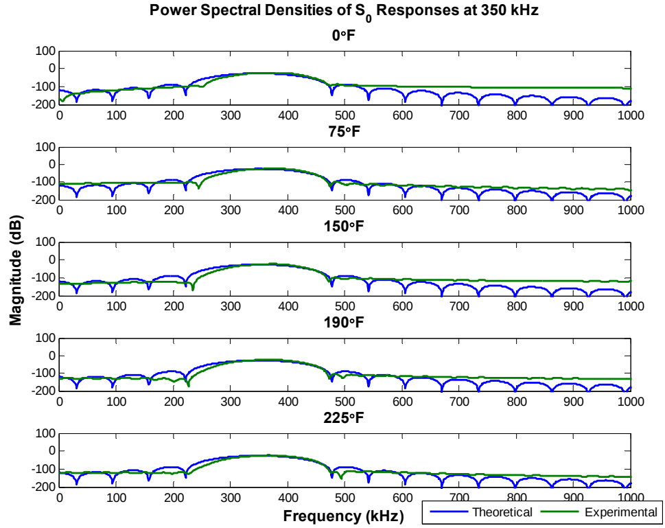
Figure 81: Power Spectral Densities of S_0 Responses at 350 kHz
