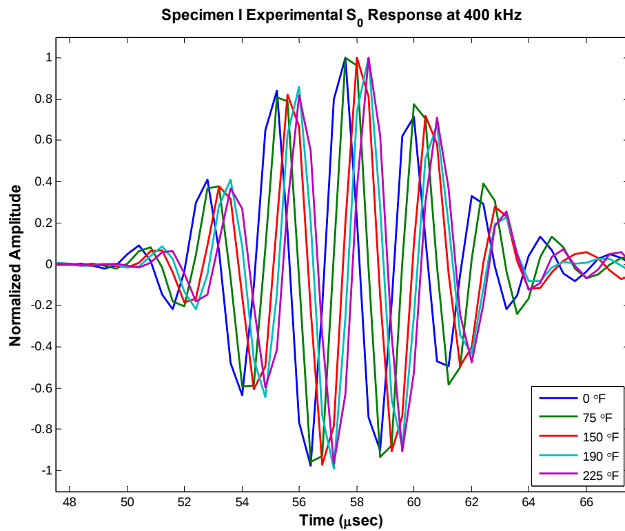
Figure 105: Specimen I Experimental S_0 Response at 400 kHz
