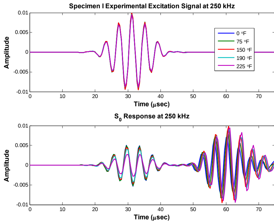
Figure 100: Specimen I Raw Signals at 250 kHz
