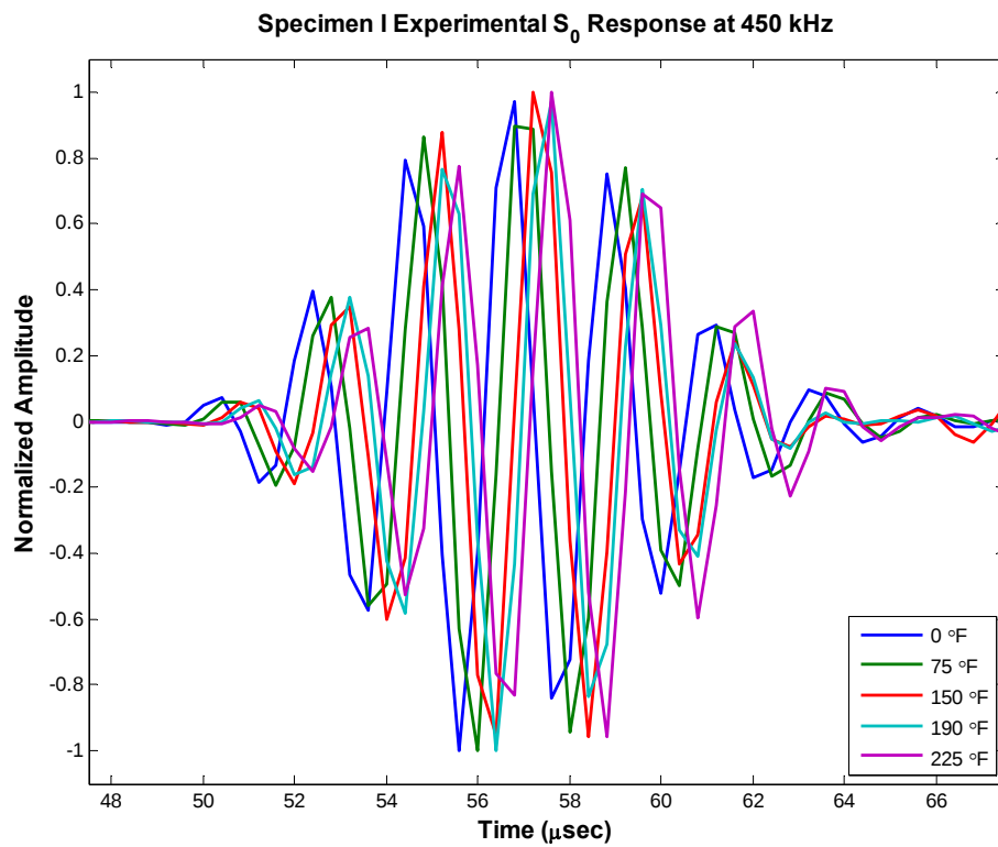
Figure 107: Specimen I Experimental S_0 Response at 450 kHz
