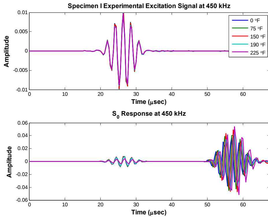
Figure 106: Specimen I Raw Signals at 450 kHz
