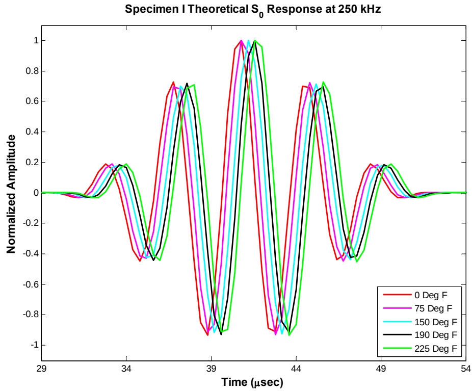
Figure 87: Specimen I Theoretical S_0 Response at 250 kHz
