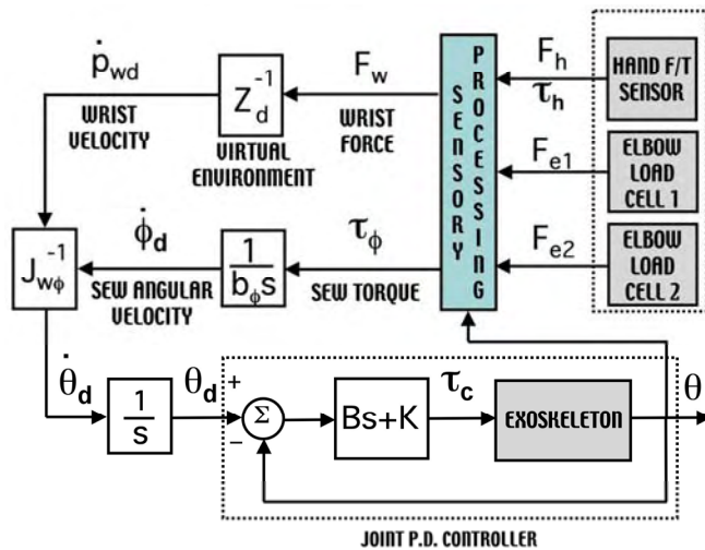
Figure 3 Admittance controller.
