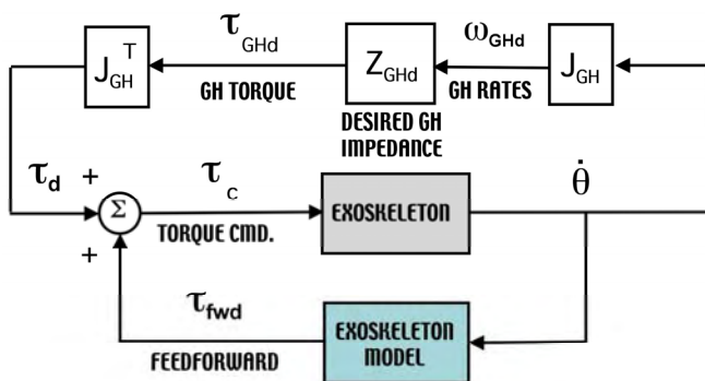
Figure 4 Impedance controller.
