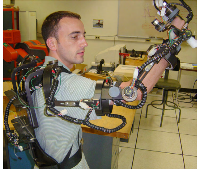
Fig. 2. SSL personnel dons the MB Exoskeleton during visit to Wright-Patterson Air Force Base. (SSL Photo Archives – used with permission of the Wright-Patterson Air Force Research Laboratory)
