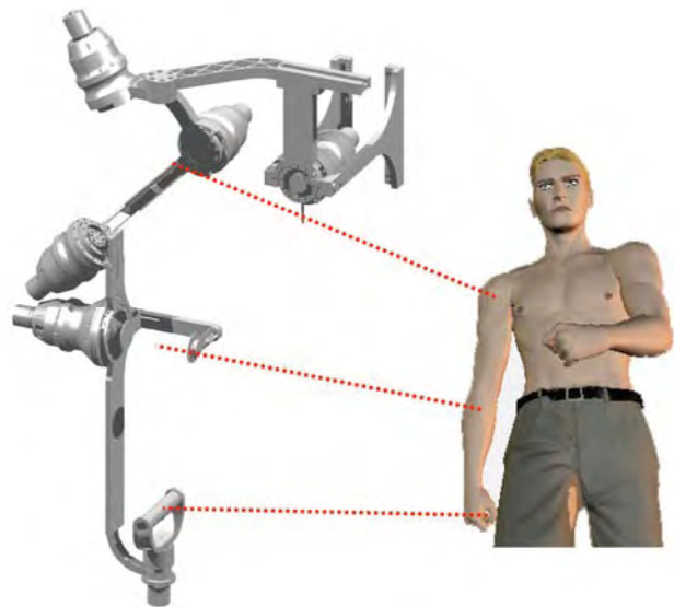
Figure 1 The MGA Exoskeleton designed for shoulder therapy.
