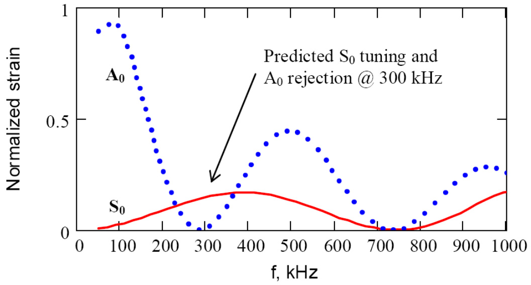
Figure 1.9 Theoretical Lamb wave response of a 1.6 mm aluminum plate [4]
